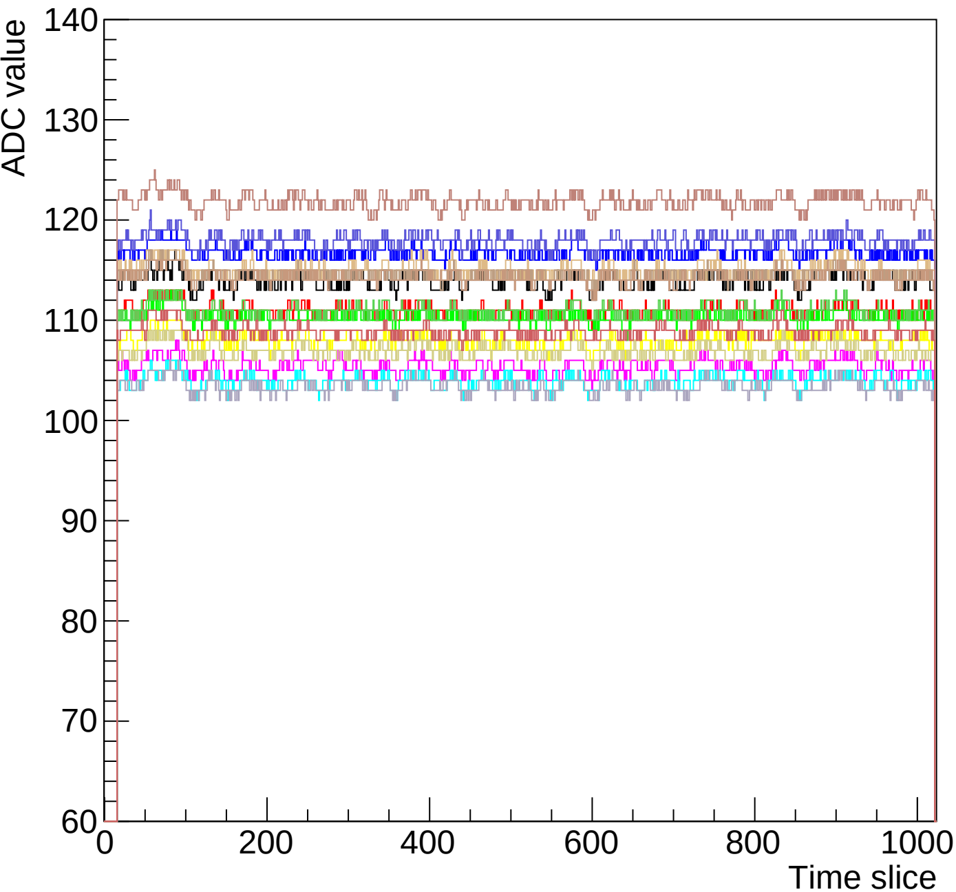
Run 0 event 20 mcm 0 chip 2 lvcard-fec0-debug
