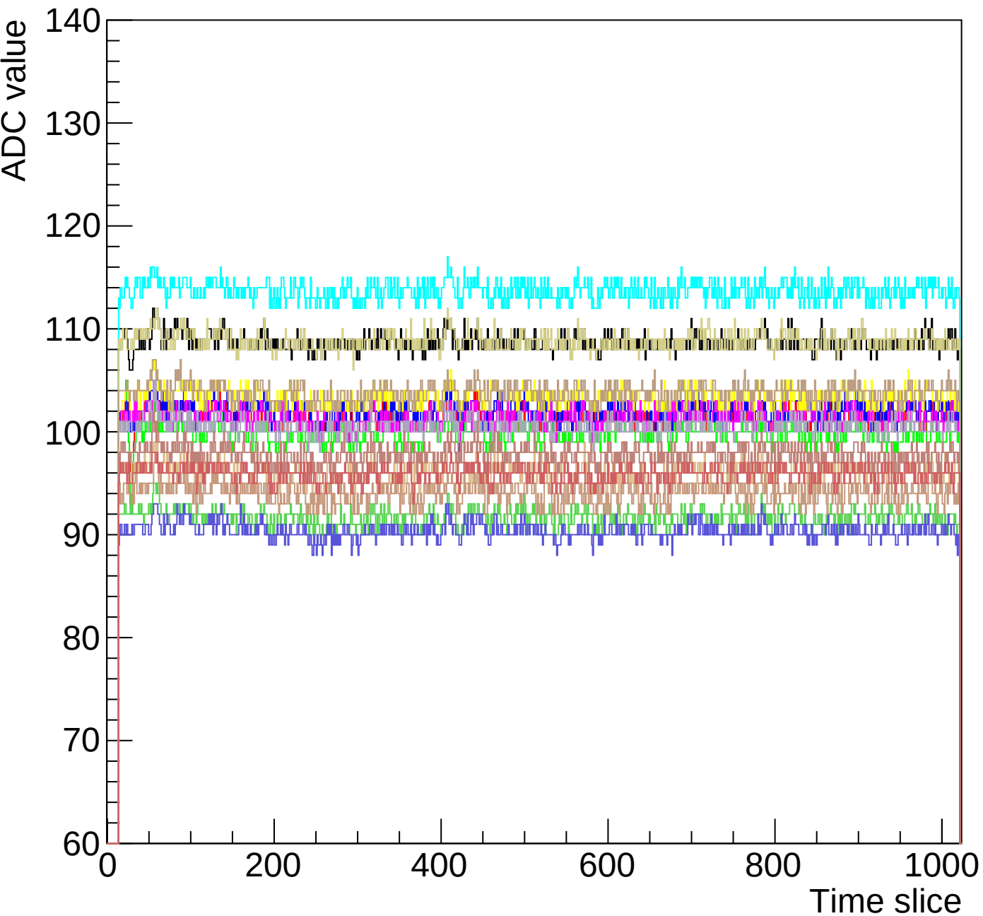
Run 0 event 20 mcm 1 chip 0 chamber-fec01-debug1
