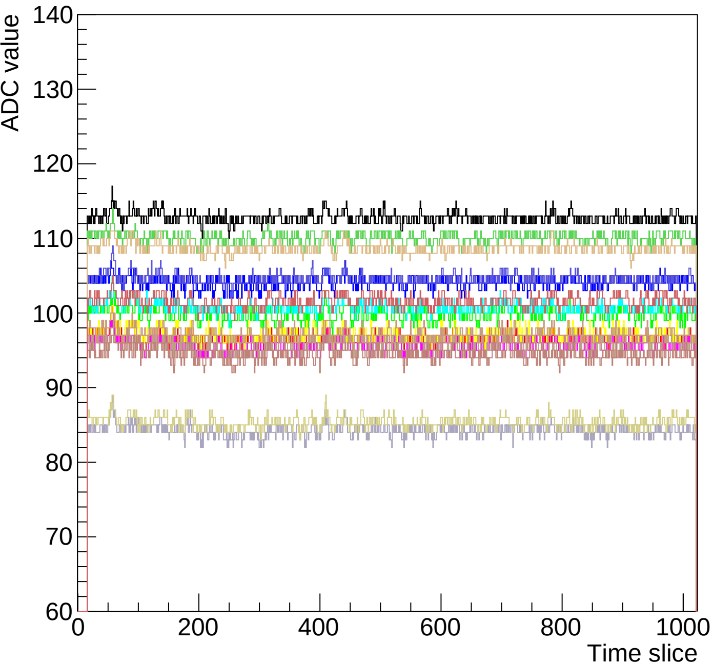
Run 0 event 20 mcm 1 chip 2 chamber-fec01-debug1
