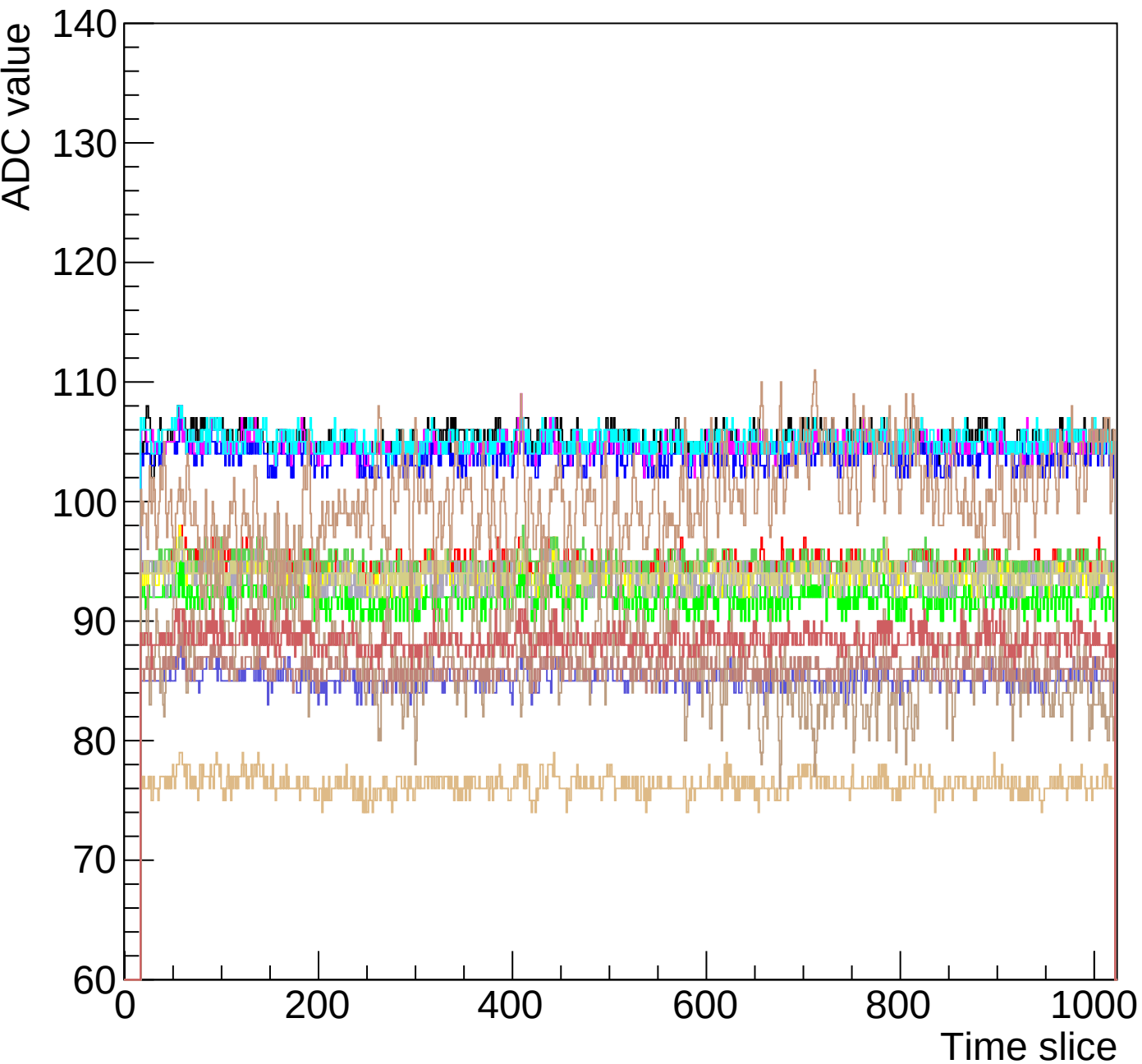
Run 0 event 20 mcm 1 chip 3 chamber-fec01-debug1
