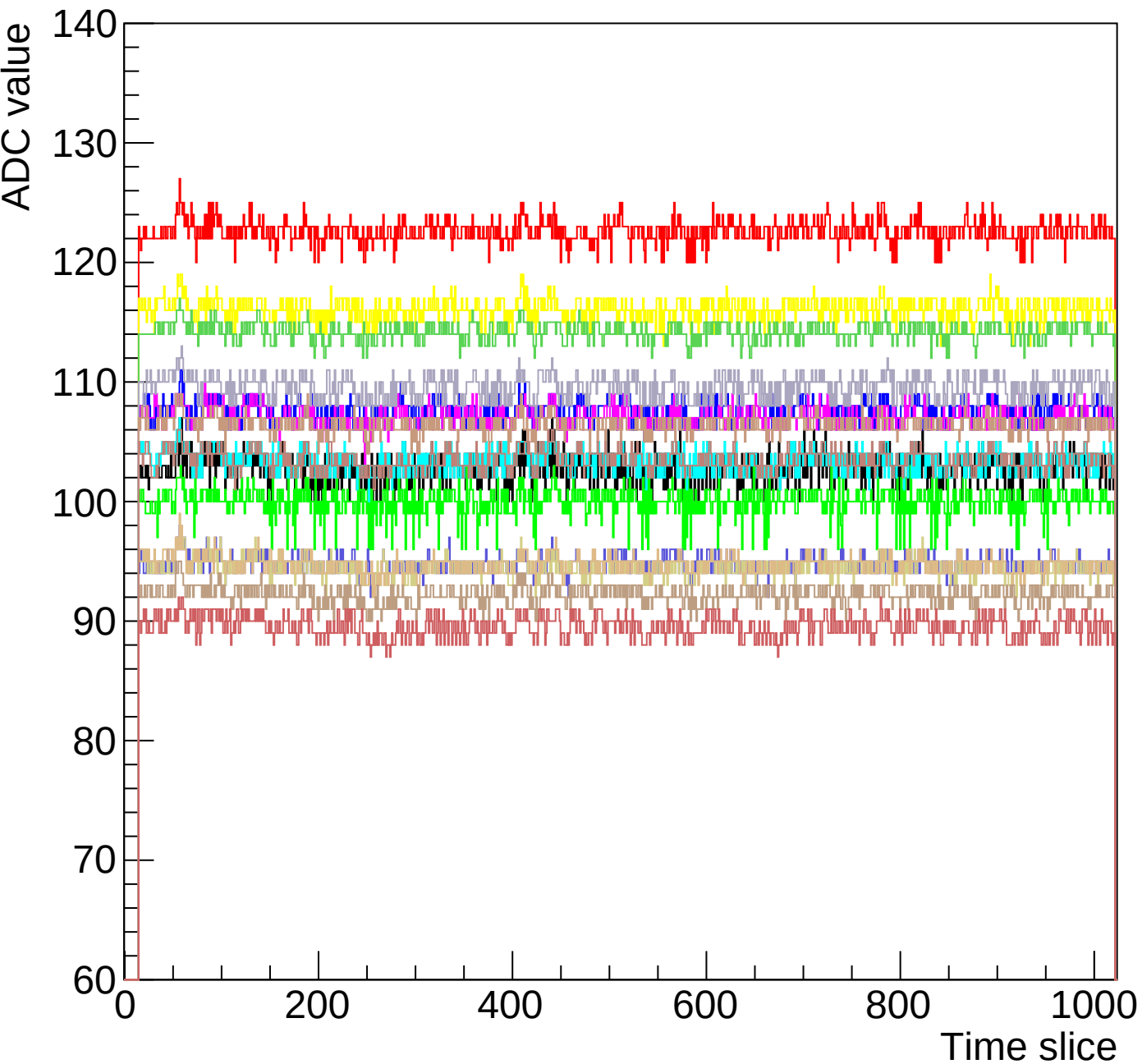
Run 0 event 20 mcm 1 chip 1 chamber-fec01-debug1
