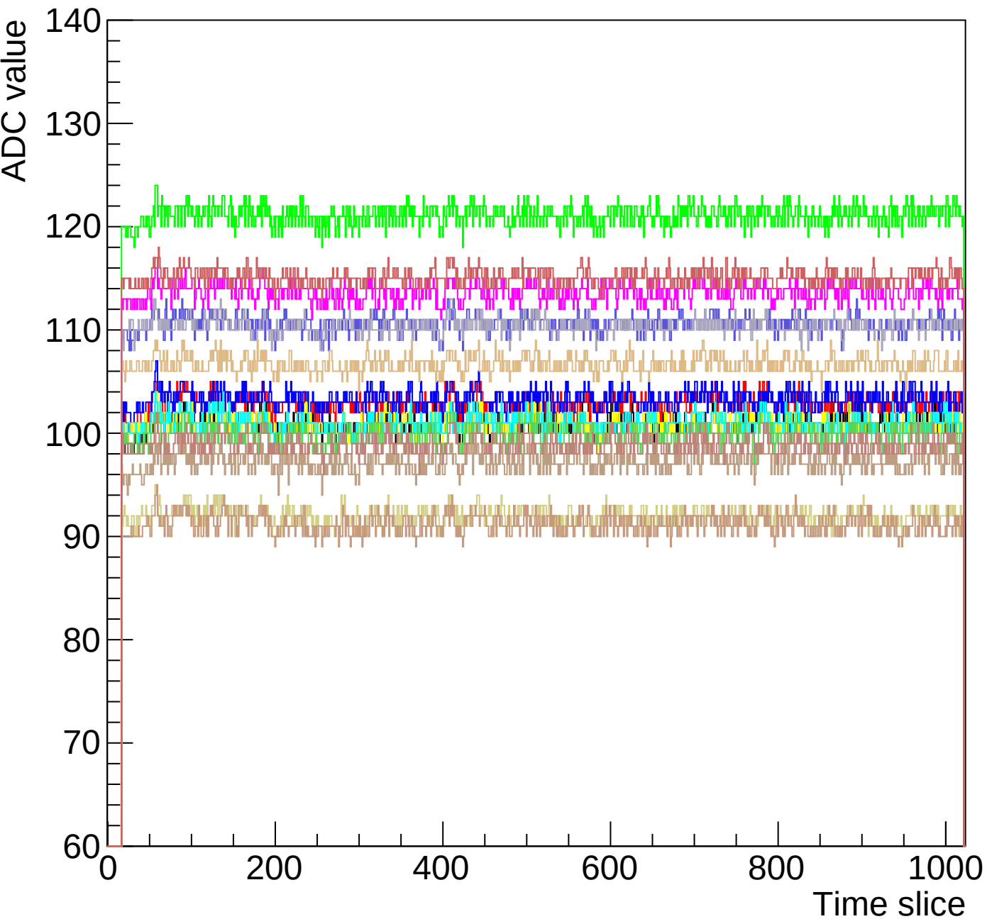
Run 0 event 20 mcm 1 chip 7 chamber-fec01-debug1
