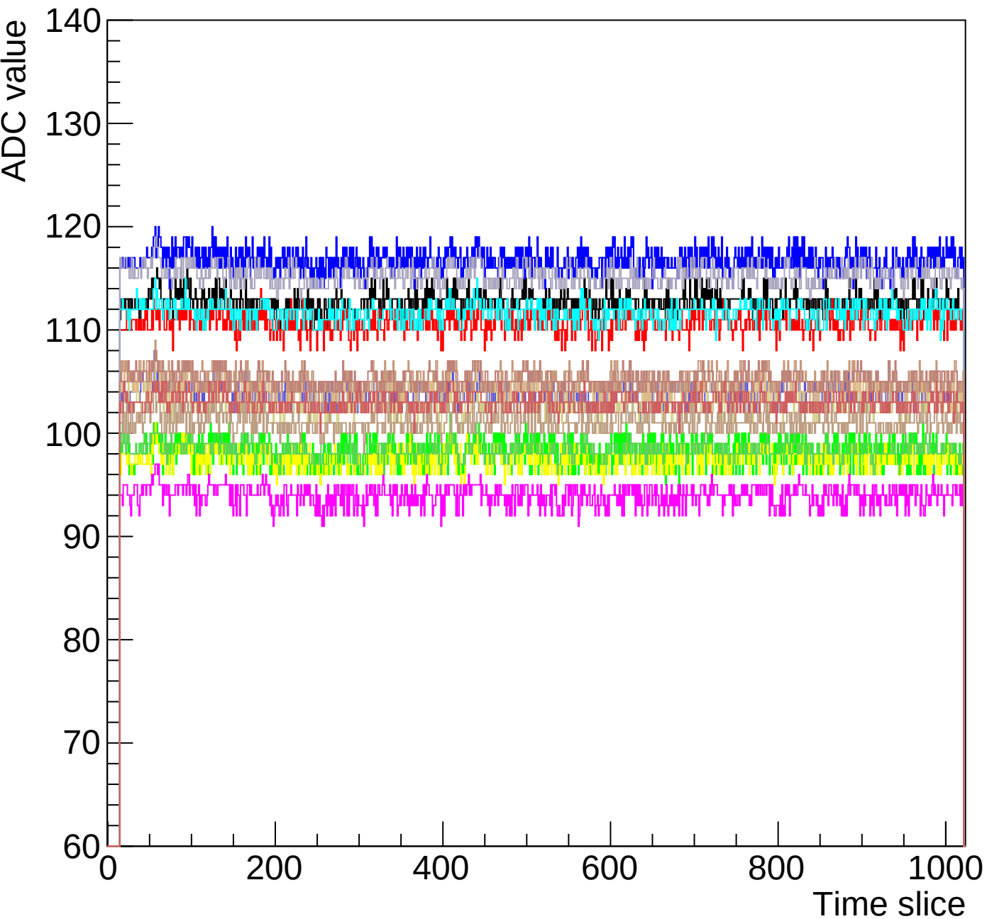
Run 0 event 20 mcm 1 chip 5 chamber-fec01-debug1
