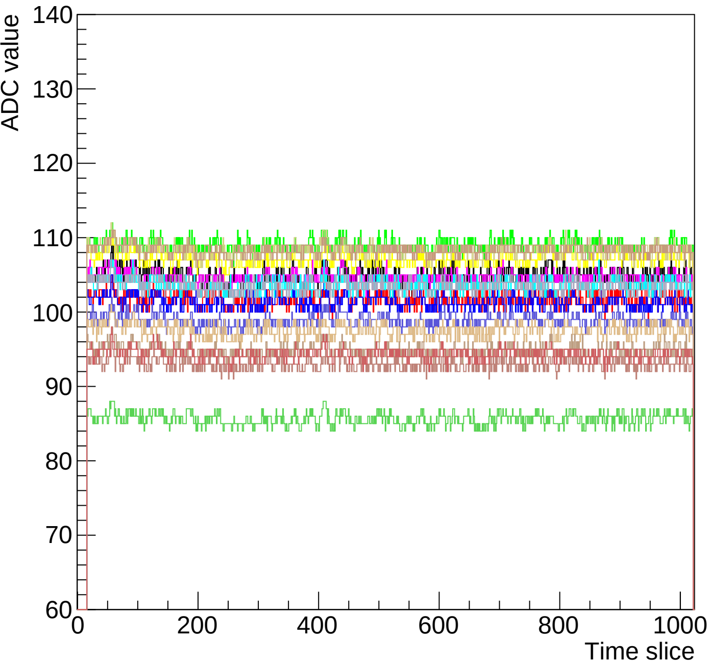
Run 0 event 20 mcm 1 chip 6 chamber-fec01-debug1
