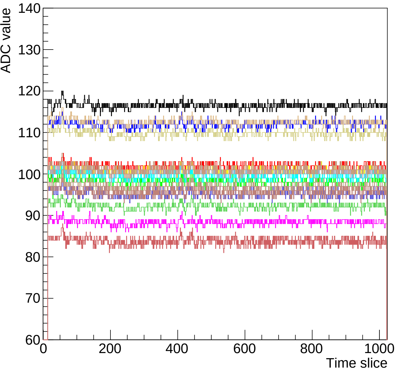
Run 0 event 20 mcm 1 chip 4 chamber-fec01-debug1
