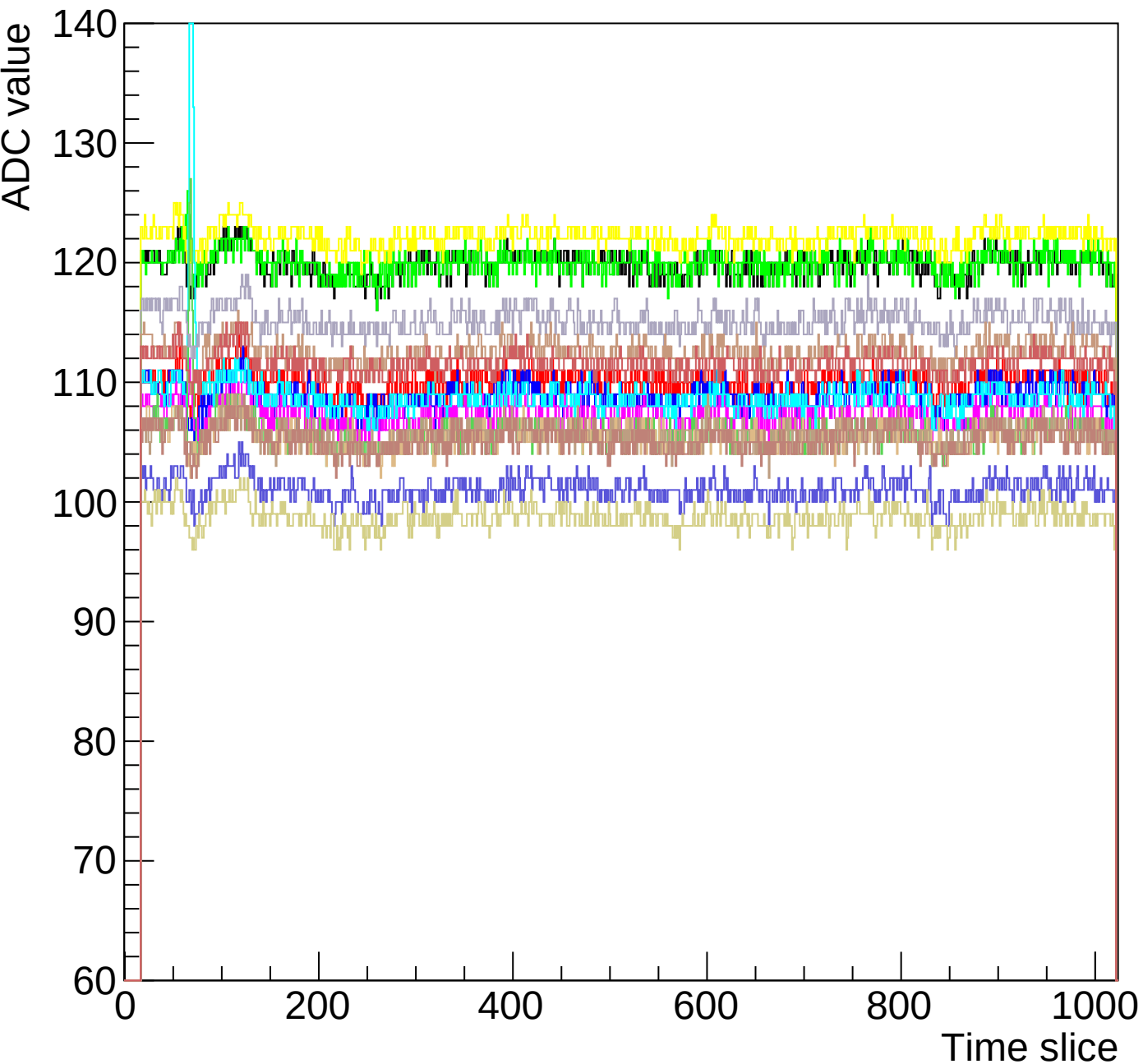
Run 0 event 7 mcm 1 chip 7 chamber-fec01-debug
