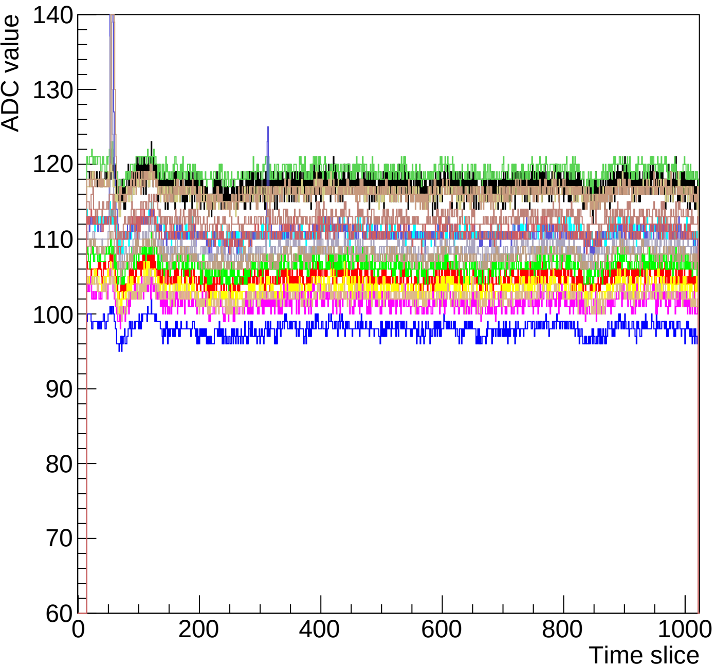
Run 0 event 7 mcm 1 chip 1 chamber-fec01-debug
