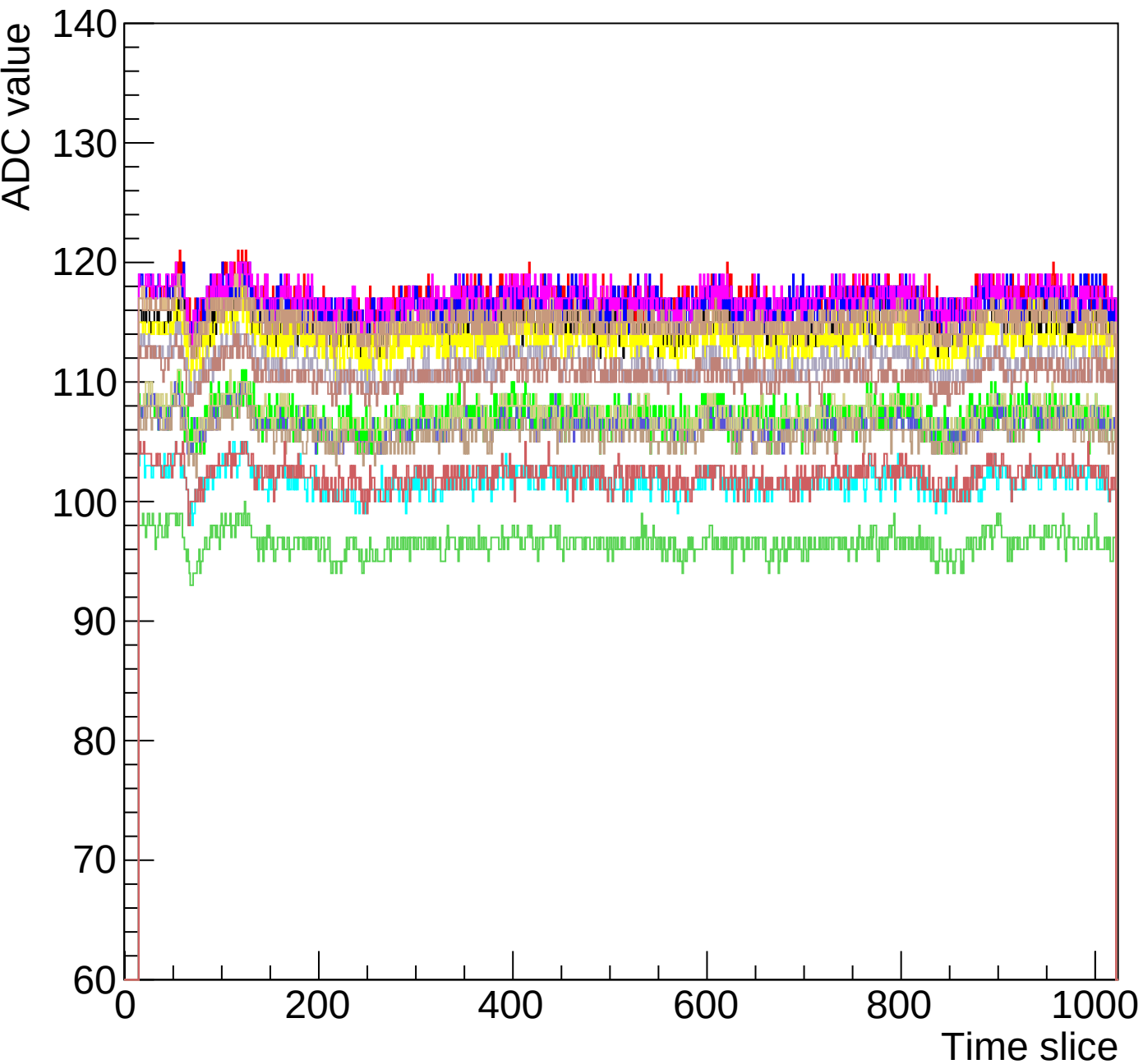
Run 0 event 7 mcm 1 chip 5 chamber-fec01-debug
