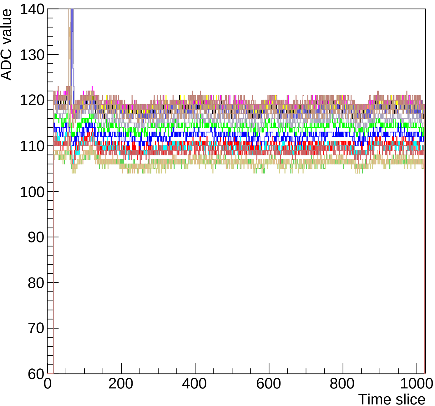
Run 0 event 7 mcm 1 chip 6 chamber-fec01-debug
