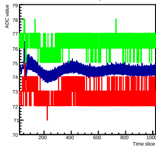
Norm mcm 1 chip 3 chan 4
