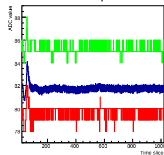
Norm mcm 0 chip 3 chan 10
