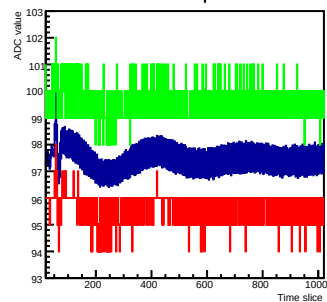
Norm mcm 1 chip 0 chan 15
