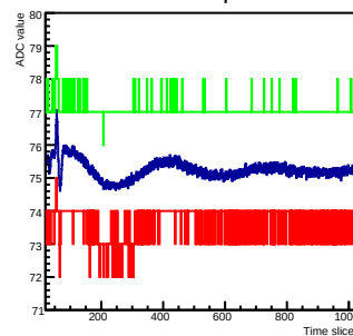
Norm mcm 1 chip 2 chan 2
