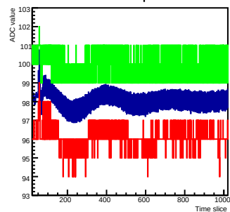
Norm mcm 1 chip 0 chan 11
