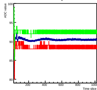
Norm mcm 1 chip 0 chan 2
