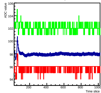
Norm mcm 0 chip 2 chan 3
