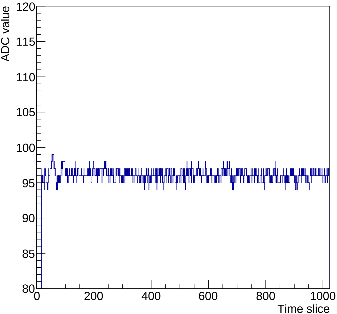
Run 1 event 20 mcm 0 chip 3 channel 12 full
