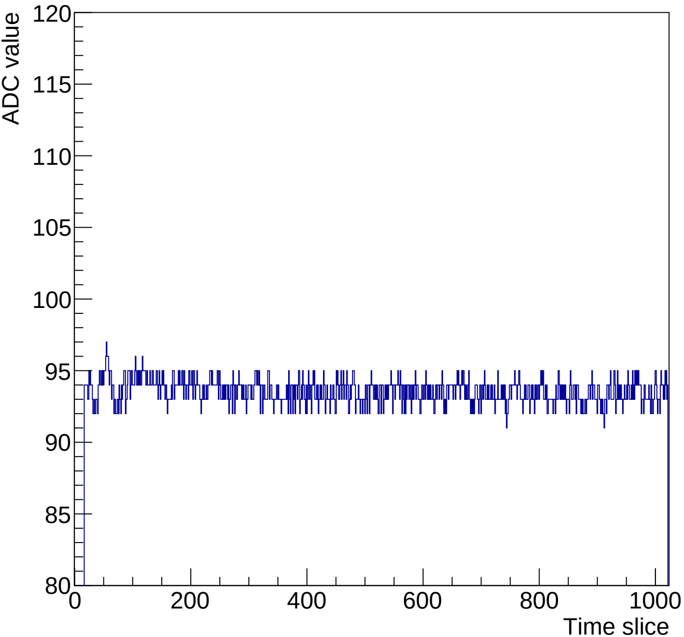
Run 1 event 20 mcm 0 chip 3 channel 14 full
