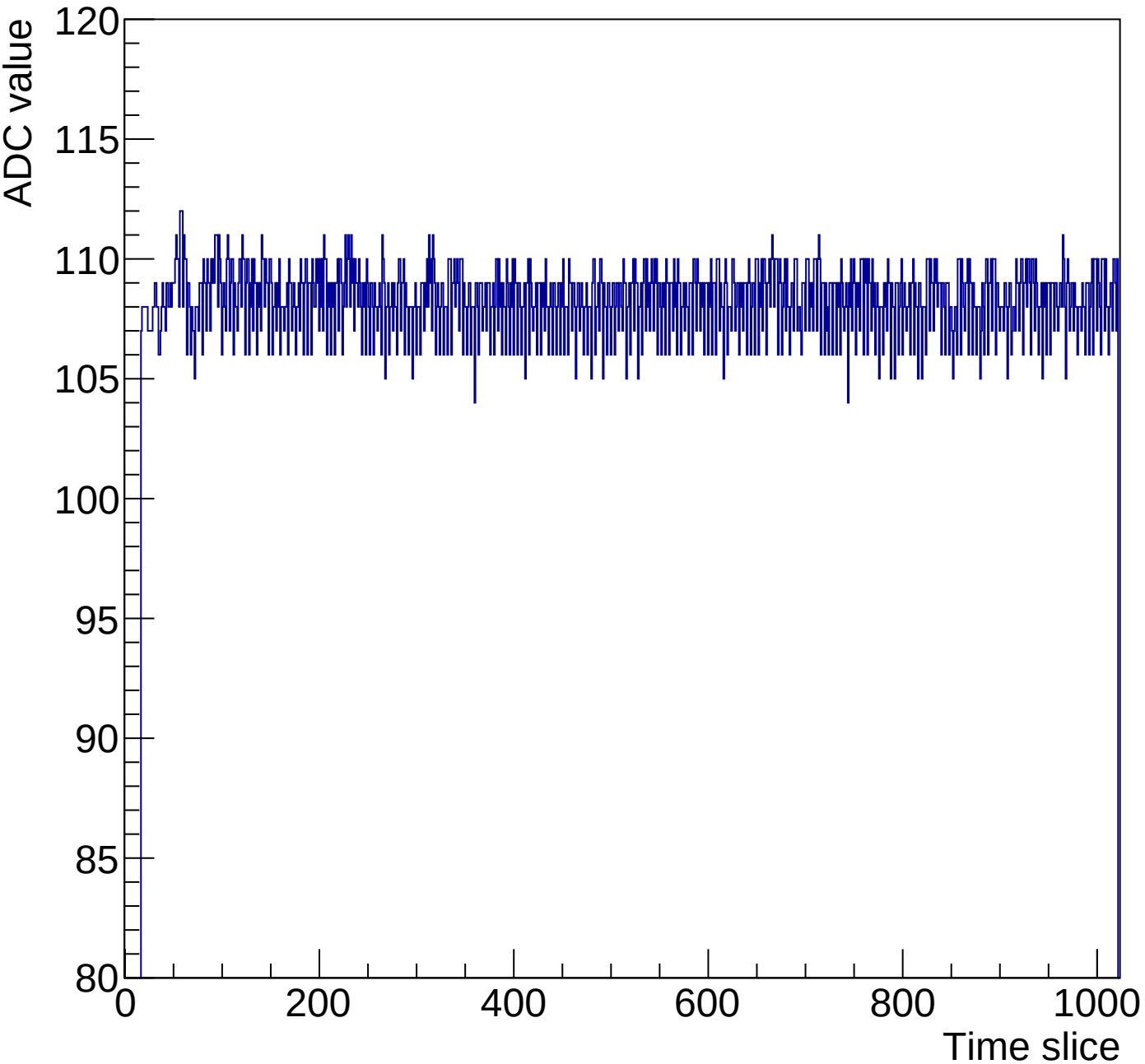
Run 1 event 20 mcm 0 chip 3 channel 2 full
