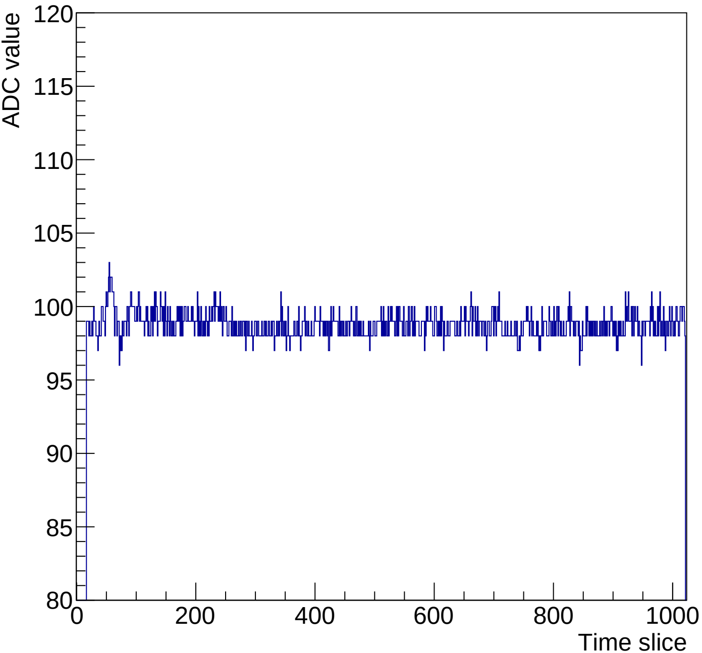
Run 1 event 20 mcm 0 chip 3 channel 10 full
