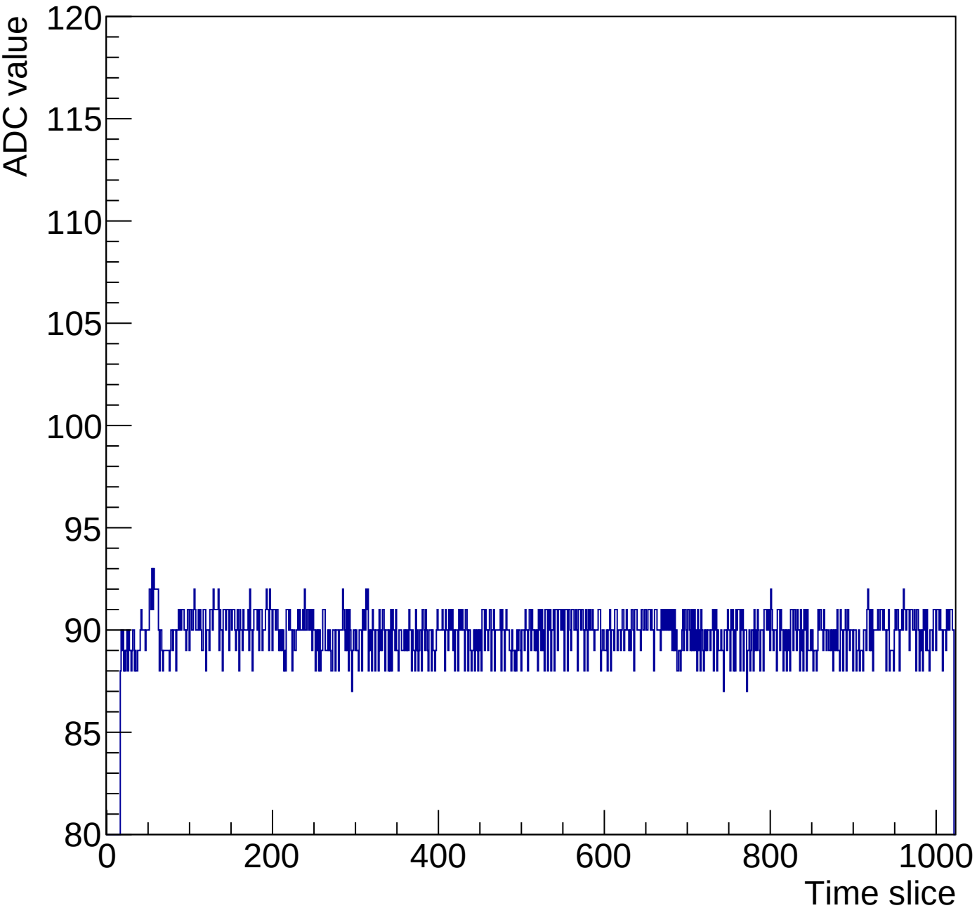
Run 1 event 20 mcm 0 chip 3 channel 4 full
