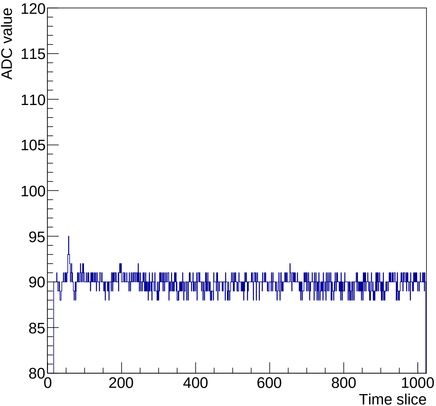
Run 1 event 20 mcm 0 chip 3 channel 9 full
