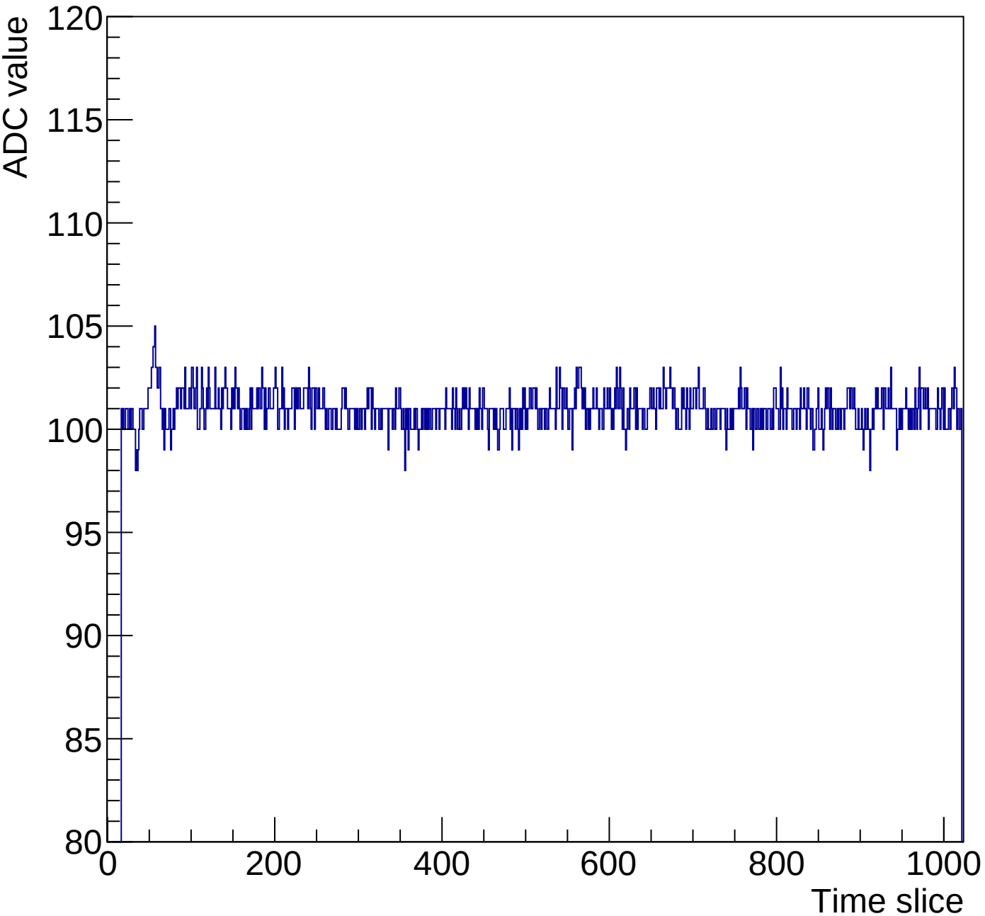
Run 1 event 20 mcm 0 chip 3 channel 8 full
