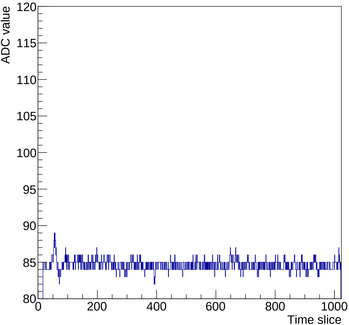
Run 1 event 20 mcm 0 chip 3 channel 7 full
