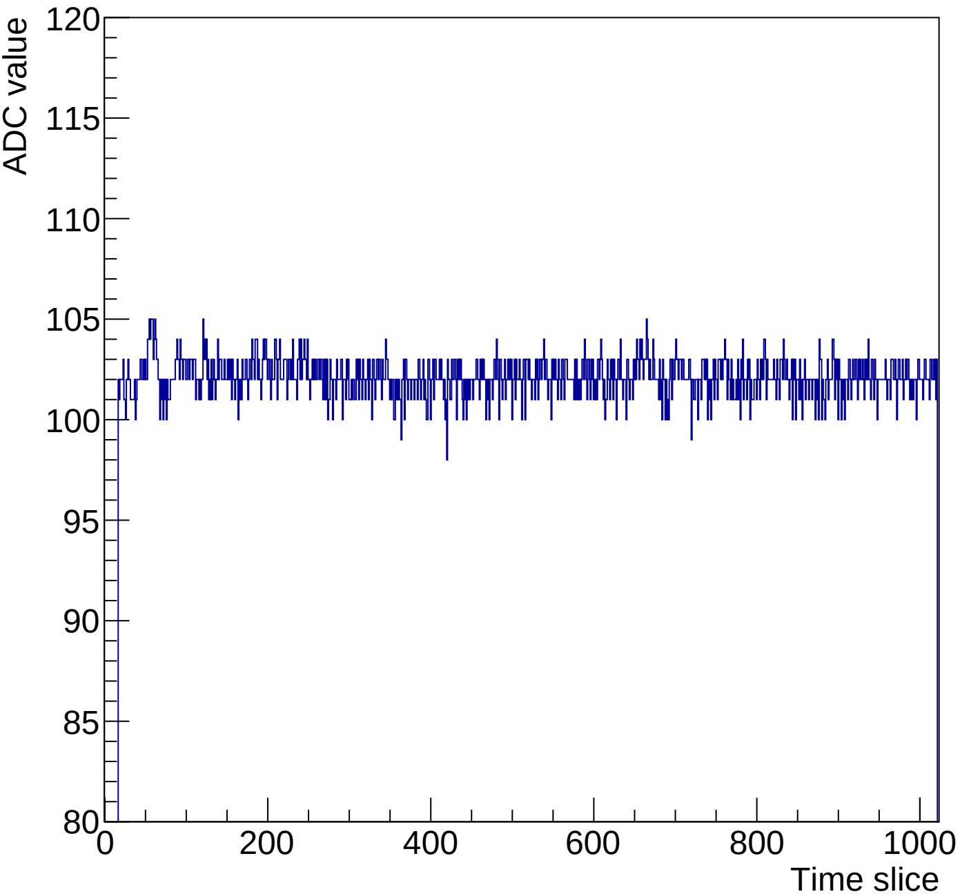
Run 1 event 20 mcm 0 chip 3 channel 5 full
