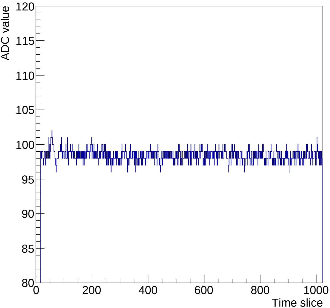
Run 1 event 20 mcm 0 chip 3 channel 11 full
