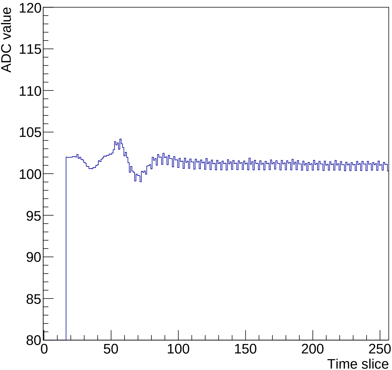
Run 1 Time mcm 0 chip 3 chan 10 256-90ns
