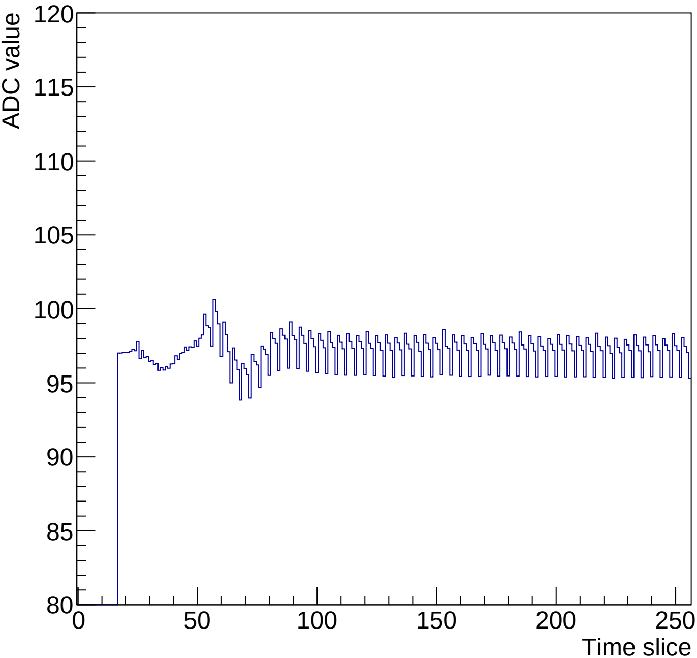
Run 1 Time mcm 0 chip 3 chan 3 256-90ns
