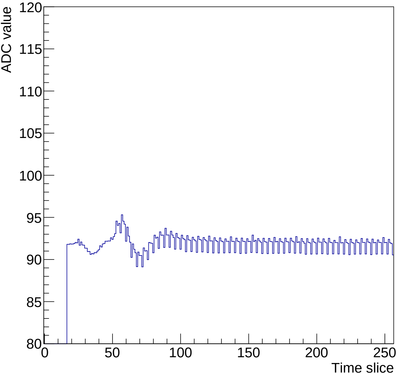
Run 1 Time mcm 0 chip 3 chan 4 256-90ns
