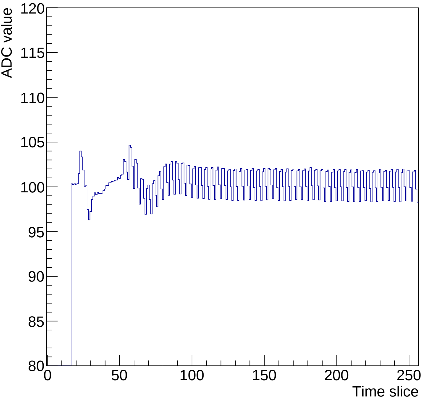
Run 1 Time mcm 0 chip 3 chan 0 256-90ns
