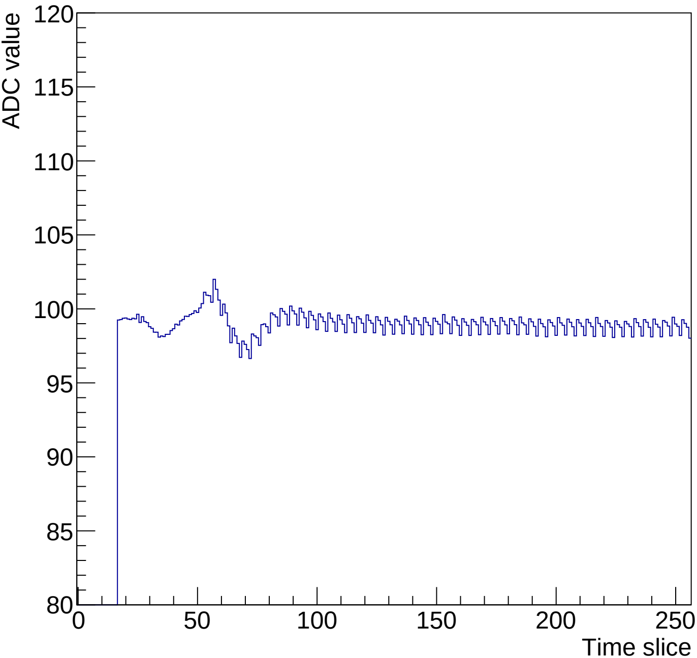
Run 1 Time mcm 0 chip 3 chan 12 256-90ns
