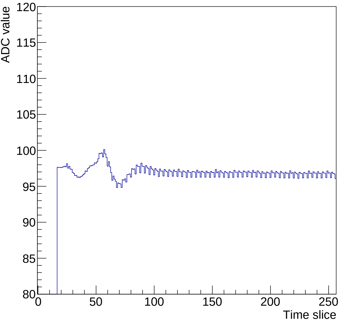
Run 1 Time mcm 0 chip 3 chan 14 256-90ns
