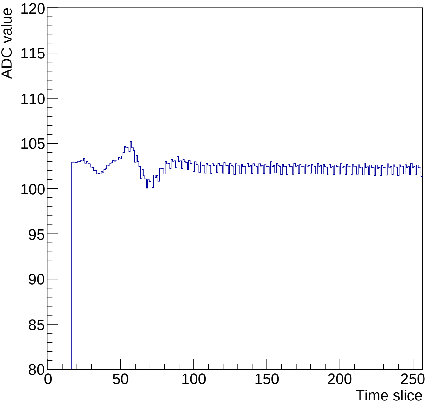
Run 1 Time mcm 0 chip 3 chan 11 256-90ns
