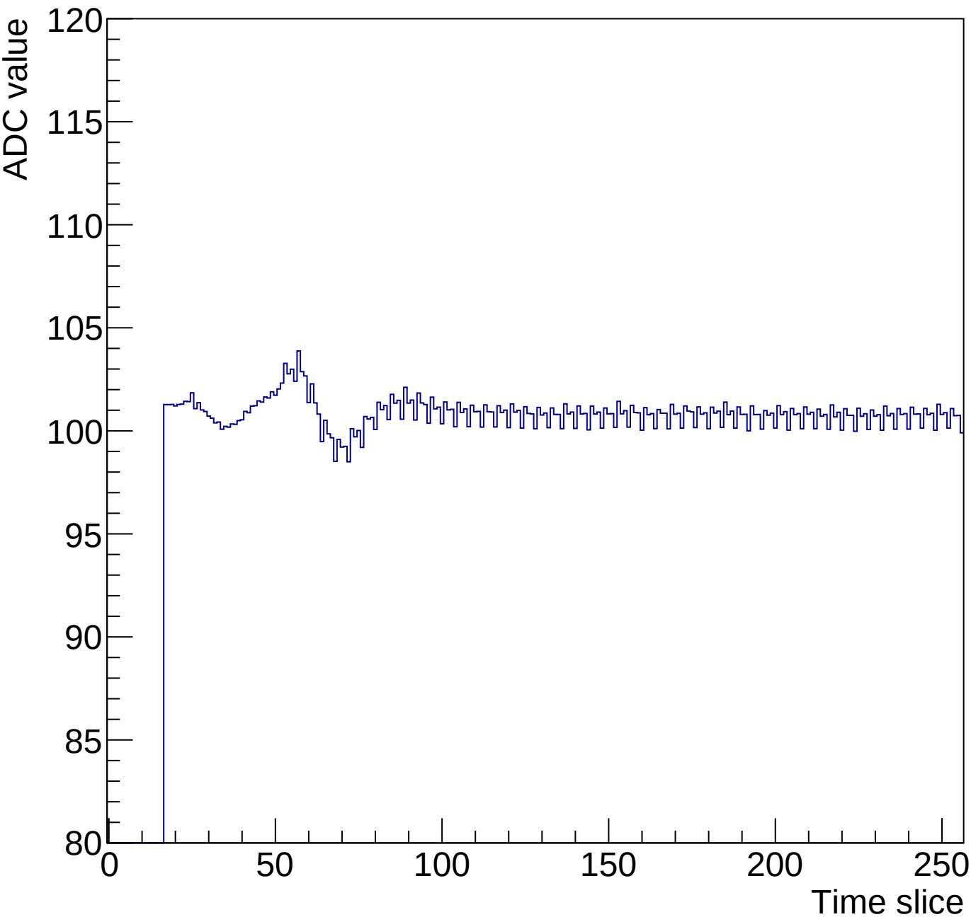
Run 1 Time mcm 0 chip 3 chan 6 256-90ns
