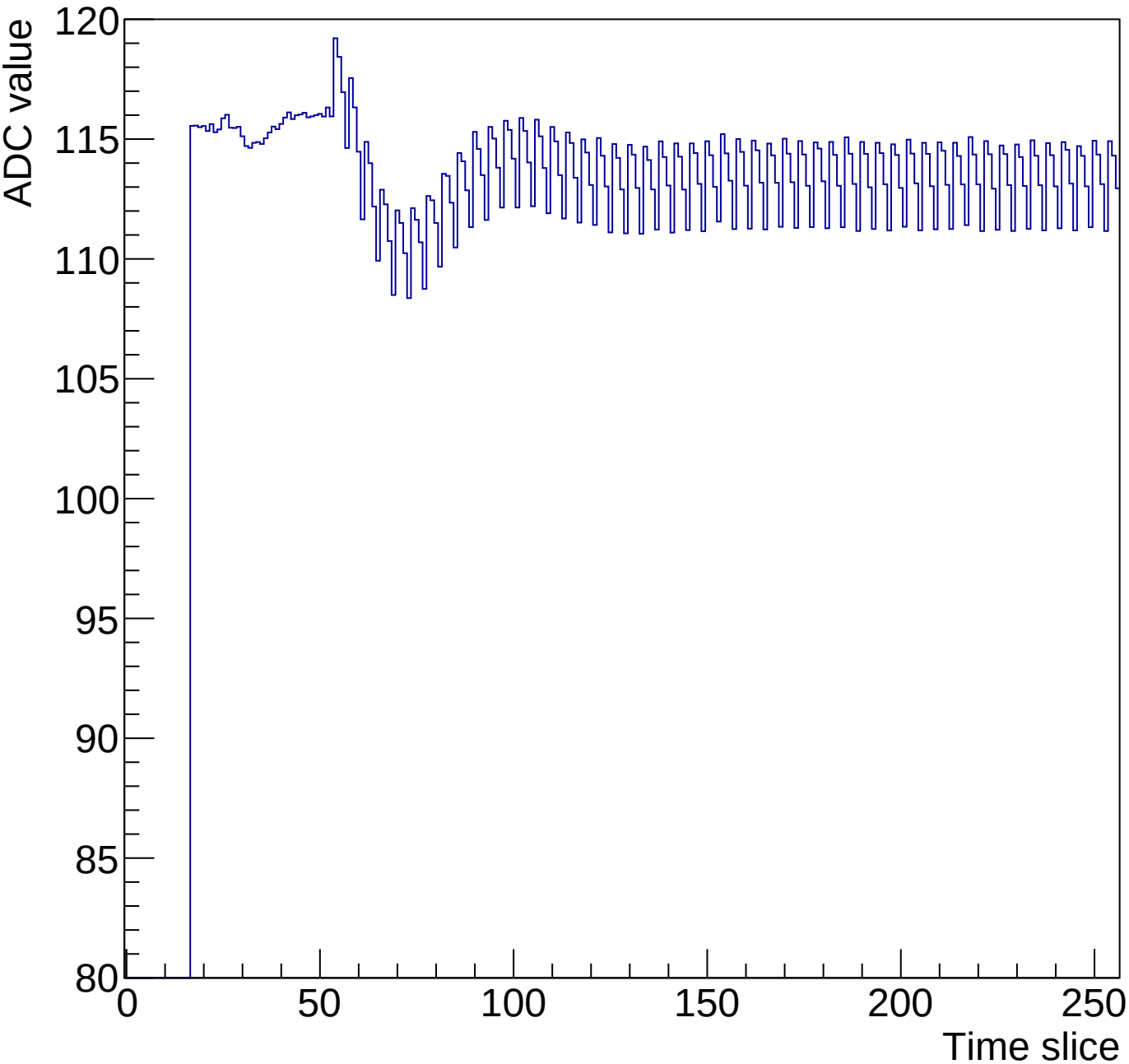
Run 3 Time mcm 0 chip 3 chan 15 256-30ns
