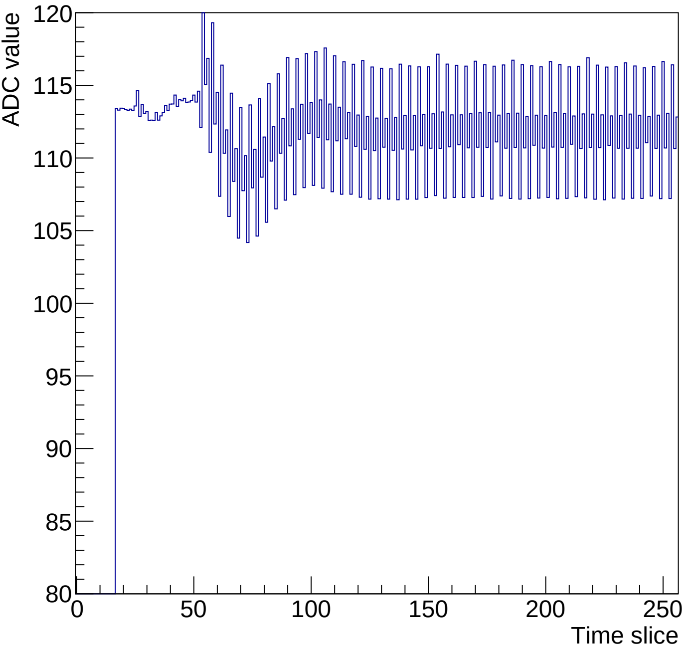
Run 3 Time mcm 0 chip 3 chan 13 256-30ns
