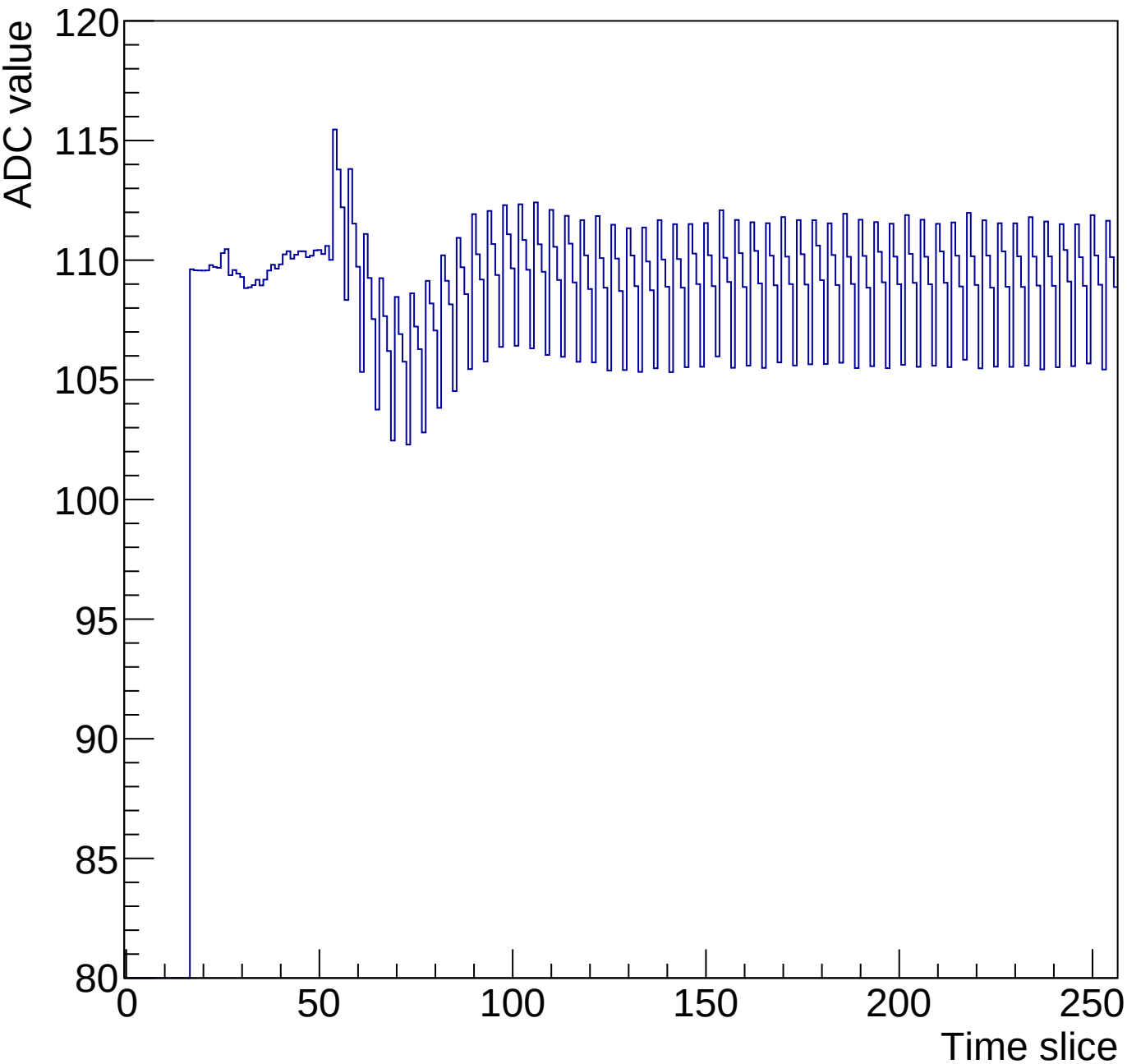
Run 3 Time mcm 0 chip 3 chan 8 256-30ns
