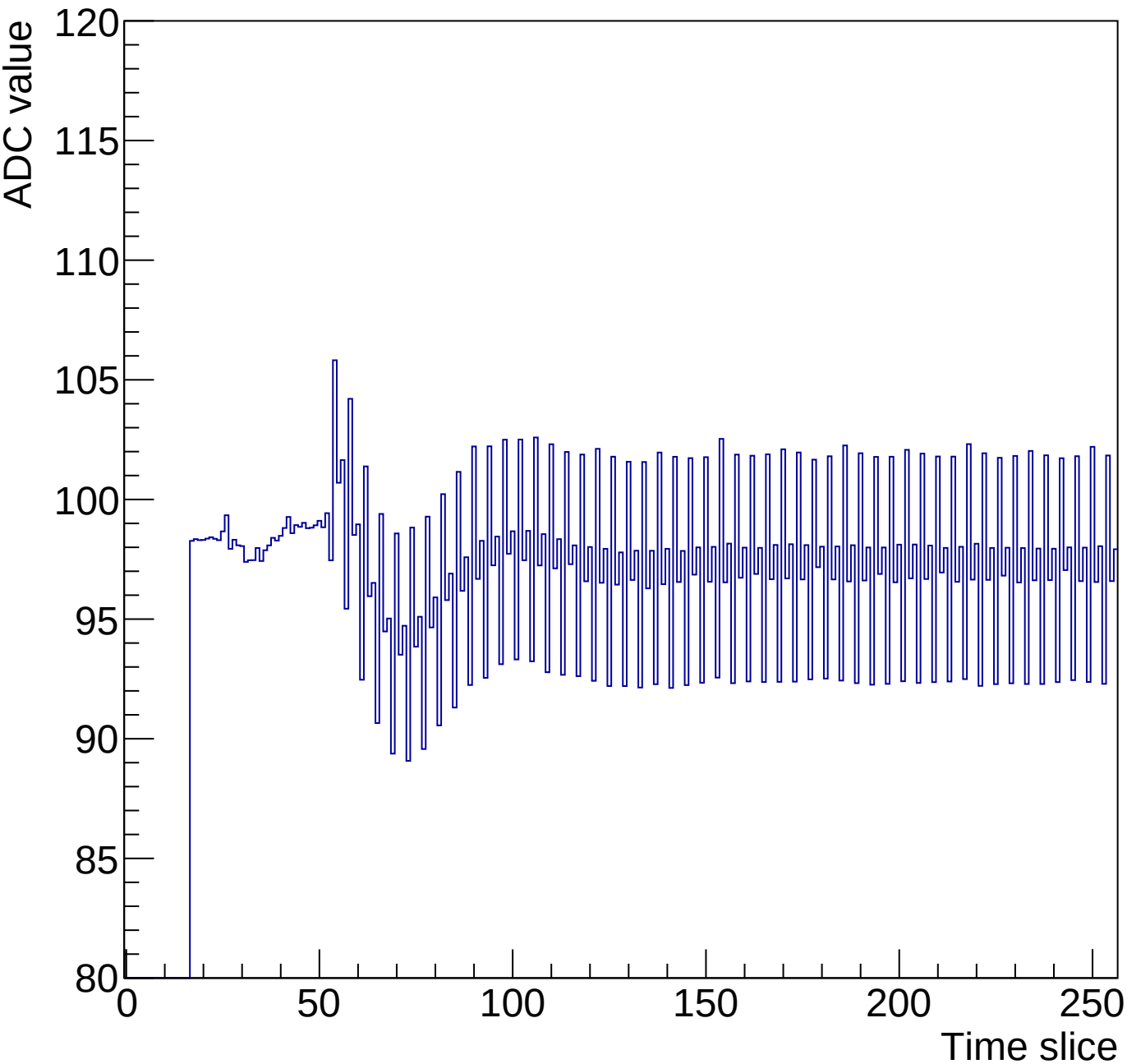
Run 3 Time mcm 0 chip 3 chan 9 256-30ns
