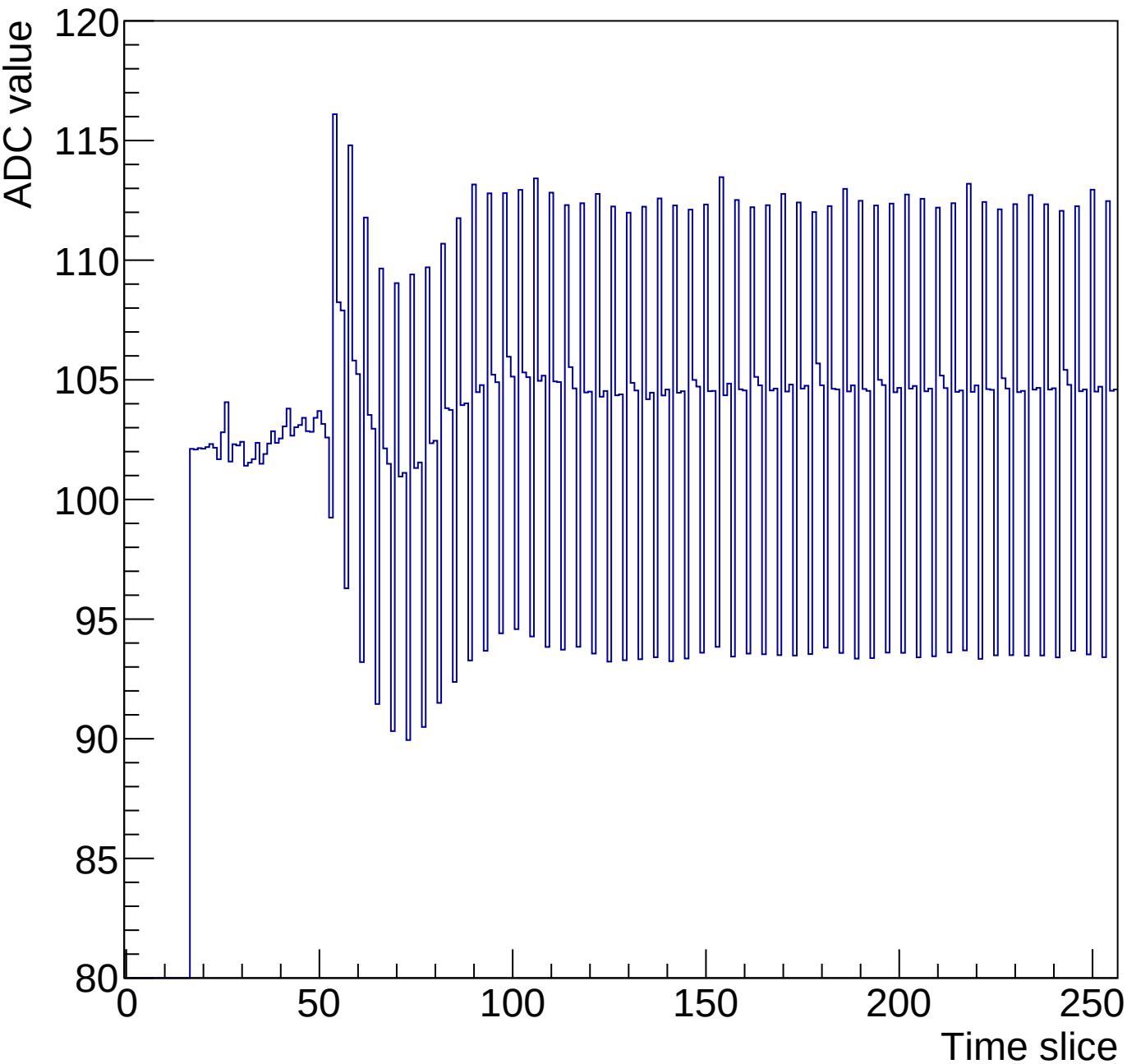
Run 3 Time mcm 0 chip 3 chan 3 256-30ns
