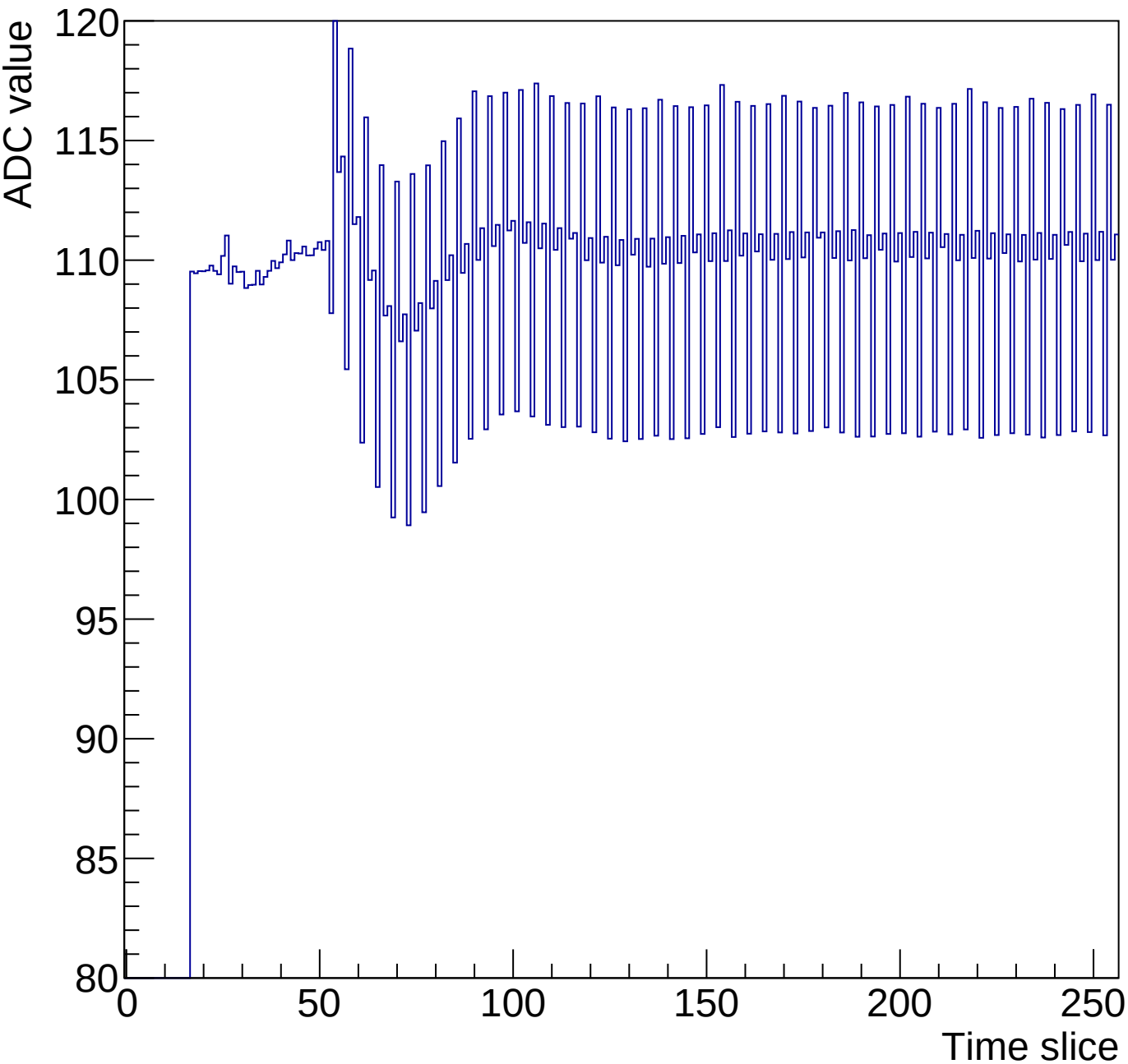
Run 3 Time mcm 0 chip 3 chan 5 256-30ns
