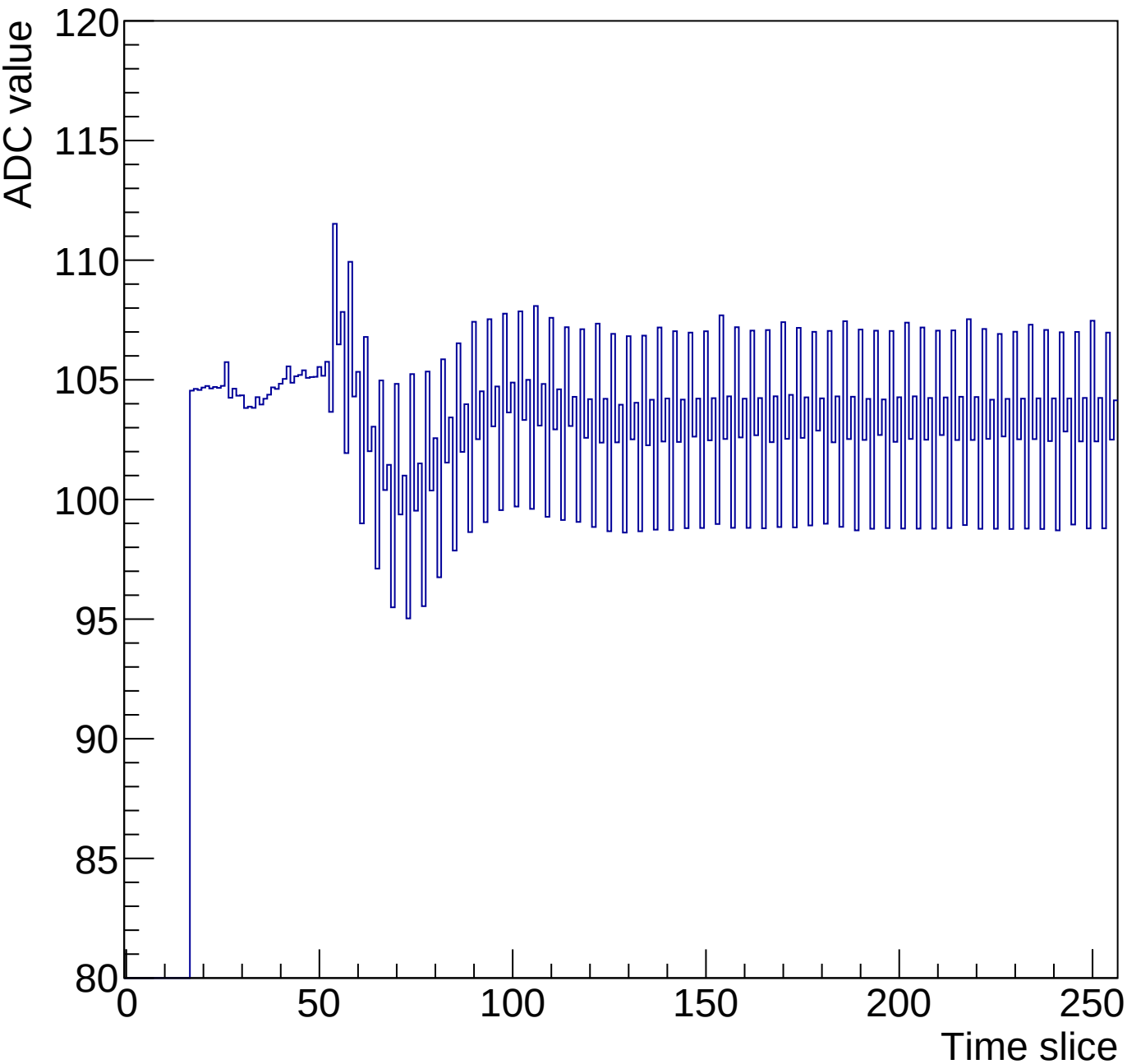
Run 3 Time mcm 0 chip 3 chan 10 256-30ns
