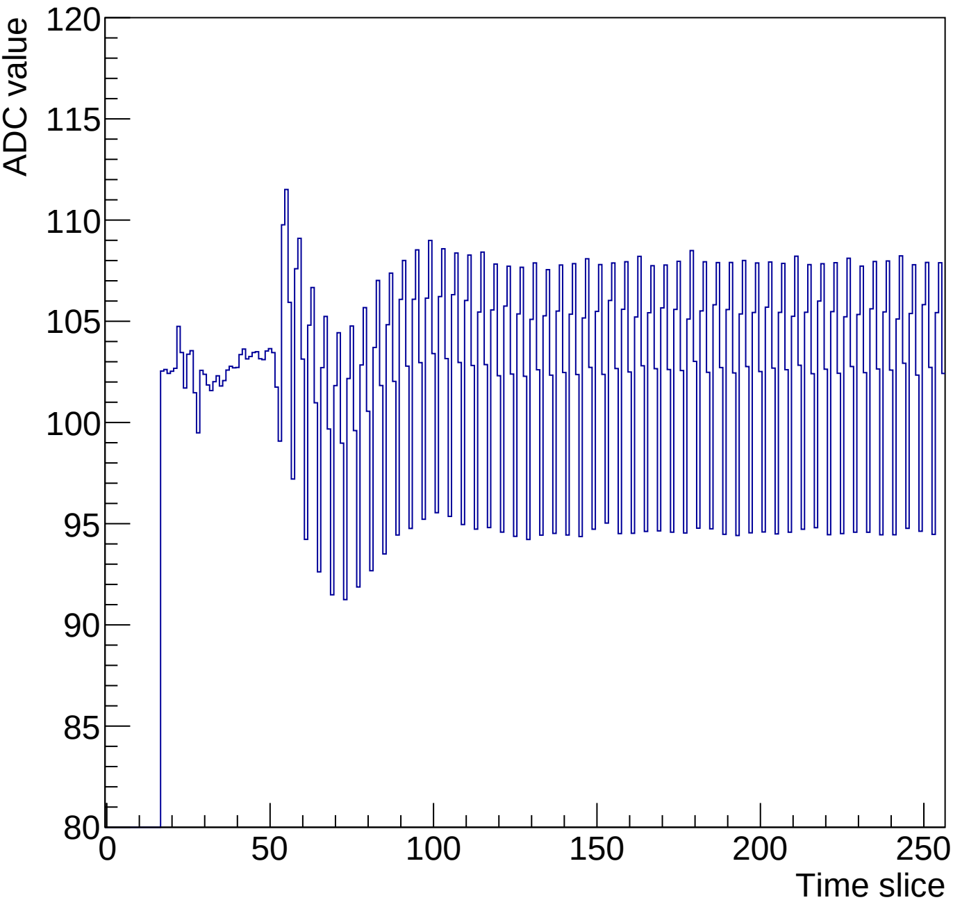
Run 3 Time mcm 0 chip 3 chan 0 256-30ns
