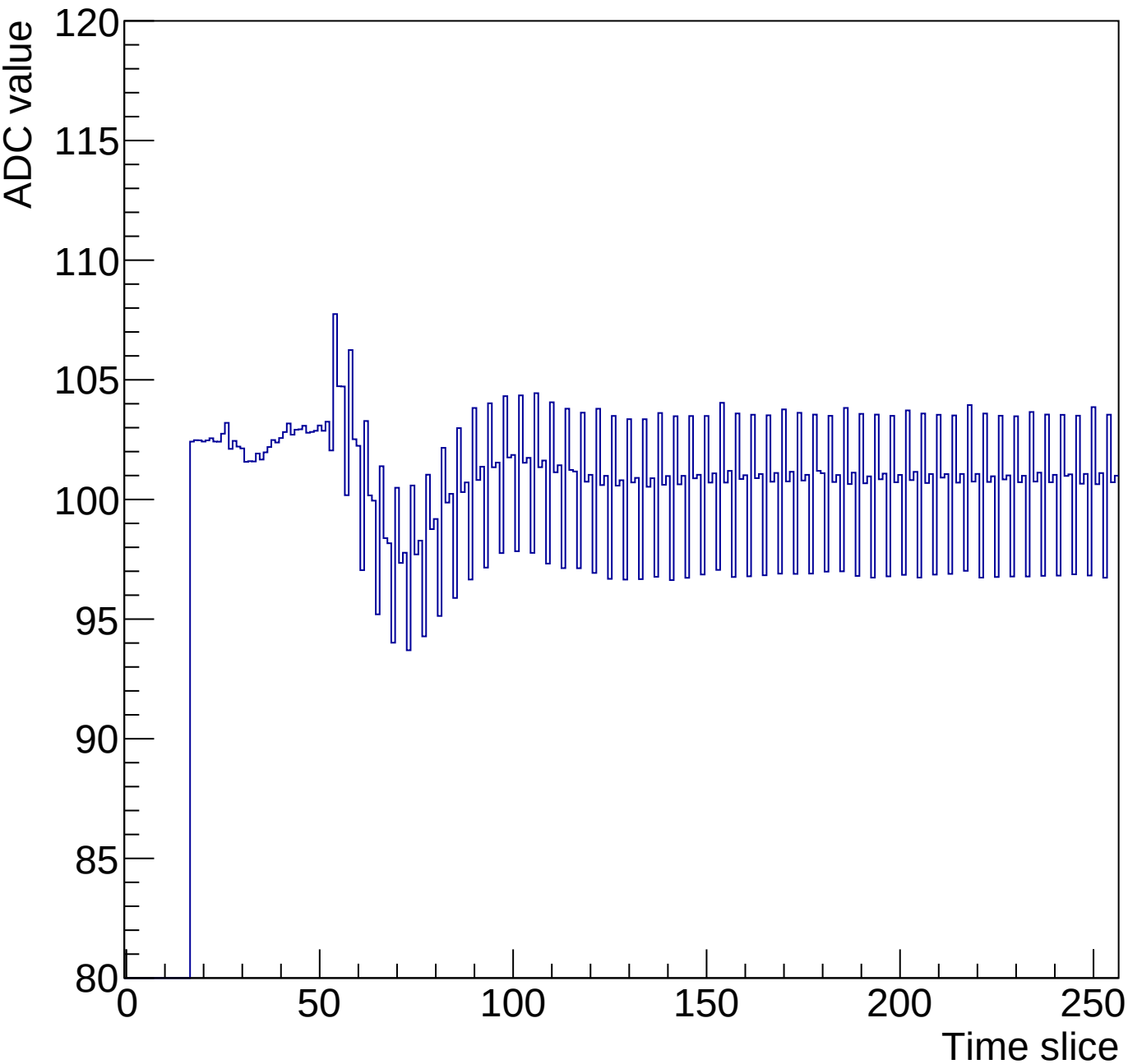
Run 3 Time mcm 0 chip 3 chan 14 256-30ns
