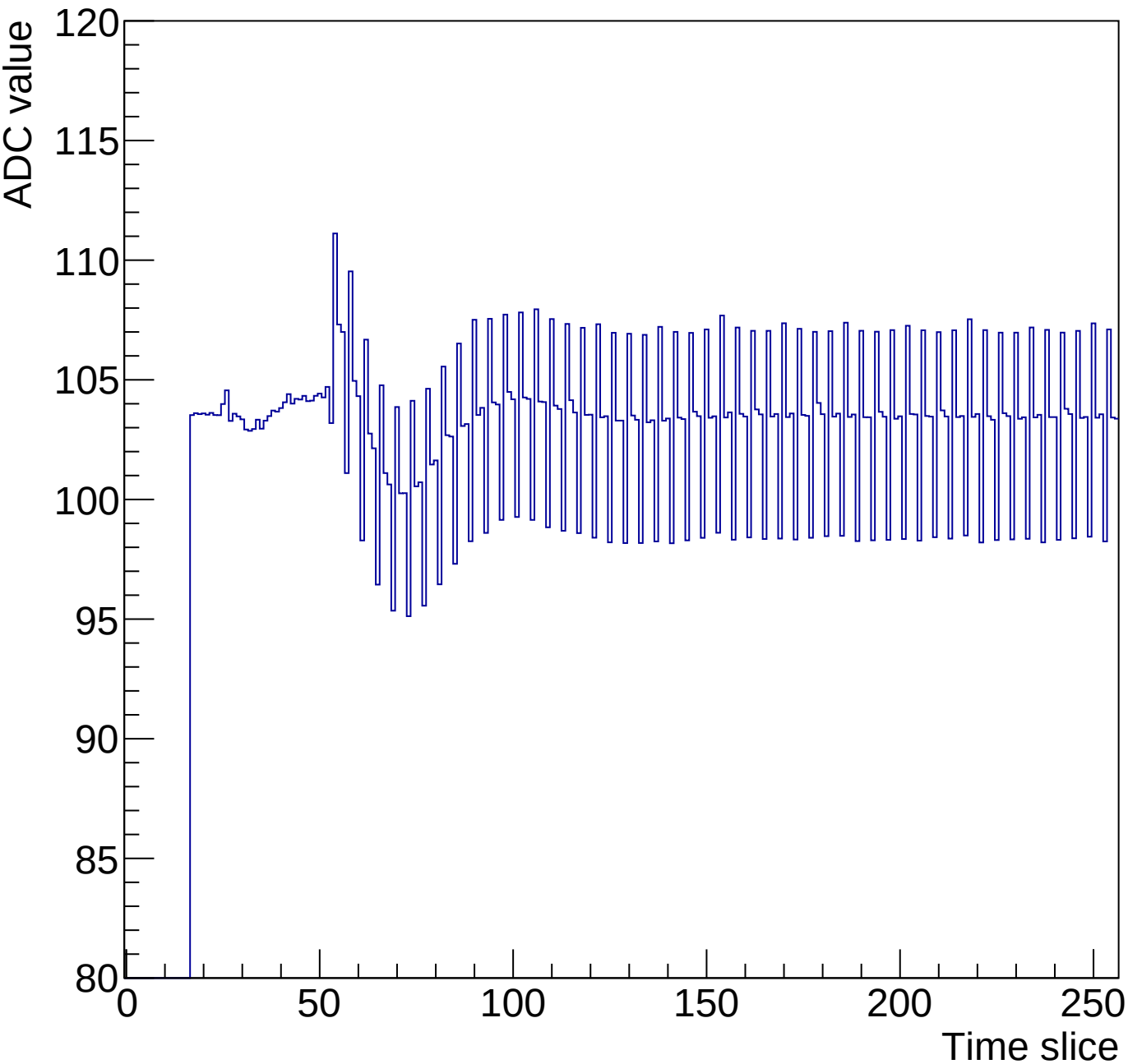
Run 3 Time mcm 0 chip 3 chan 12 256-30ns
