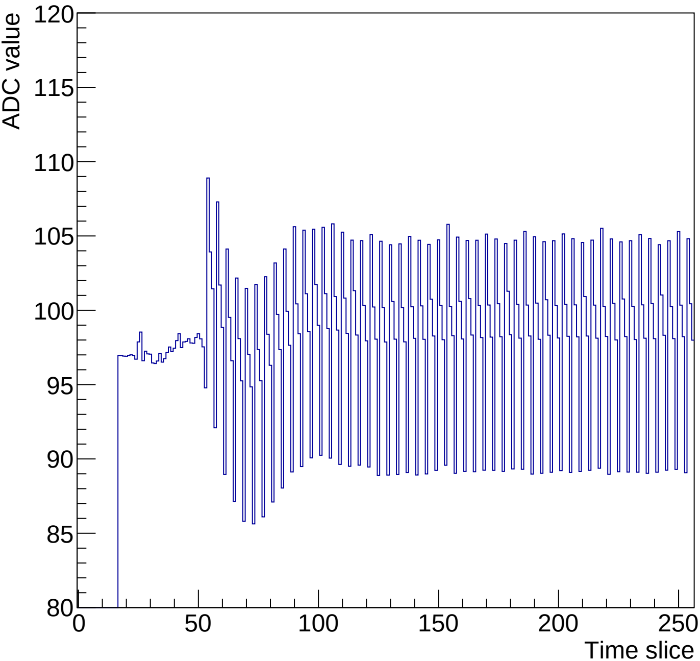
Run 3 Time mcm 0 chip 3 chan 4 256-30ns
