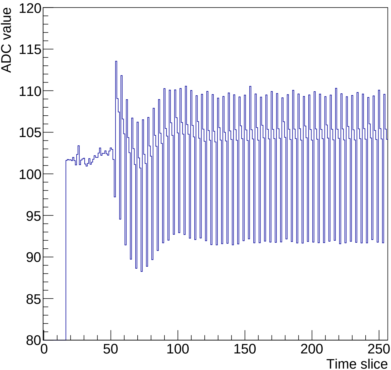
Run 3 Time mcm 0 chip 3 chan 1 256-30ns
