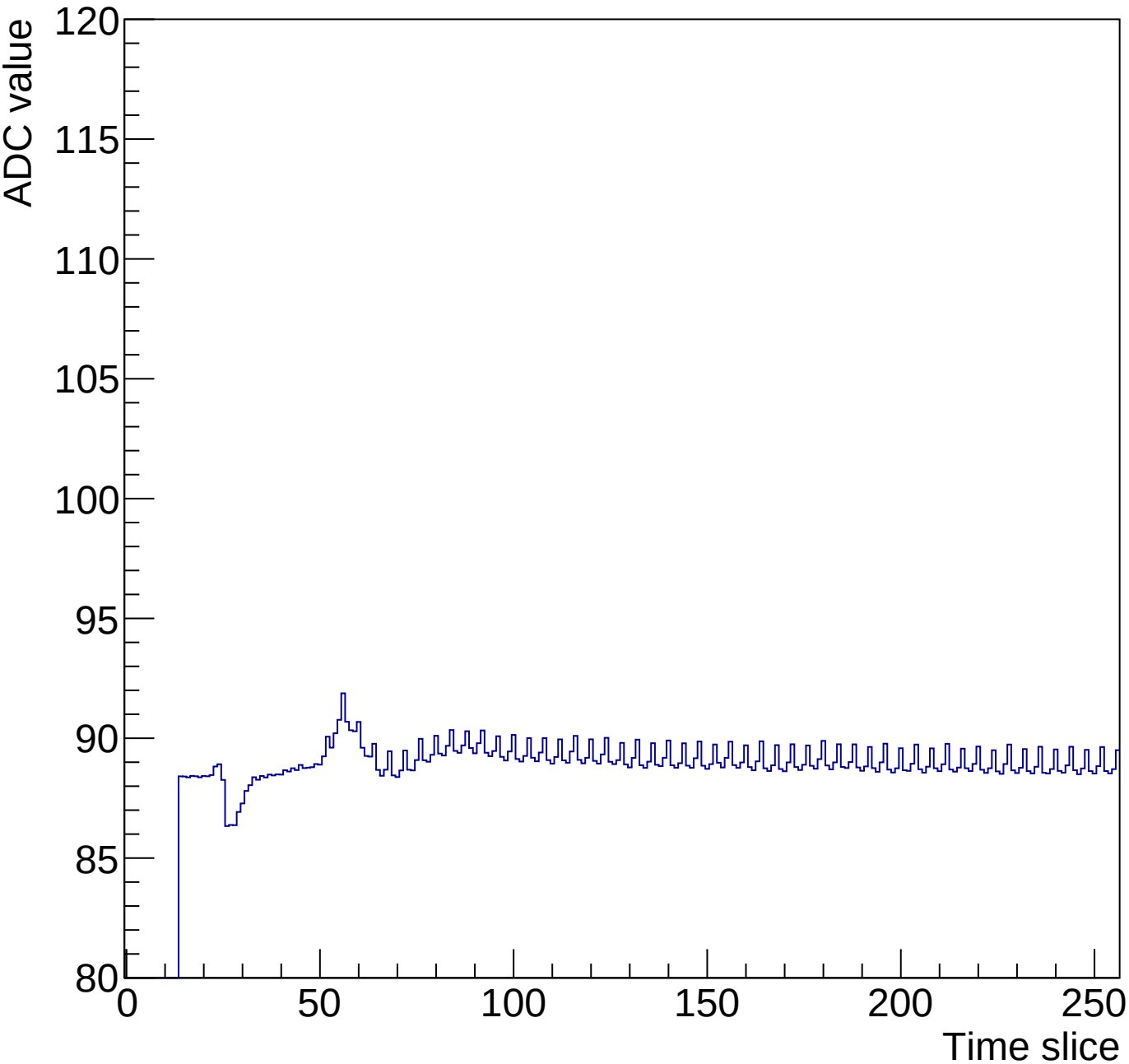
Run 0 Time mcm 1 chip 0 chan 0 256-120ns
