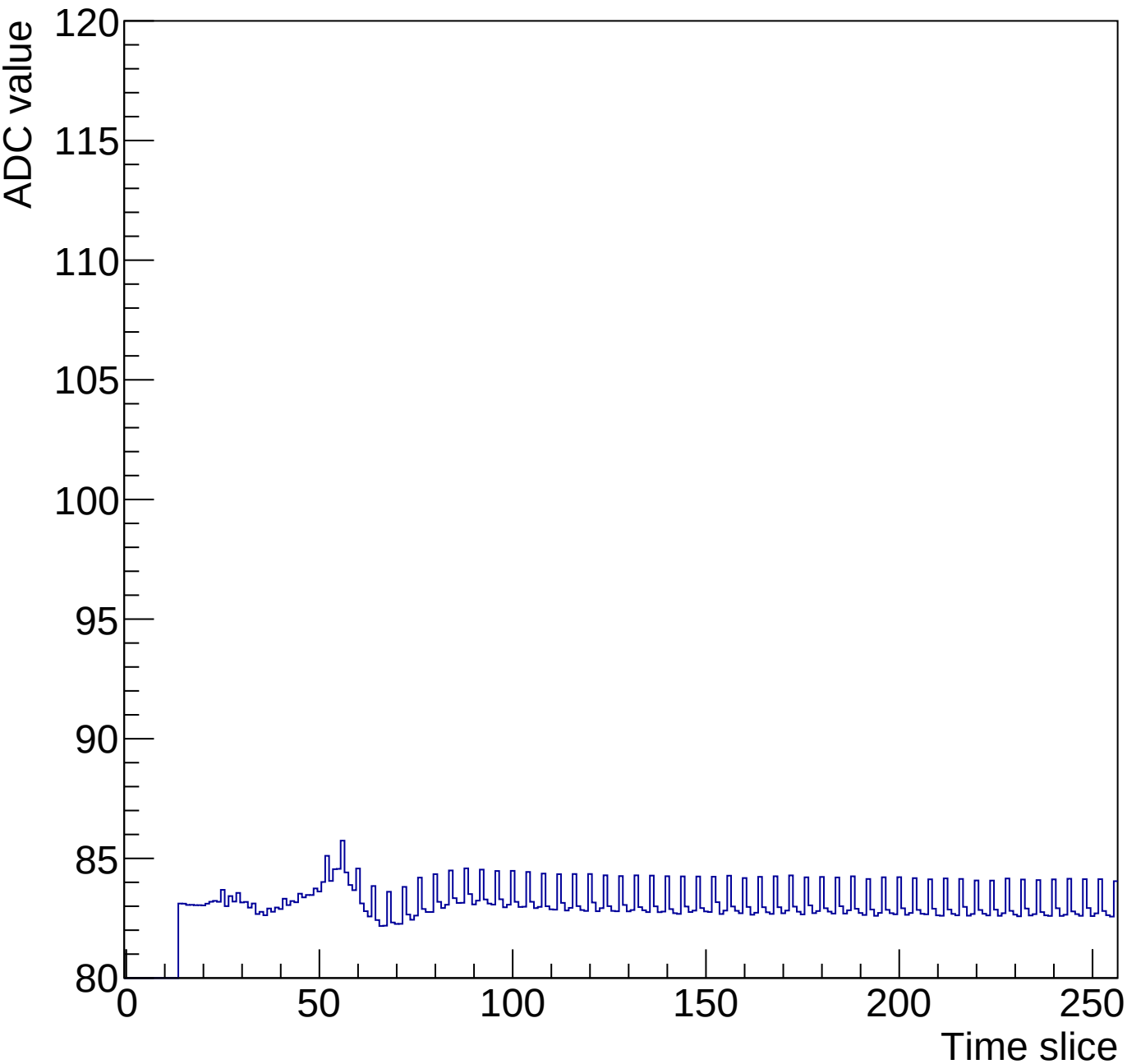
Run 1 Time mcm 1 chip 0 chan 13 256-90ns
