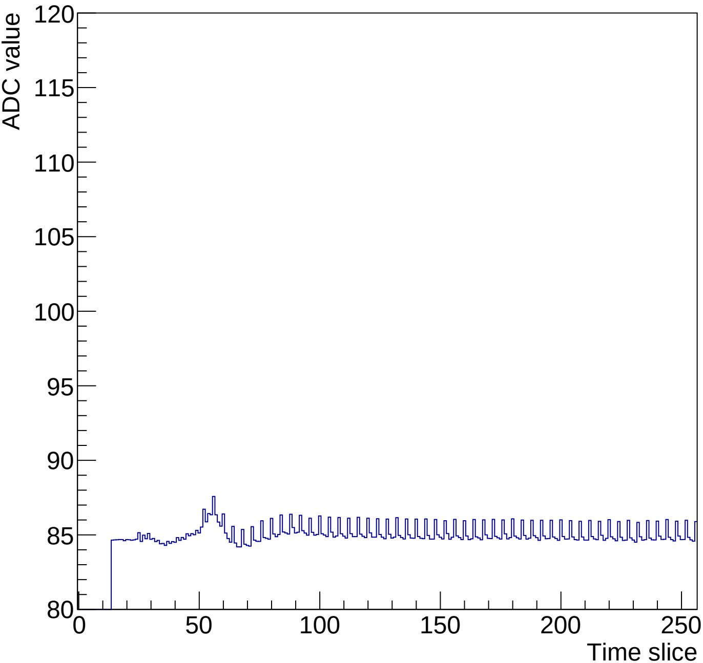
Run 1 Time mcm 1 chip 0 chan 12 256-90ns
