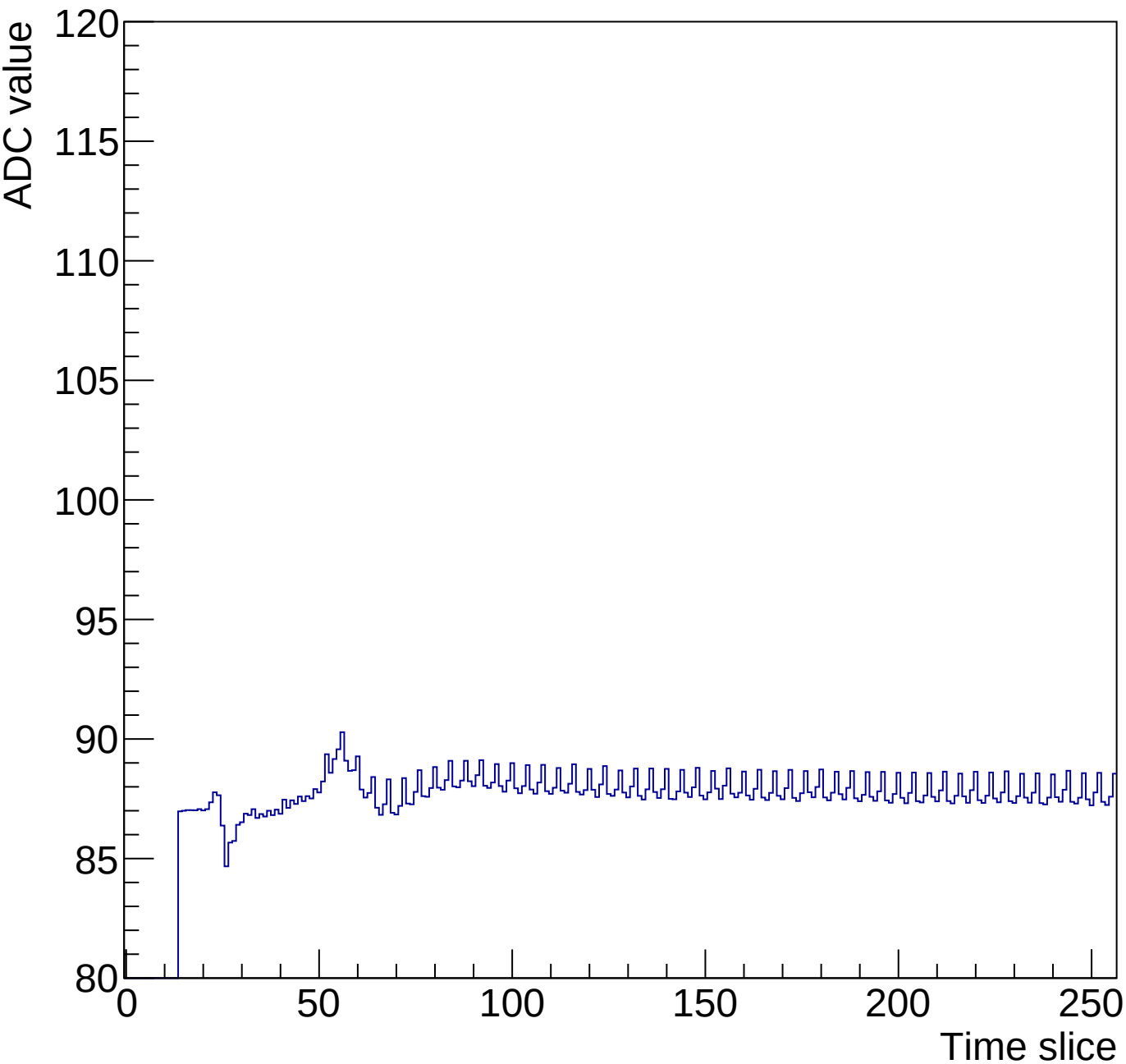
Run 1 Time mcm 1 chip 0 chan 0 256-90ns
