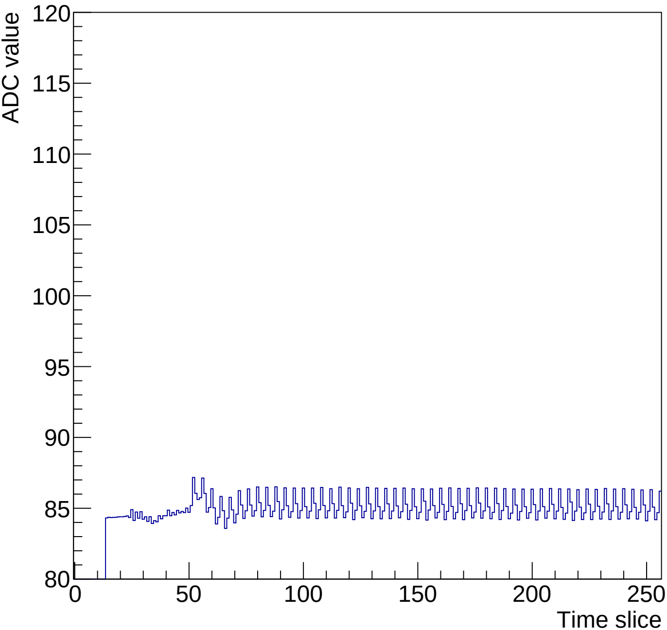
Run 2 Time mcm 1 chip 0 chan 8 256-60ns
