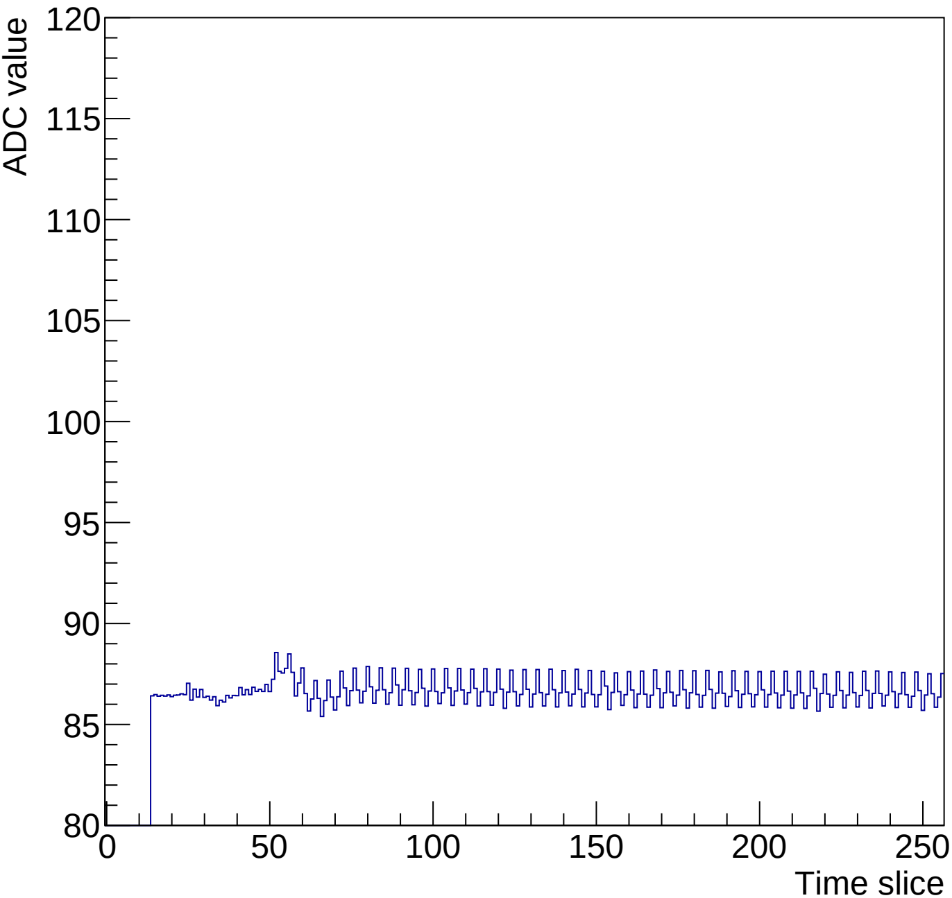
Run 2 Time mcm 1 chip 0 chan 10 256-60ns
