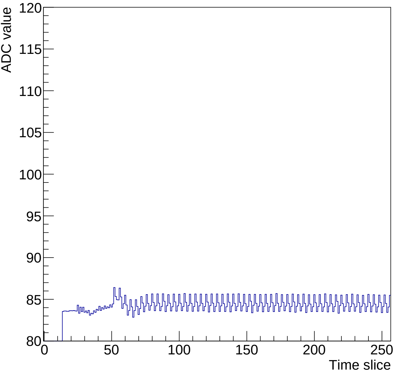
Run 2 Time mcm 1 chip 0 chan 12 256-60ns
