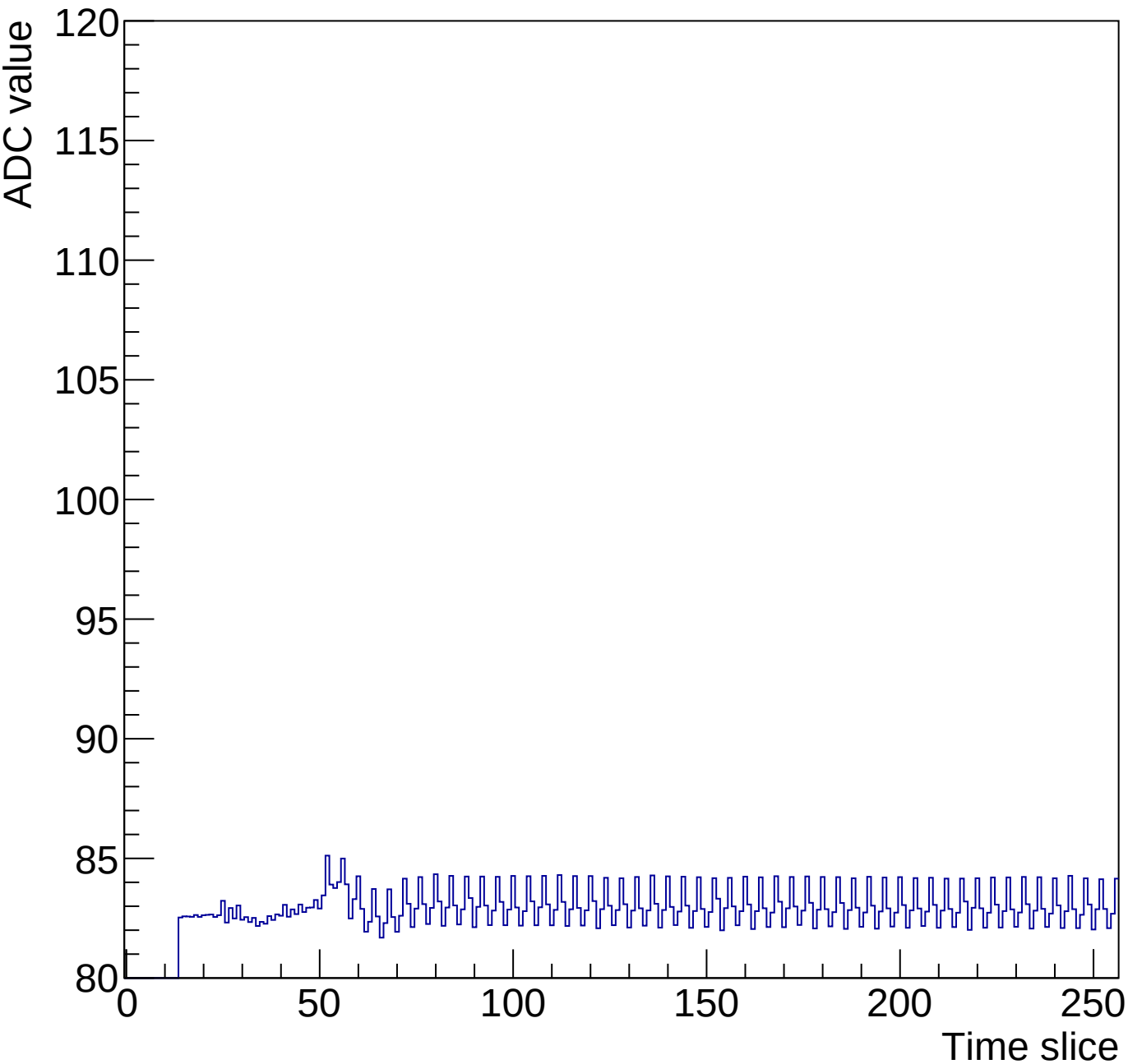
Run 2 Time mcm 1 chip 0 chan 13 256-60ns
