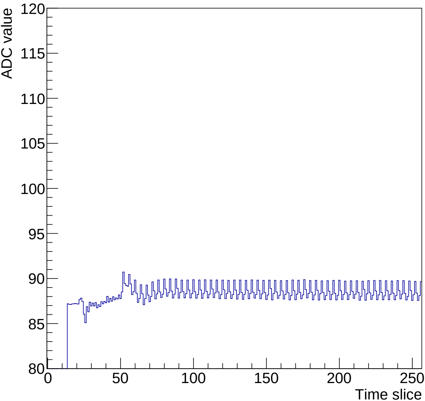
Run 2 Time mcm 1 chip 0 chan 0 256-60ns
