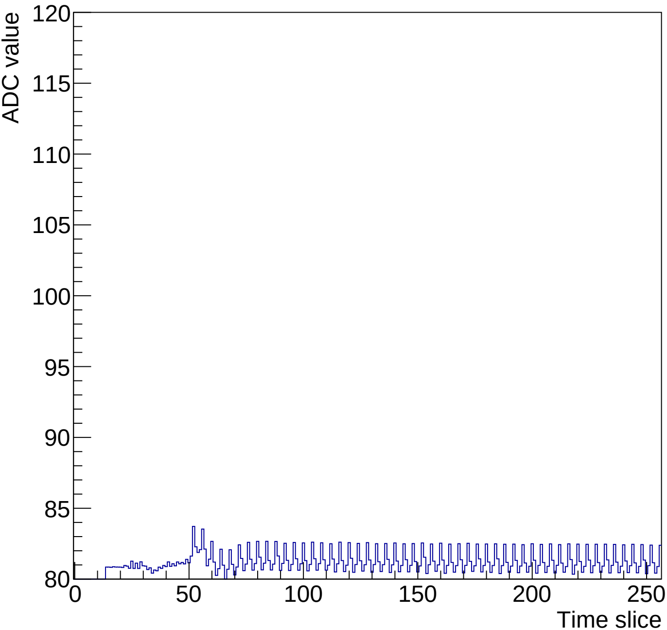
Run 2 Time mcm 1 chip 0 chan 15 256-60ns
