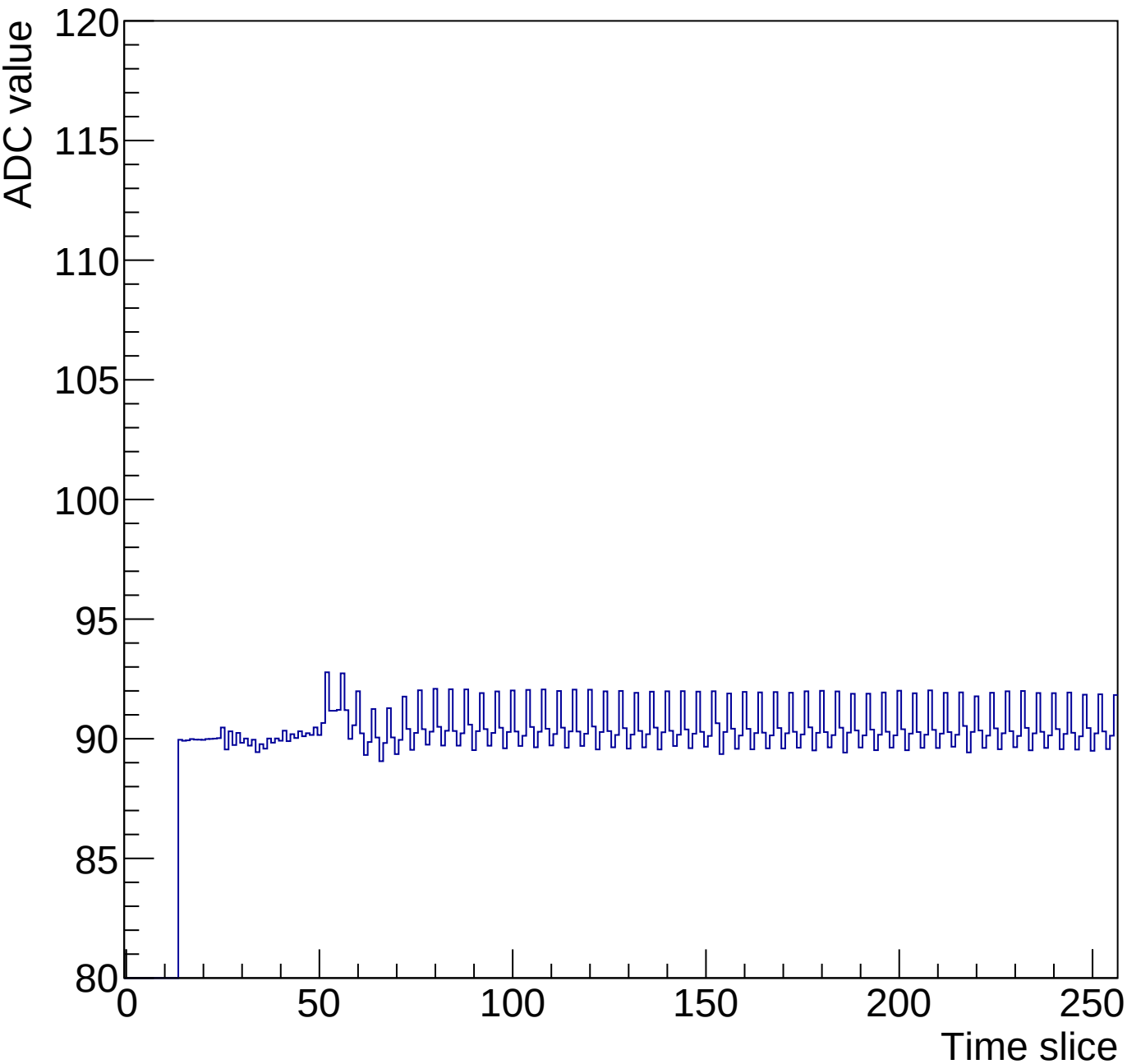
Run 2 Time mcm 1 chip 0 chan 6 256-60ns
