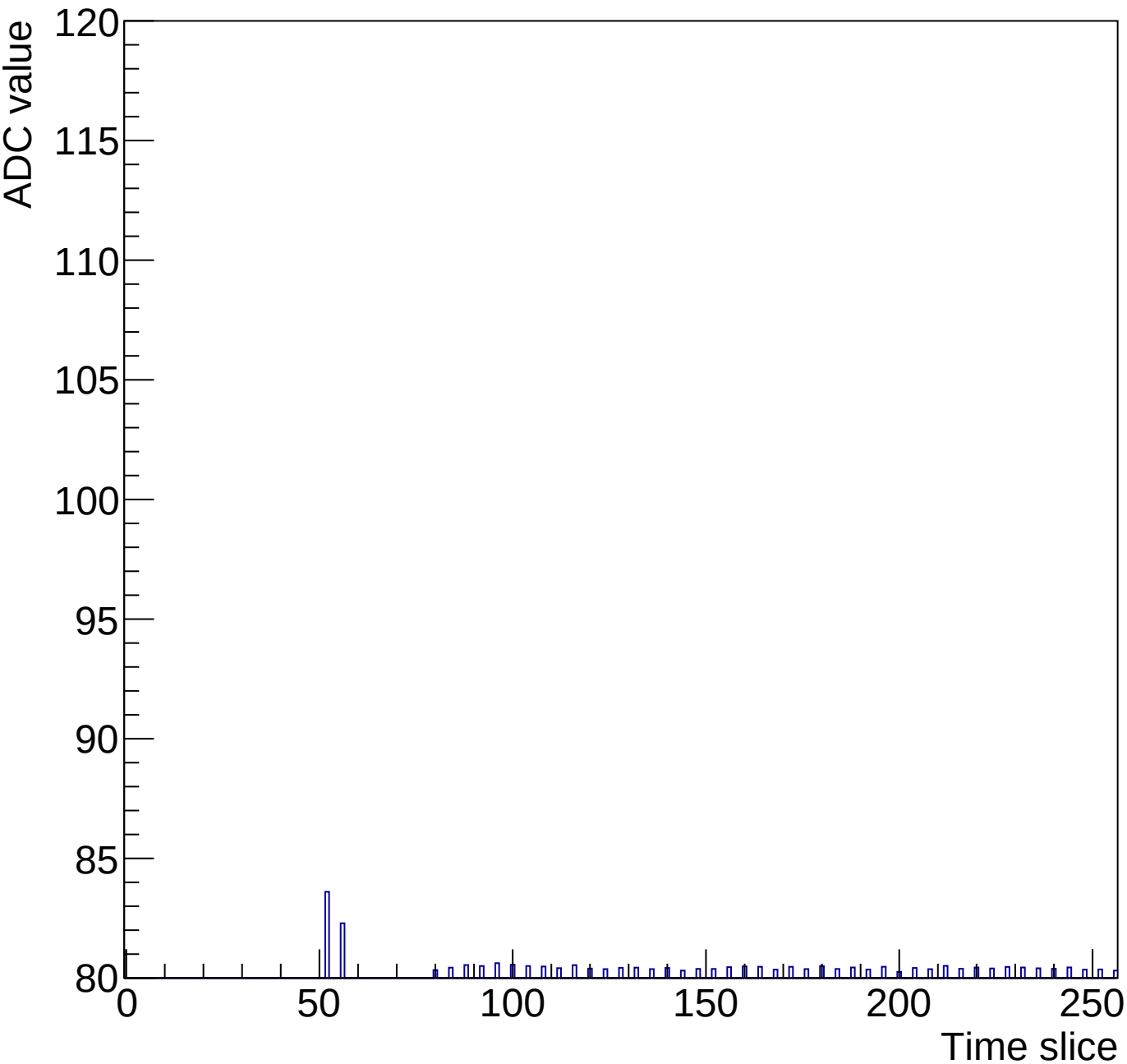
Run 3 Time mcm 1 chip 0 chan 3 256-30ns
