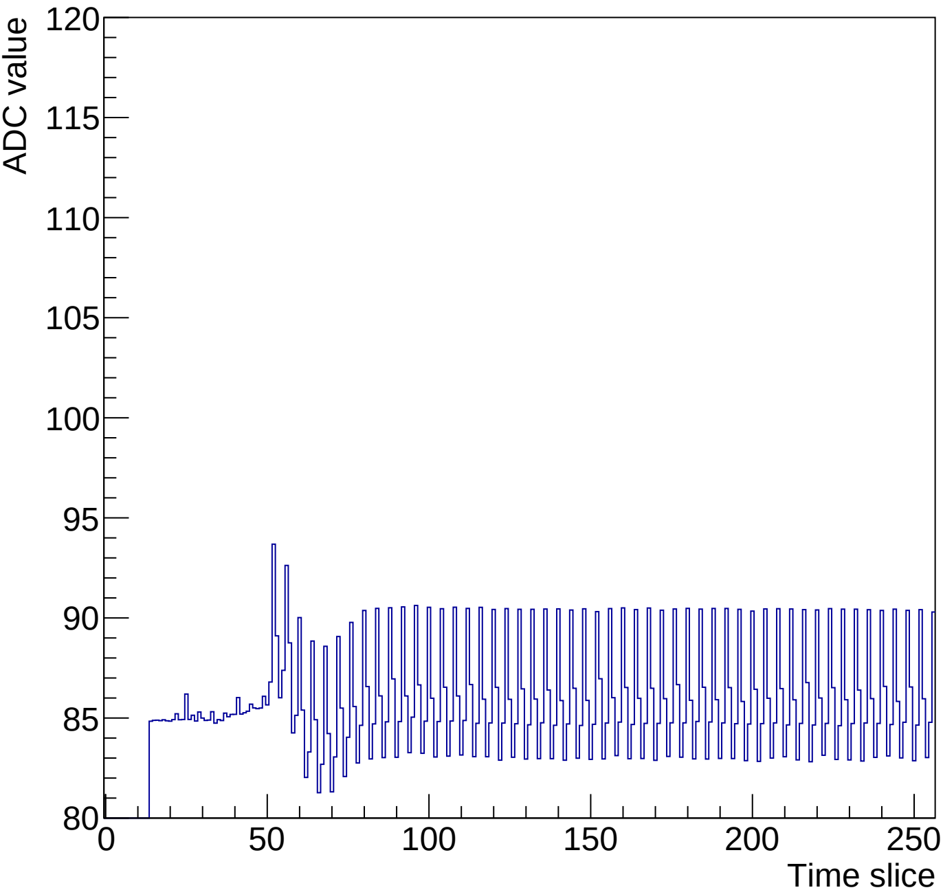
Run 3 Time mcm 1 chip 0 chan 4 256-30ns
