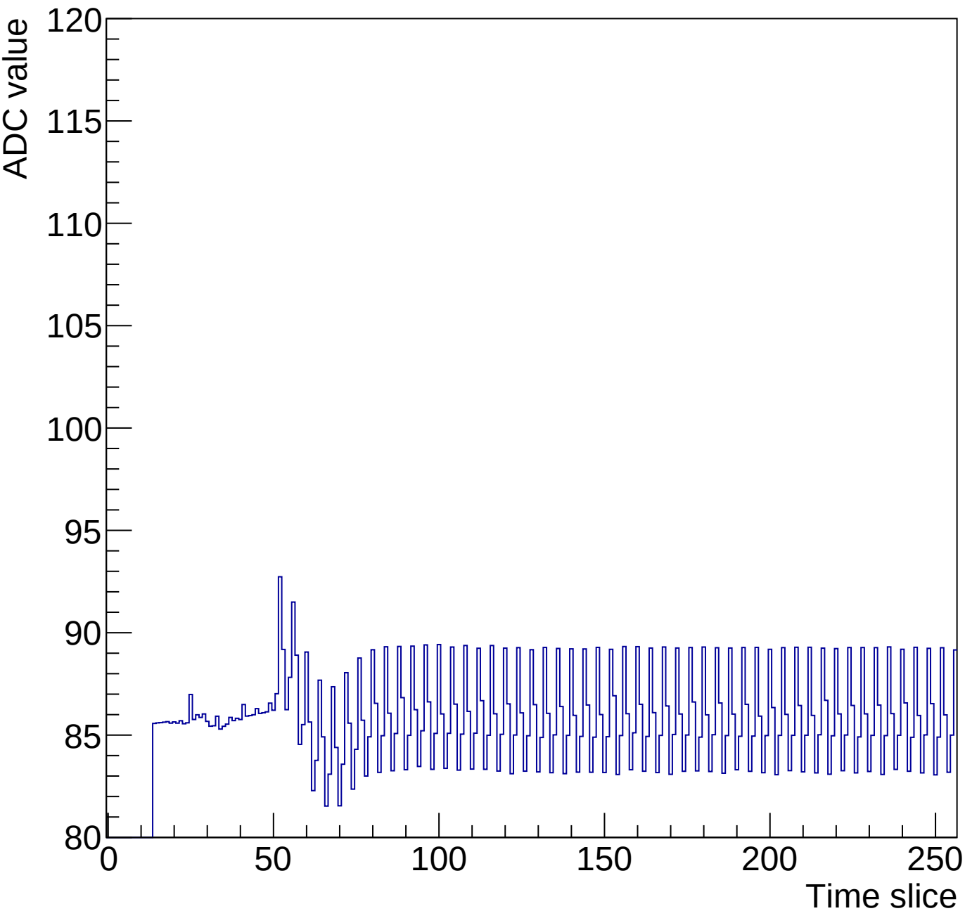
Run 3 Time mcm 1 chip 0 chan 8 256-30ns
