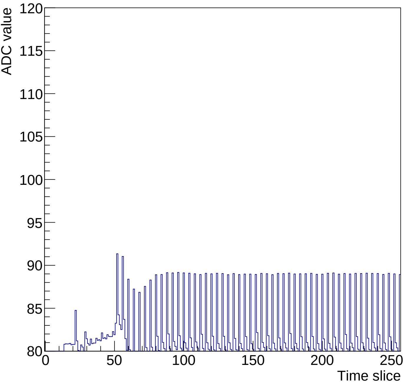
Run 3 Time mcm 1 chip 0 chan 1 256-30ns
