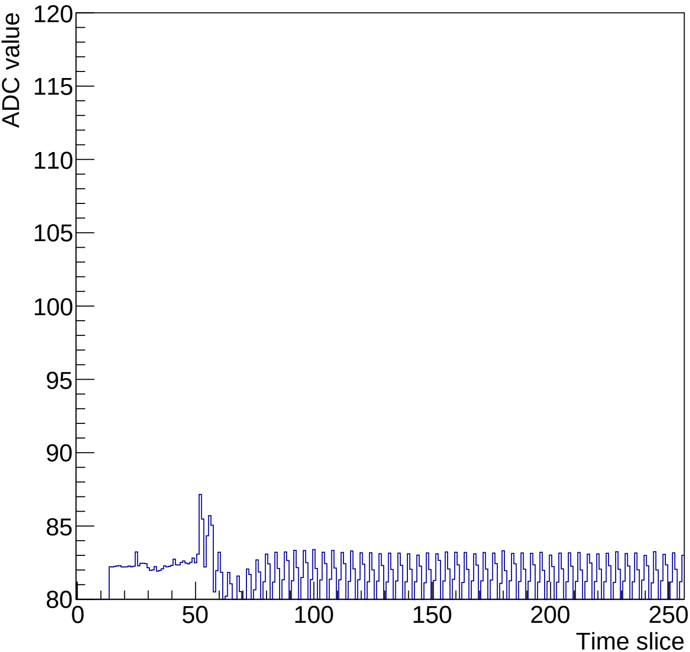
Run 3 Time mcm 1 chip 0 chan 13 256-30ns
