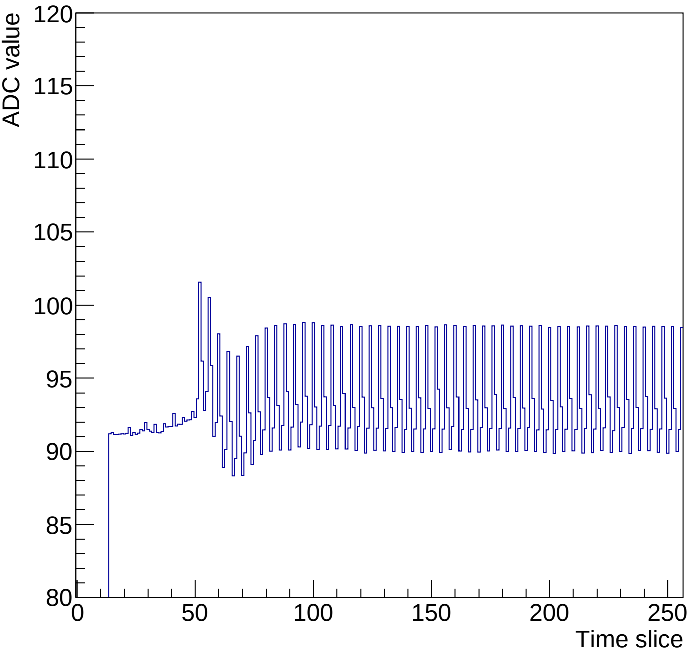
Run 3 Time mcm 1 chip 0 chan 0 256-30ns
