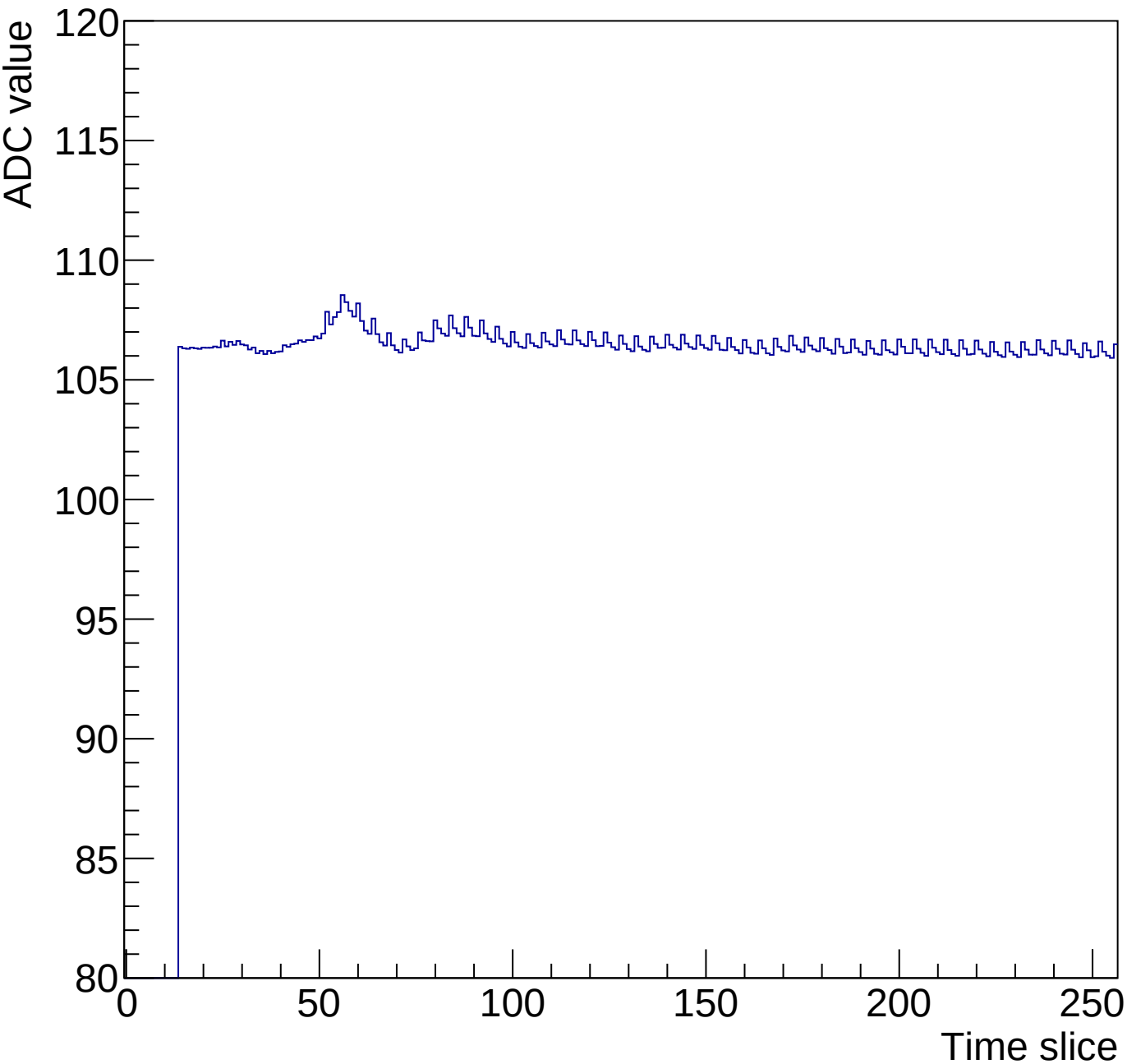
Run 0 Time mcm 2 chip 0 chan 0 256-120ns
