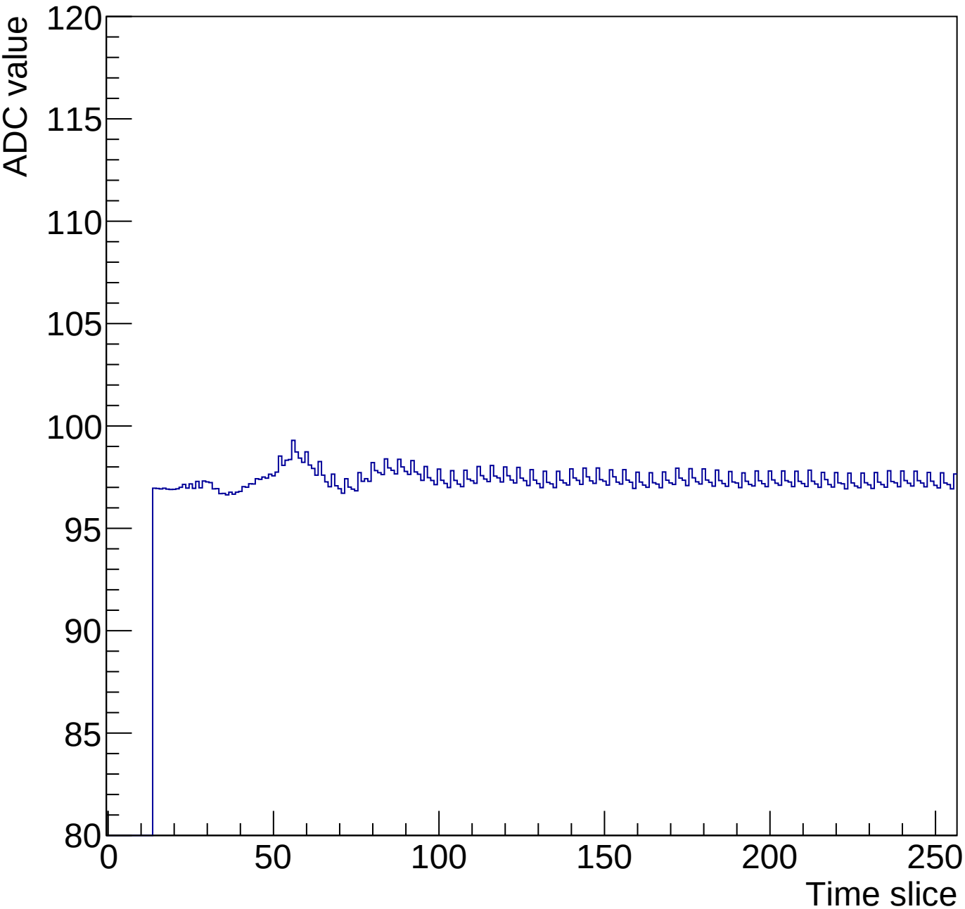
Run 0 Time mcm 2 chip 0 chan 15 256-120ns
