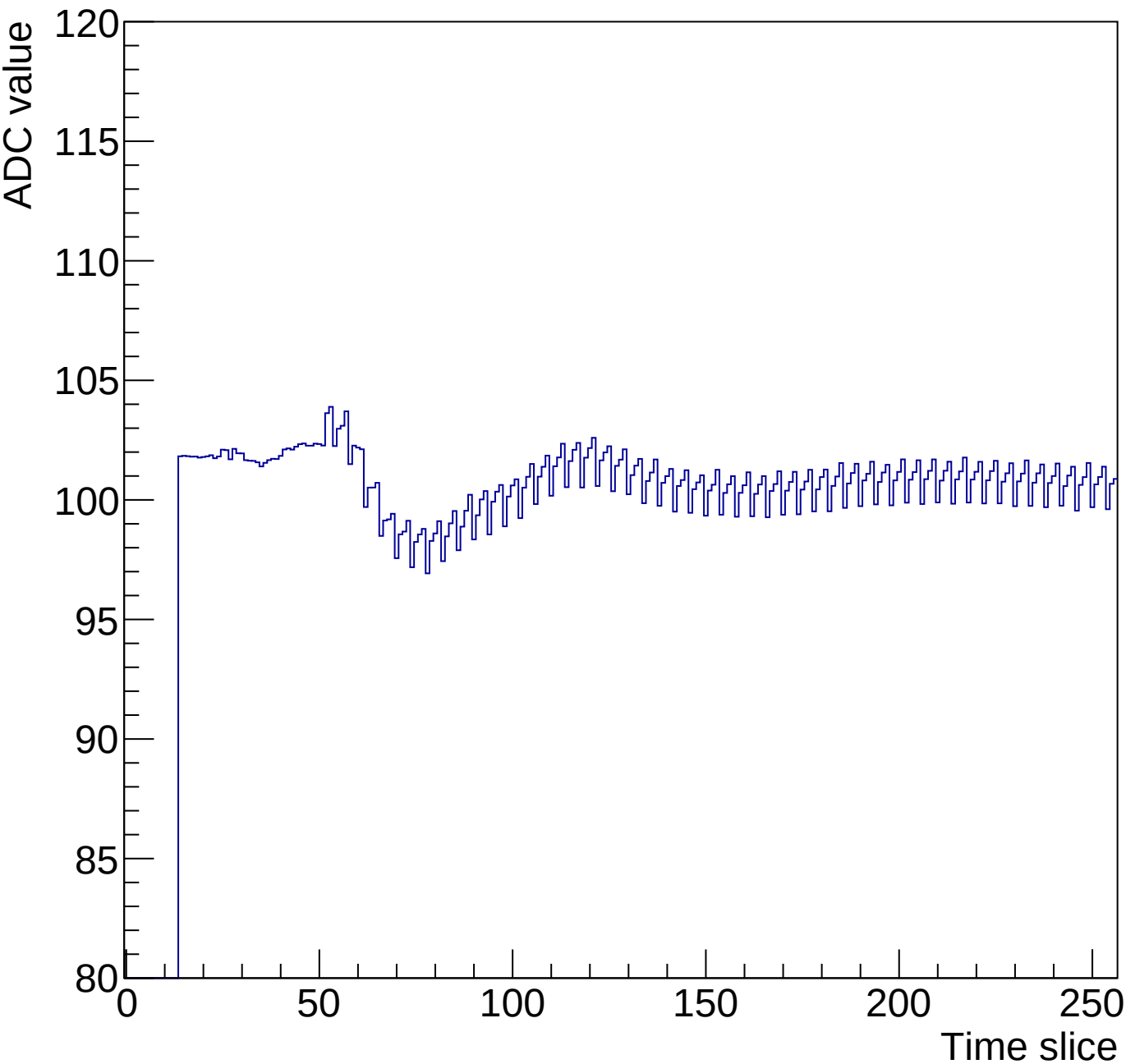
Run 3 Time mcm 2 chip 0 chan 0 256-30ns
