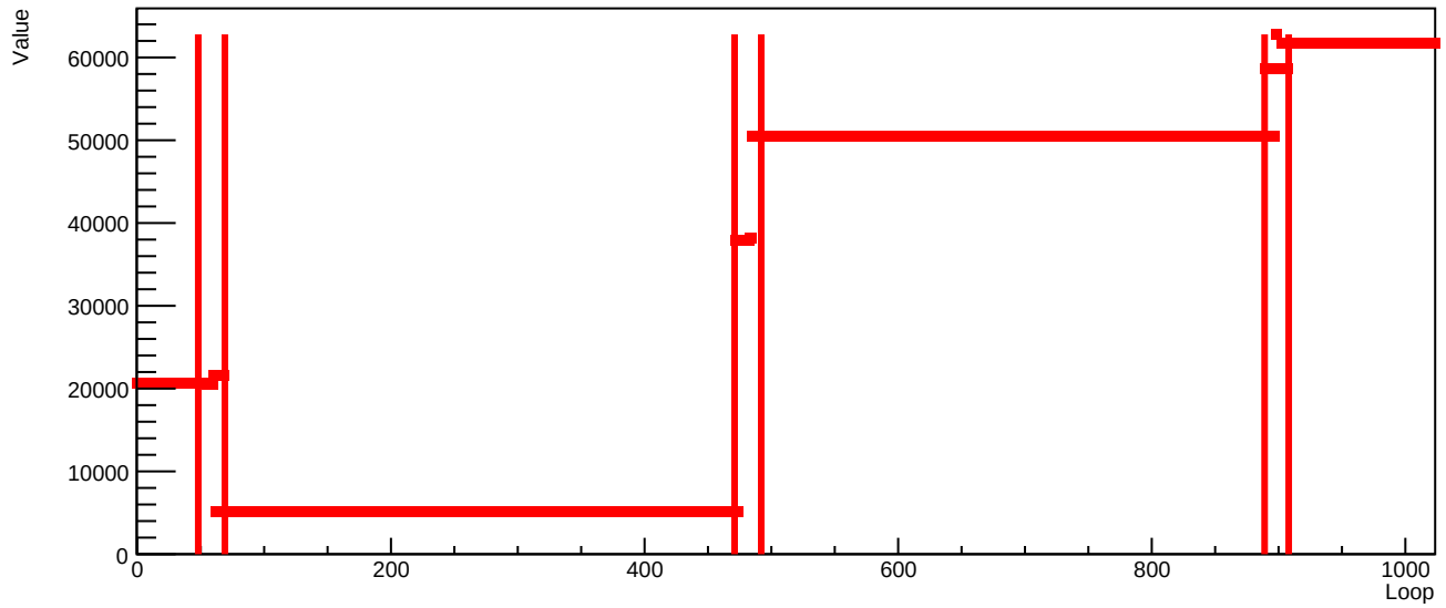
DCL timing3-reset22.csv MCM1 ID97
