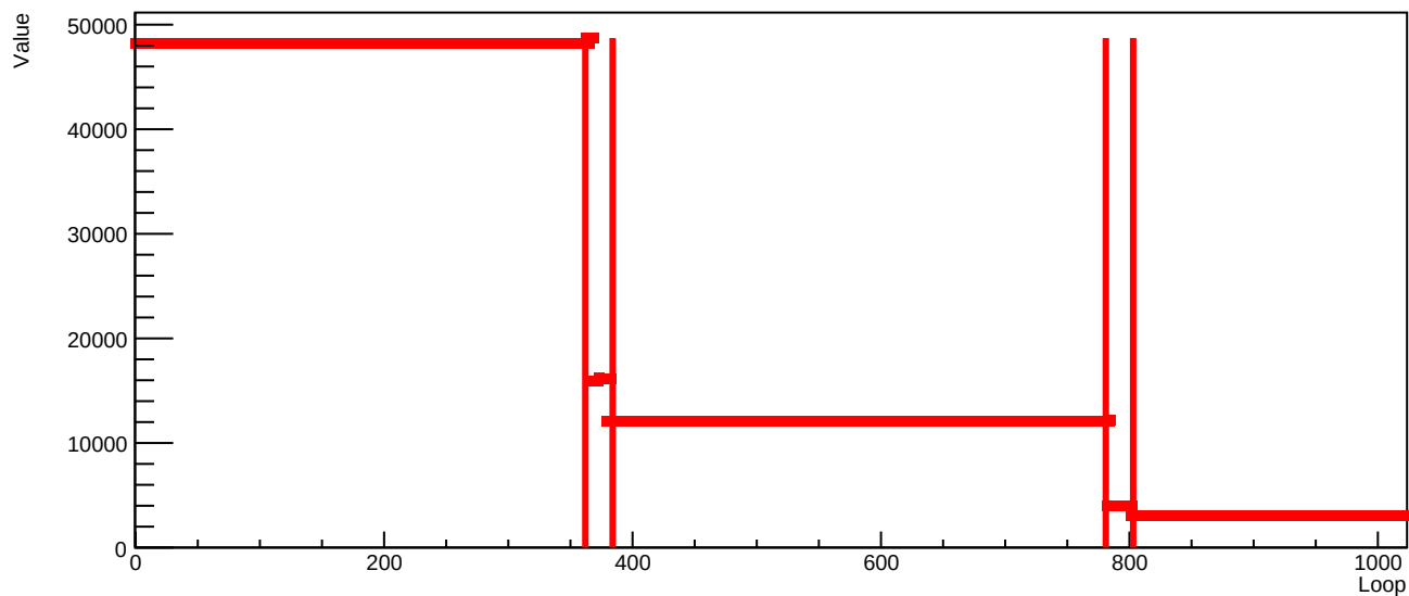
DCL timing3-reset34.csv MCM1 ID491
