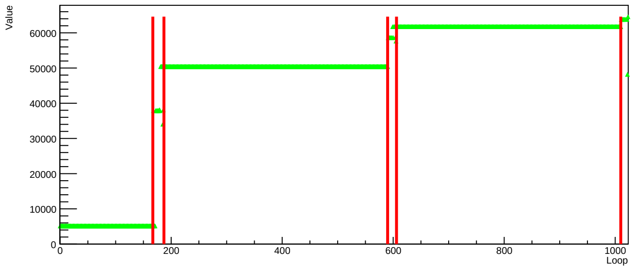
DCL timing3-reset82.csv MCM2 ID508
