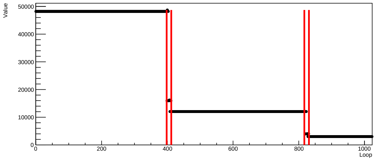
DCL timing3-reset29.csv MCM0 ID253
