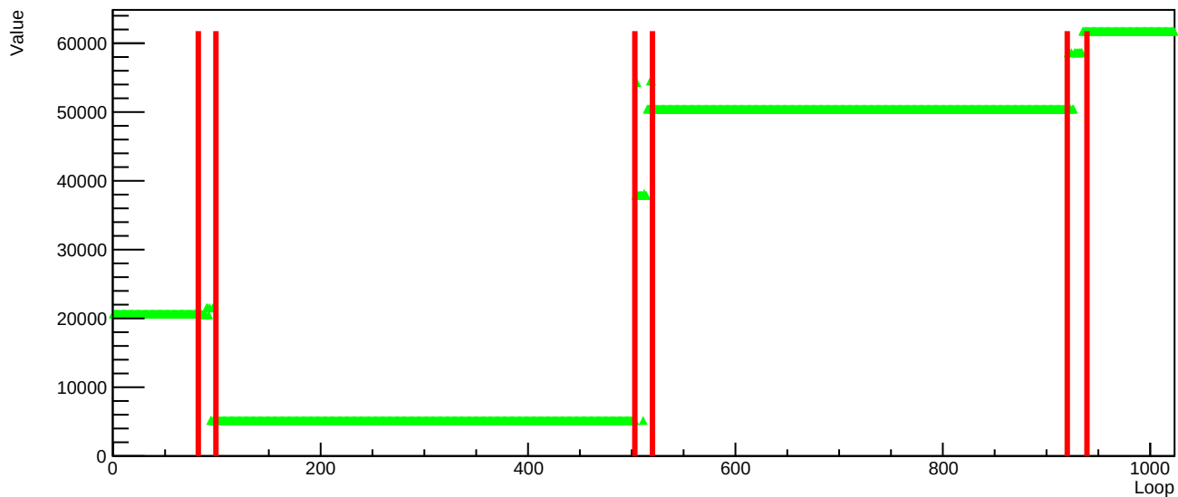
DCL timing3-reset48.csv MCM2 ID717
