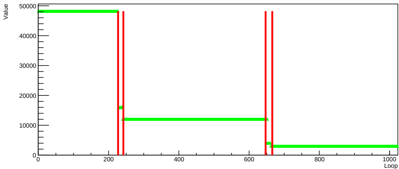
DCL timing3-reset36.csv MCM2 ID16
