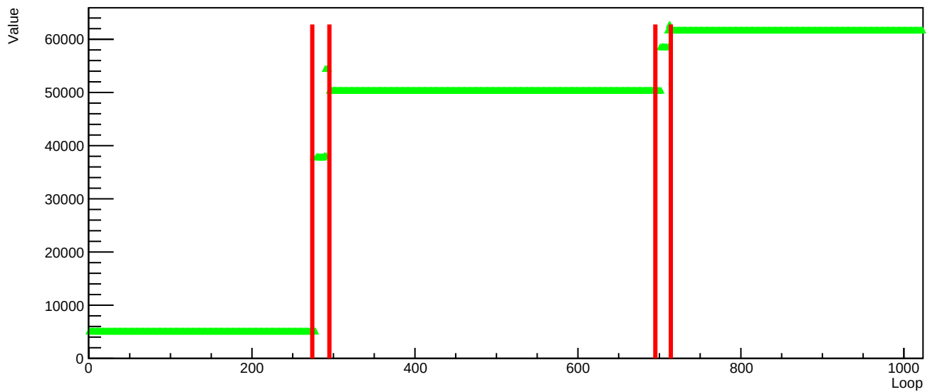
DCL timing3-reset38.csv MCM2 ID16
