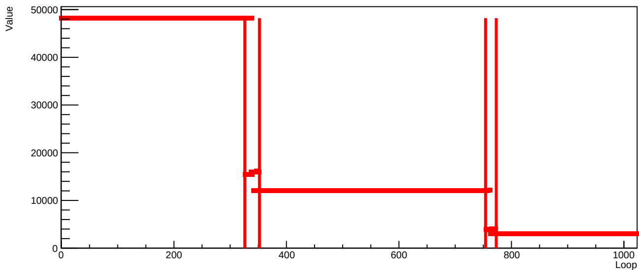
DCL timing3-reset50.csv MCM1 ID19
