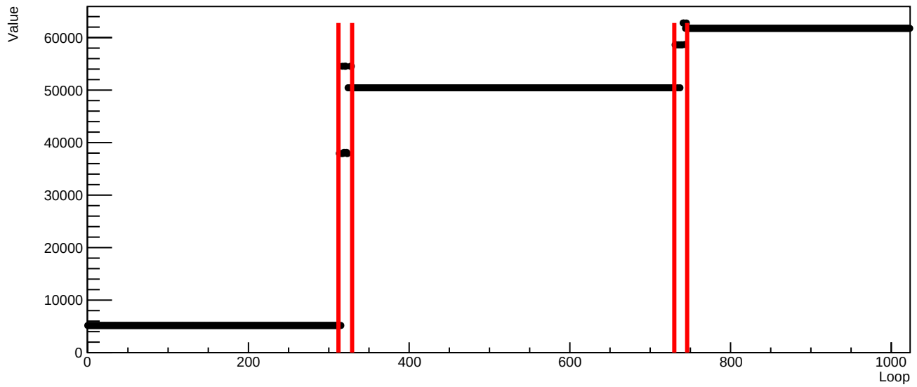
DCL timing3-reset53.csv MCM0 ID0
