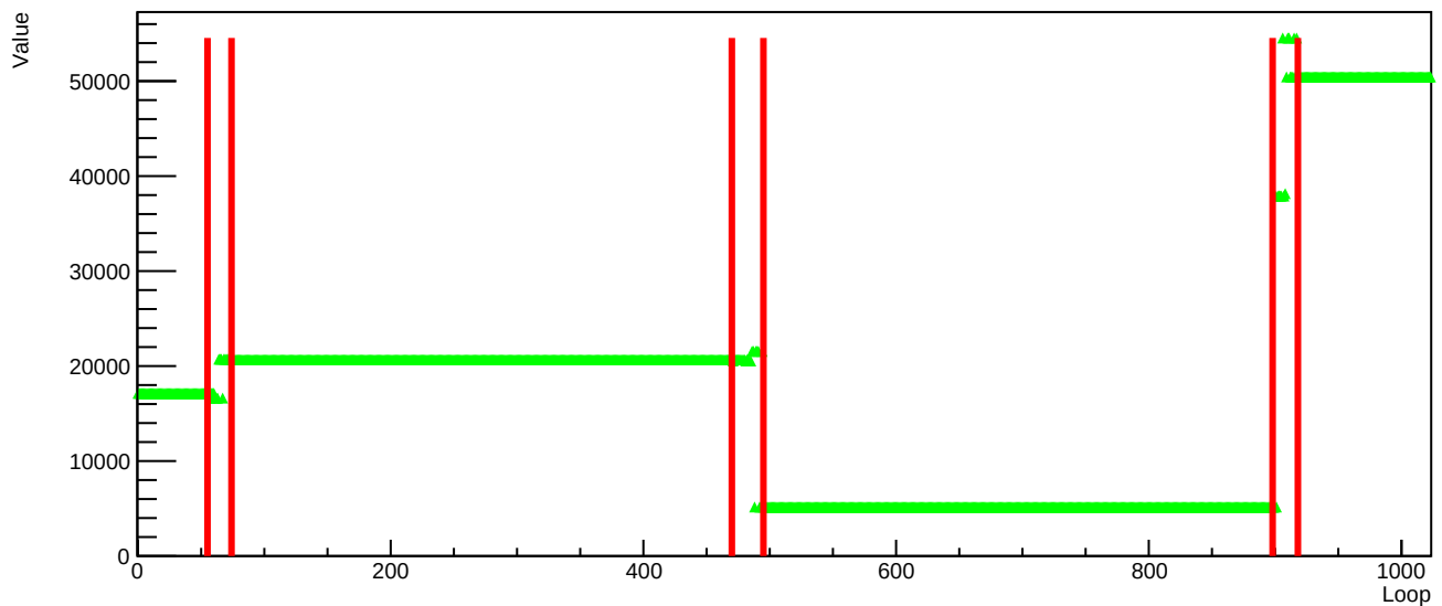
DCL timing3-reset58.csv MCM2 ID24
