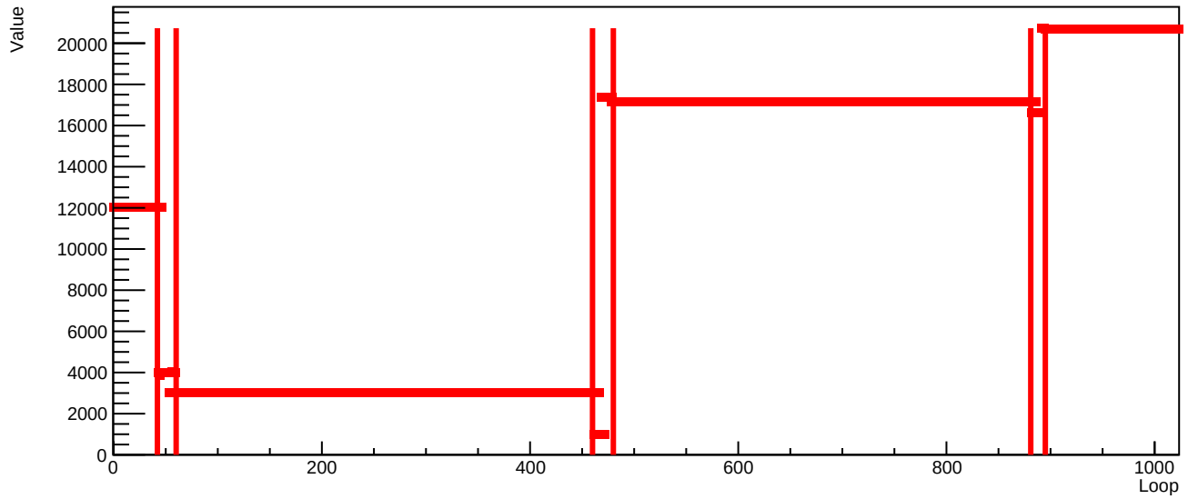
DCL timing3-reset58.csv MCM1 ID23
