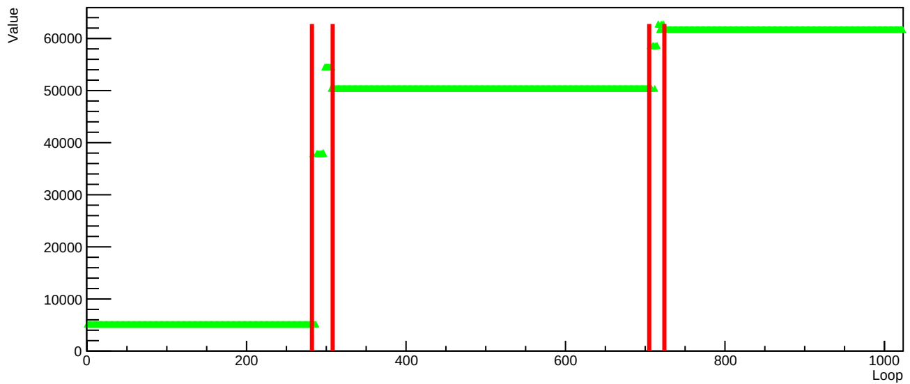
DCL timing3-reset68.csv MCM2 ID28
