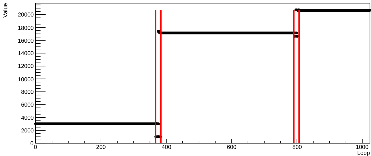
DCL timing3-reset75.csv MCM0 ID0
