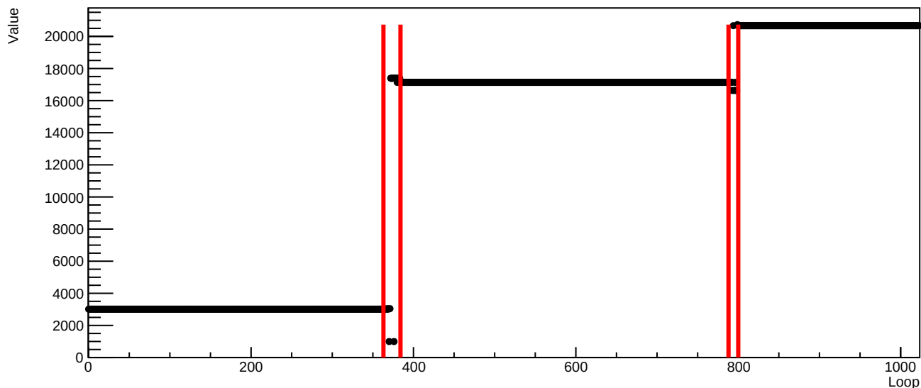
DCL timing3-reset9.csv MCM0 ID0
