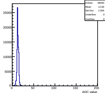
Pedestals mcm 0 ch 10 chamber-1
