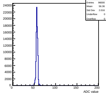
Pedestals mcm 0 ch 3 chamber-1
