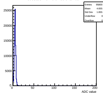
Pedestals mcm 0 ch 39 chamber-1
