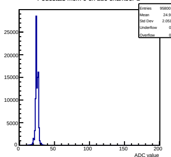
Pedestals mcm 0 ch 110 chamber-1
