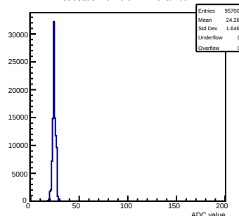
Pedestals mcm 0 ch 127 chamber-1
