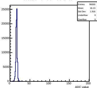
Pedestals mcm 0 ch 76 chamber-1
