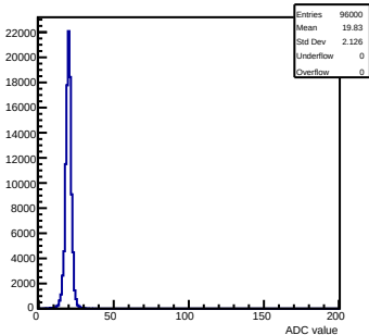
Pedestals mcm 0 ch 64 chamber-1
