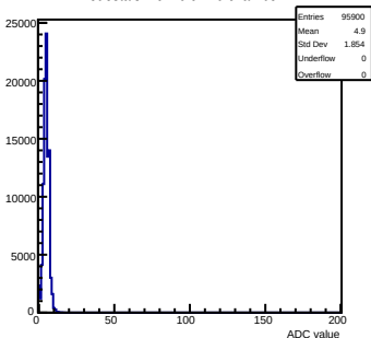
Pedestals mcm 0 ch 20 chamber-1
