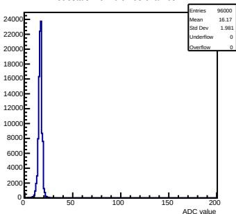
Pedestals mcm 0 ch 68 chamber-1
