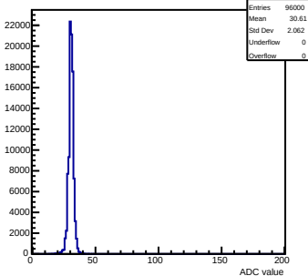
Pedestals mcm 0 ch 0 chamber-1
