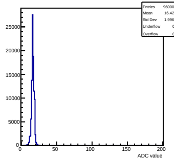
Pedestals mcm 0 ch 66 chamber-1
