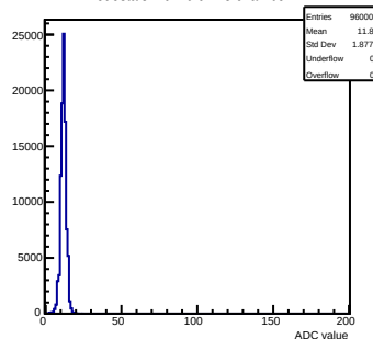
Pedestals mcm 0 ch 78 chamber-1
