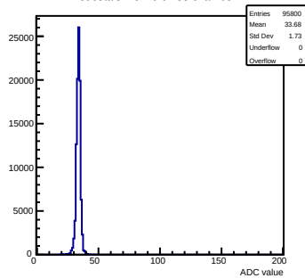
Pedestals mcm 0 ch 33 chamber-1
