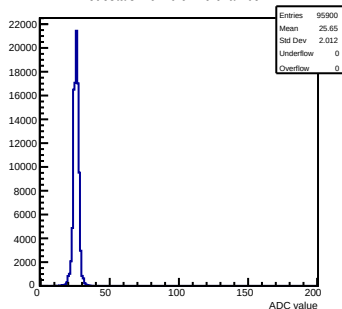
Pedestals mcm 0 ch 29 chamber-1
