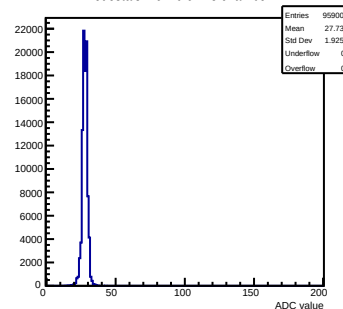
Pedestals mcm 0 ch 23 chamber-1
