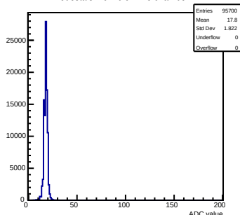
Pedestals mcm 0 ch 125 chamber-1
