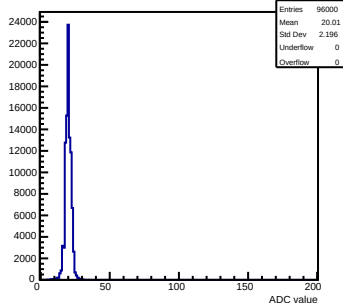
Pedestals mcm 0 ch 9 chamber-1
