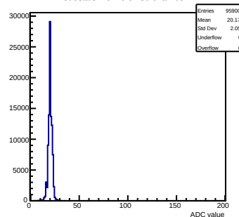
Pedestals mcm 0 ch 30 chamber-1
