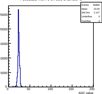
Pedestals mcm 0 ch 105 chamber-1
