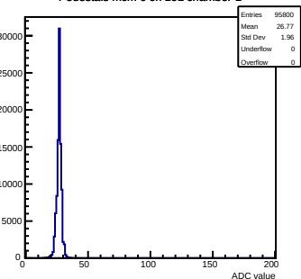
Pedestals mcm 0 ch 101 chamber-1
