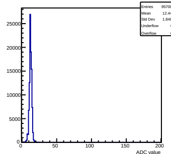
Pedestals mcm 0 ch 118 chamber-1
