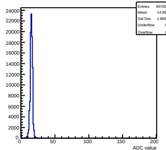
Pedestals mcm 0 ch 115 chamber-1
