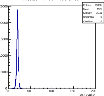
Pedestals mcm 0 ch 109 chamber-1
