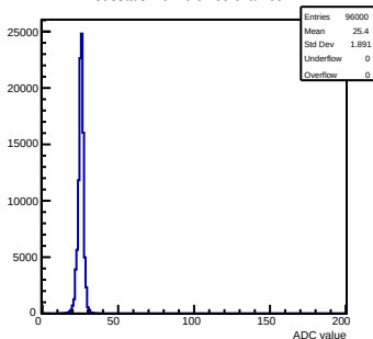
Pedestals mcm 0 ch 69 chamber-1
