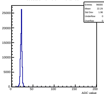
Pedestals mcm 0 ch 77 chamber-1
