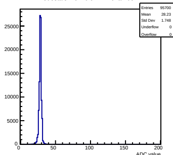
Pedestals mcm 0 ch 121 chamber-1
