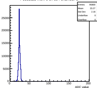
Pedestals mcm 0 ch 104 chamber-1
