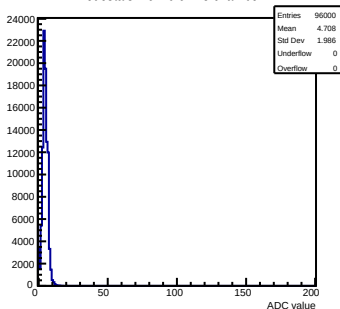
Pedestals mcm 0 ch 73 chamber-1
