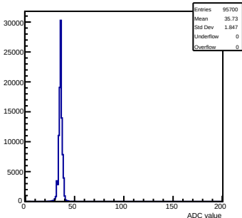
Pedestals mcm 0 ch 116 chamber-1
