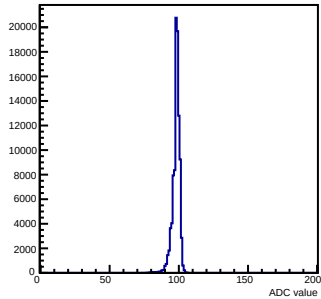
Pedestals mcm 0 ch 107 chamber-fec0
