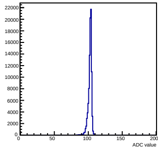
Pedestals mcm 0 ch 45 chamber-fec0
