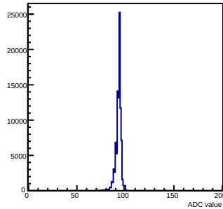
Pedestals mcm 0 ch 70 chamber-fec0
