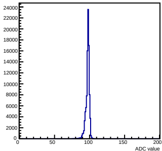
Pedestals mcm 0 ch 53 chamber-fec0
