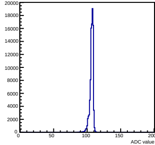
Pedestals mcm 0 ch 69 chamber-fec0
