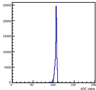
Pedestals mcm 0 ch 121 chamber-fec0
