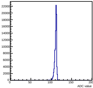
Pedestals mcm 0 ch 100 chamber-fec0
