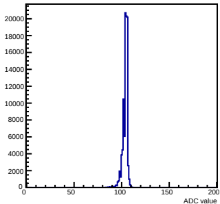
Pedestals mcm 0 ch 61 chamber-fec0
