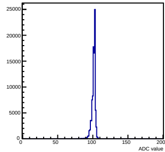
Pedestals mcm 0 ch 43 chamber-fec0
