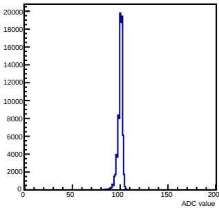
Pedestals mcm 0 ch 44 chamber-fec0
