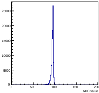
Pedestals mcm 0 ch 17 chamber-fec0
