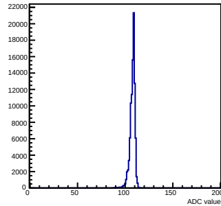
Pedestals mcm 0 ch 83 chamber-fec0
