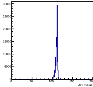
Pedestals mcm 0 ch 2 chamber-fec0
