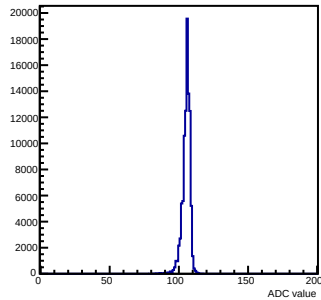
Pedestals mcm 0 ch 50 chamber-fec0
