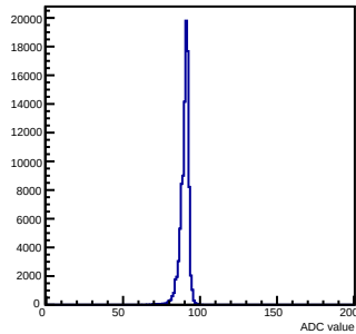
Pedestals mcm 0 ch 51 chamber-fec0
