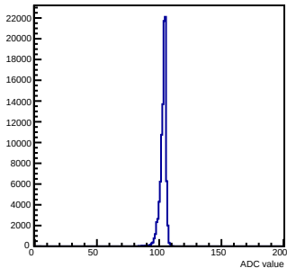
Pedestals mcm 0 ch 89 chamber-fec0
