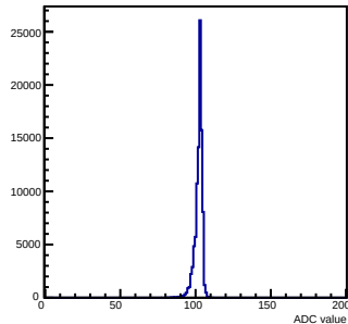
Pedestals mcm 0 ch 55 chamber-fec0
