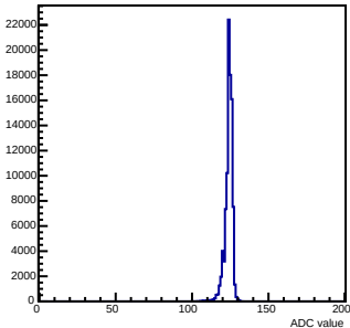
Pedestals mcm 0 ch 12 chamber-fec0
