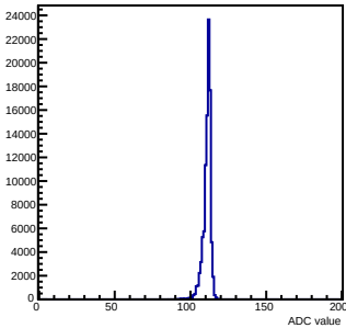
Pedestals mcm 0 ch 108 chamber-fec0
