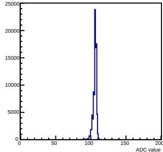
Pedestals mcm 0 ch 58 chamber-fec0
