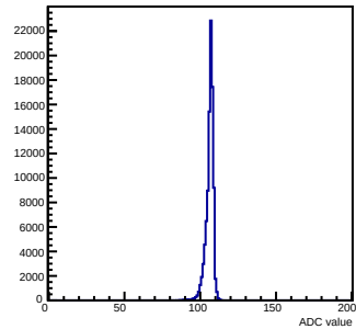
Pedestals mcm 0 ch 47 chamber-fec0
