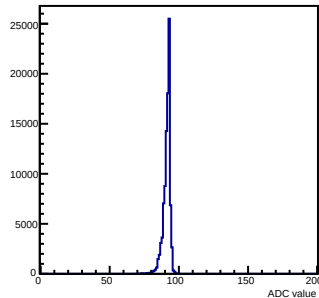
Pedestals mcm 0 ch 86 chamber-fec0
