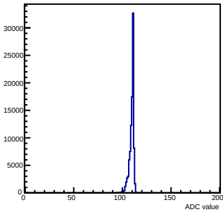
Pedestals mcm 0 ch 32 chamber-fec0
