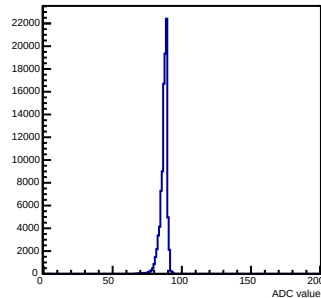
Pedestals mcm 0 ch 87 chamber-fec0
