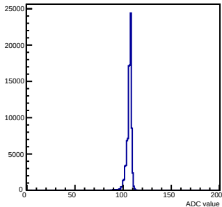
Pedestals mcm 0 ch 93 chamber-fec0
