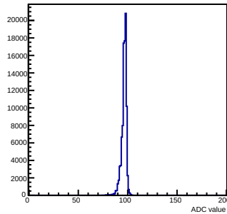
Pedestals mcm 0 ch 42 chamber-fec0
