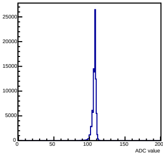
Pedestals mcm 0 ch 40 chamber-fec0
