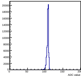
Pedestals mcm 0 ch 26 chamber-fec0
