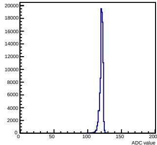
Pedestals mcm 0 ch 5 chamber-fec0
