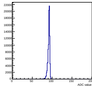
Pedestals mcm 0 ch 122 chamber-fec0
