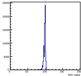
Pedestals mcm 0 ch 117 chamber-fec0
