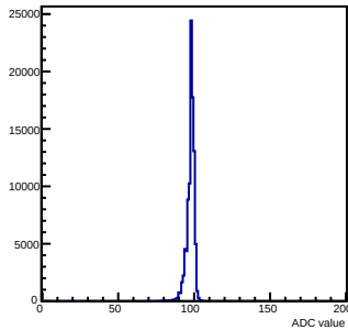
Pedestals mcm 0 ch 18 chamber-fec0
