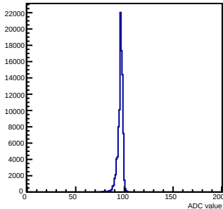
Pedestals mcm 0 ch 27 chamber-fec0
