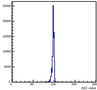
Pedestals mcm 0 ch 111 chamber-fec0
