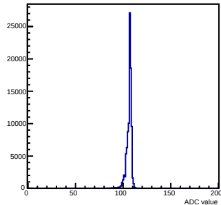
Pedestals mcm 0 ch 54 chamber-fec0
