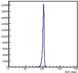
Pedestals mcm 0 ch 28 chamber-fec0
