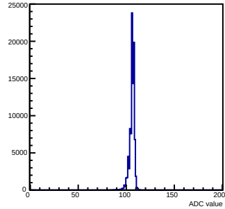
Pedestals mcm 0 ch 67 chamber-fec0
