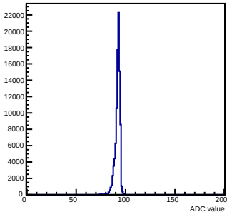
Pedestals mcm 0 ch 21 chamber-fec0
