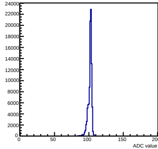
Pedestals mcm 0 ch 78 chamber-fec0
