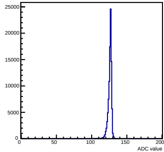
Pedestals mcm 0 ch 1 chamber-fec0
