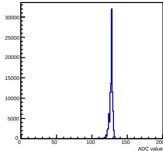
Pedestals mcm 0 ch 7 chamber-fec0
