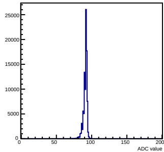
Pedestals mcm 0 ch 37 chamber-fec0
