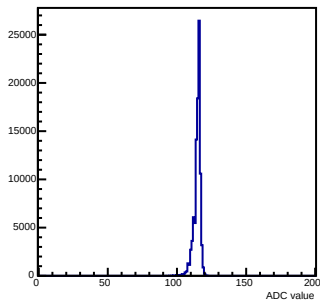
Pedestals mcm 0 ch 116 chamber-fec0
