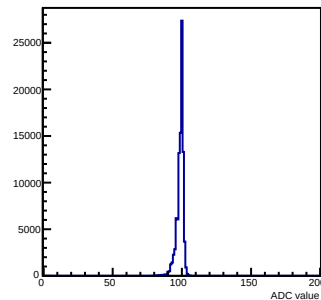
Pedestals mcm 0 ch 118 chamber-fec0
