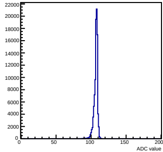
Pedestals mcm 0 ch 105 chamber-fec0
