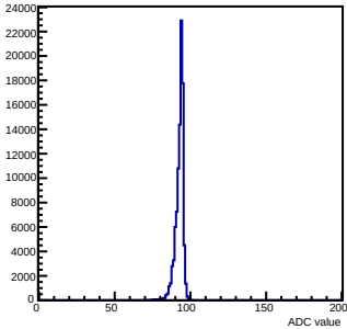
Pedestals mcm 0 ch 36 chamber-fec0
