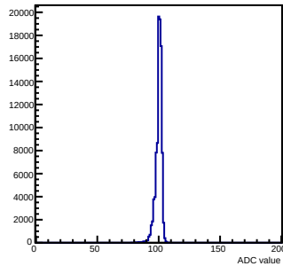
Pedestals mcm 0 ch 82 chamber-fec0
