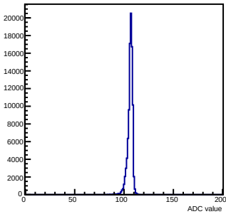
Pedestals mcm 0 ch 64 chamber-fec0
