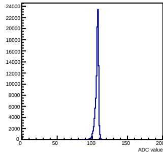
Pedestals mcm 0 ch 91 chamber-fec0
