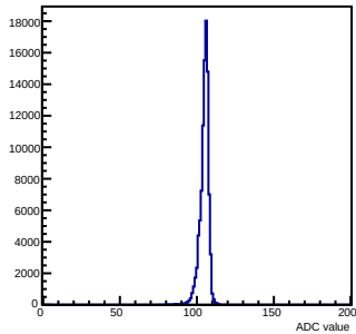
Pedestals mcm 0 ch 48 chamber-fec0
