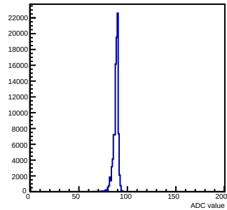
Pedestals mcm 0 ch 75 chamber-fec0
