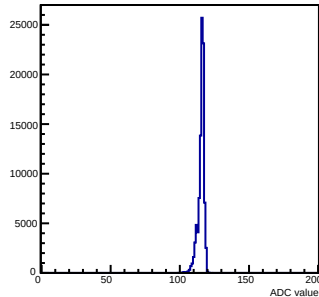
Pedestals mcm 0 ch 15 chamber-fec0
