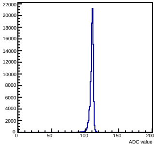
Pedestals mcm 0 ch 29 chamber-fec0
