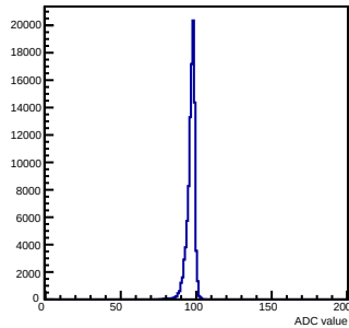
Pedestals mcm 0 ch 73 chamber-fec0
