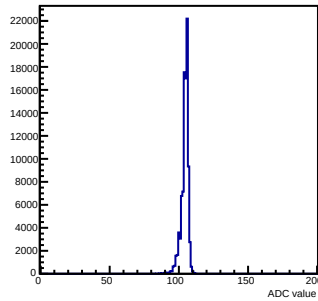
Pedestals mcm 0 ch 98 chamber-fec0
