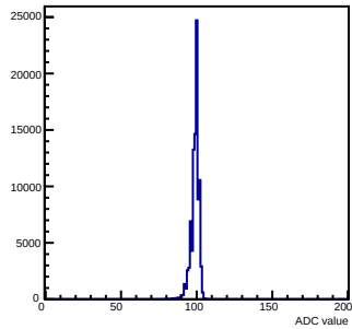
Pedestals mcm 0 ch 97 chamber-fec0
