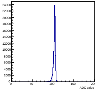
Pedestals mcm 0 ch 22 chamber-fec0
