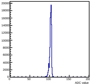
Pedestals mcm 0 ch 24 chamber-fec0
