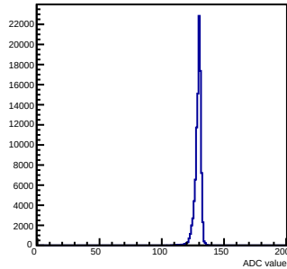
Pedestals mcm 0 ch 3 chamber-fec0
