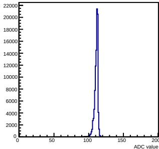
Pedestals mcm 0 ch 23 chamber-fec0
