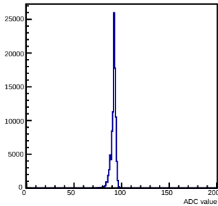
Pedestals mcm 0 ch 19 chamber-fec0
