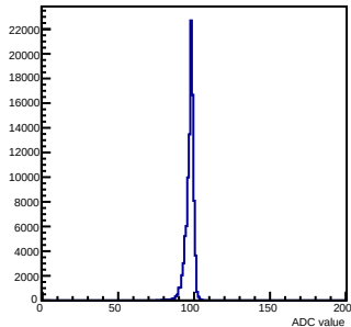
Pedestals mcm 0 ch 52 chamber-fec0
