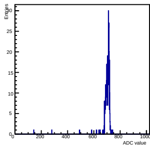
Max PH 0sup ch 0 chip 14 zerosuppreamp0gain0shaper0decay05
