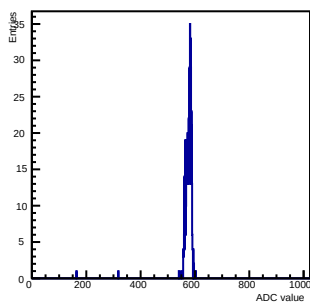
Max PH 0sup ch 5 chip 14 zerosuppreamp0gain0shaper0decay05
