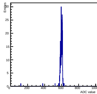
Max PH 0sup ch 10 chip 14 zerosuppreamp0gain0shaper0decay0
