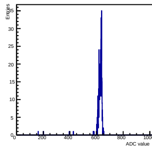
Max PH 0sup ch 2 chip 14 zerosuppreamp0gain0shaper0decay05
