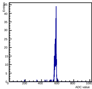
Max PH 0sup ch 8 chip 14 zerosuppreamp0gain0shaper0decay05
