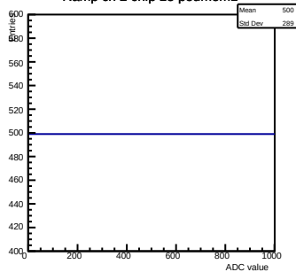
Ramp ch 2 chip 15 pedmem1
