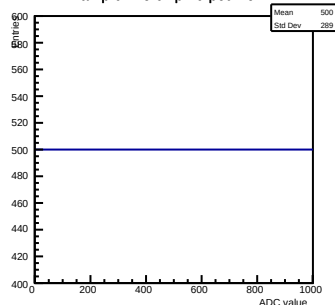
Ramp ch 15 chip 19 pedmem.
