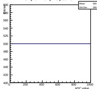
Ramp ch 7 chip 23 pedmem1
