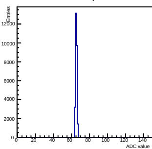
Pedestals ch 8 chip 29 nominal
