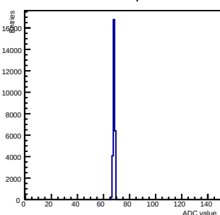
Pedestals ch 12 chip 29 nominal
