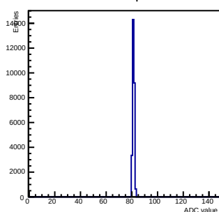
Pedestals ch 6 chip 29 nominal
