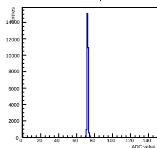
Pedestals ch 15 chip 29 nominal
