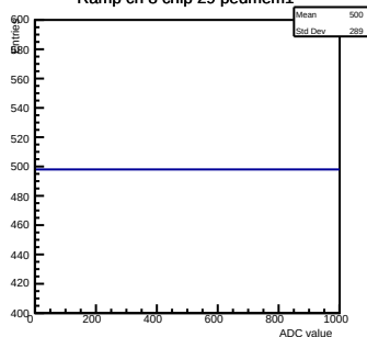
Ramp ch 8 chip 29 pedmem1
