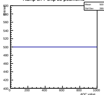
Ramp ch 7 chip 29 pedmem1
