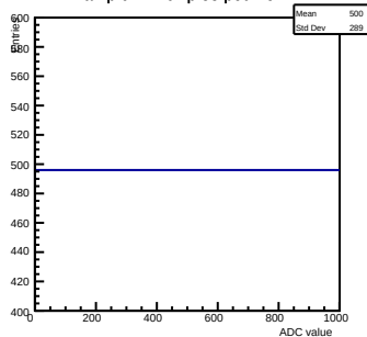
Ramp ch 12 chip 33 pedmem1
