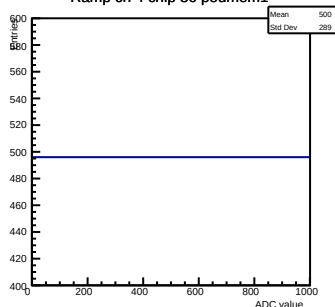
Ramp ch 4 chip 36 pedmem1
