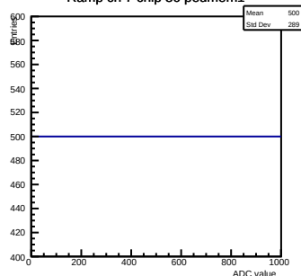
Ramp ch 7 chip 36 pedmem1
