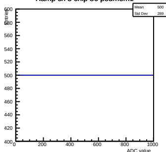
Ramp ch 5 chip 36 pedmem1
