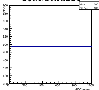
Ramp ch 14 chip 36 pedmem1
