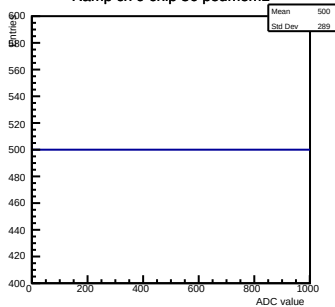
Ramp ch 9 chip 36 pedmem1
