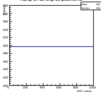
Ramp ch 12 chip 36 pedmem1
