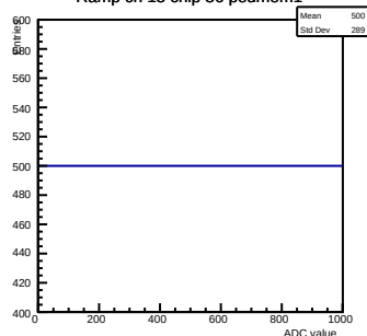
Ramp ch 15 chip 36 pedmem.
