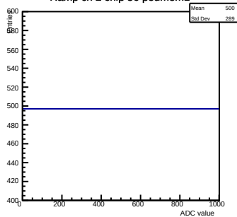
Ramp ch 2 chip 36 pedmem1
