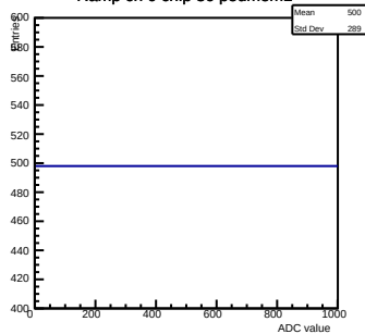
Ramp ch 0 chip 36 pedmem1
