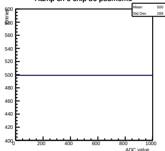
Ramp ch 6 chip 36 pedmem1
