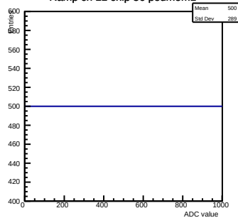
Ramp ch 11 chip 36 pedmem.
