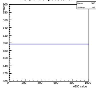
Ramp ch 8 chip 36 pedmem1
