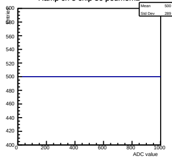
Ramp ch 3 chip 36 pedmem1
