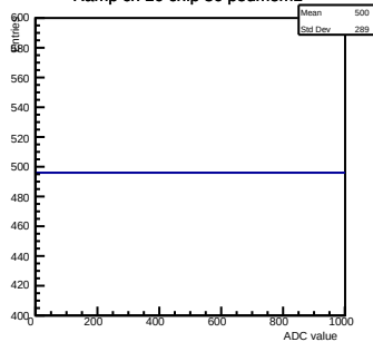
Ramp ch 10 chip 36 pedmem1
