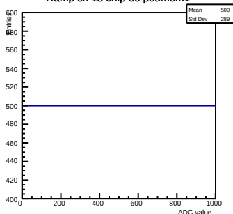
Ramp ch 13 chip 36 pedmem1
