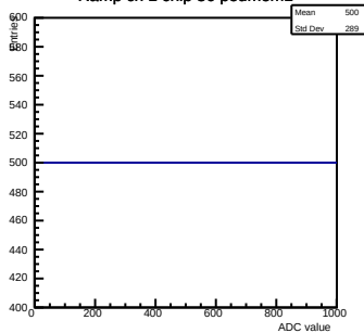
Ramp ch 1 chip 36 pedmem1
