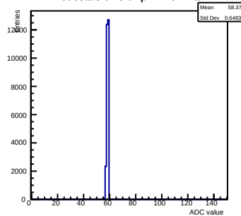
Pedestals ch 3 chip 42 nominal
