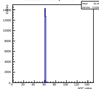
Pedestals ch 15 chip 42 nominal
