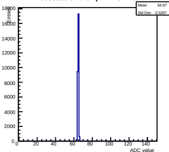
Pedestals ch 9 chip 42 nominal
