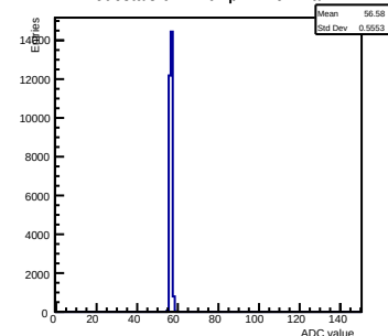
Pedestals ch 12 chip 42 nominal
