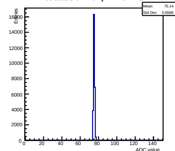
Pedestals ch 4 chip 42 nominal
