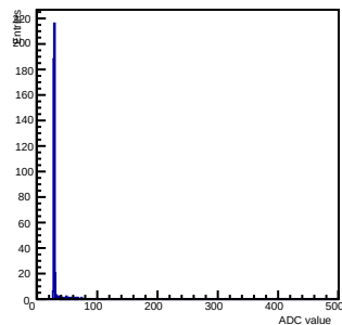
Width ch 14 chip 50 allsigpreamp1gain3shaper0decay05
