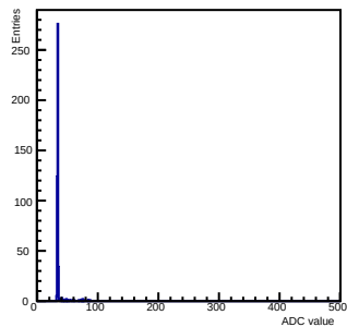
Width ch 9 chip 50 alsigpreamp1gain3shaper0decay05
