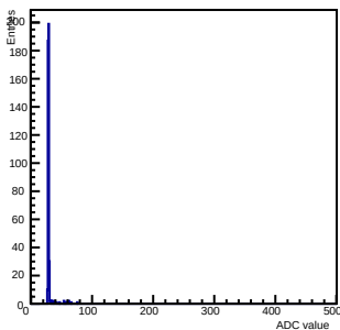
Width ch 12 chip 50 allsigpreamp1gain3shaper0decay0
