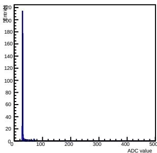
Width ch 4 chip 50 albsigpreamp1gain3shaper0decay05
