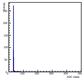
Width ch 6 chip 50 allsigpreamp1gain3shaper0decay05
