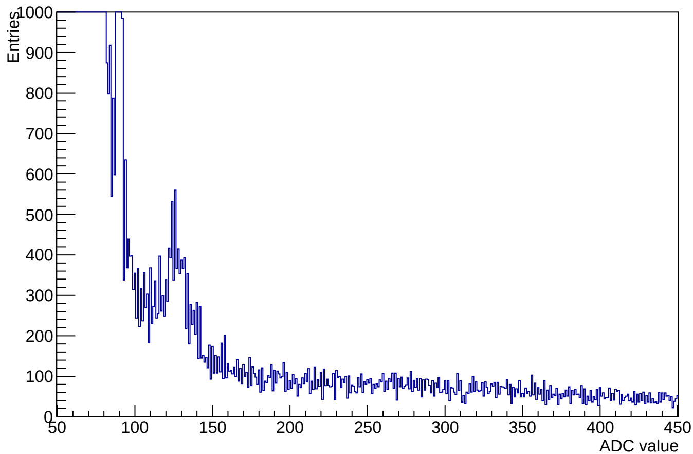
ADC samples for channel 0 clusters 8459 (used 7675)
