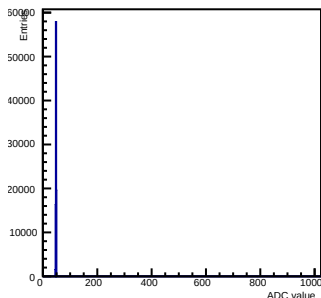
Pedestals ch 5 chip 55
