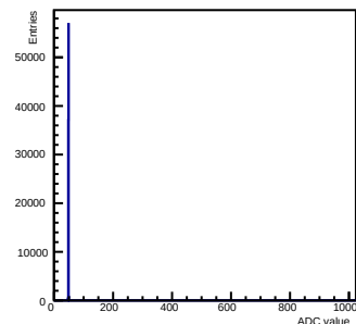
Pedestals ch 7 chip 55
