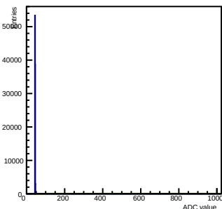
Pedestals ch 4 chip 55
