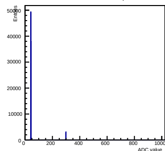
Pedestals ch 15 chip 55
