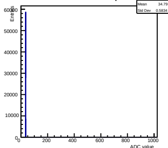
Pedestals ch 14 chip 55
