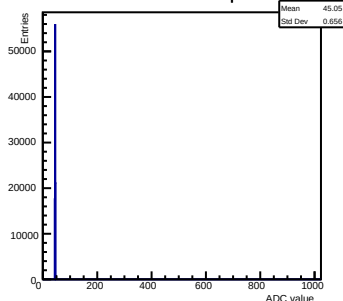
Pedestals ch 6 chip 55
