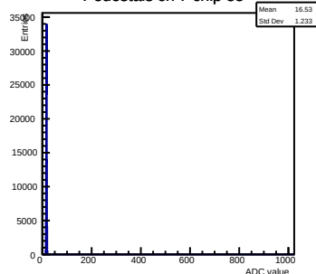
Pedestals ch 7 chip 55
