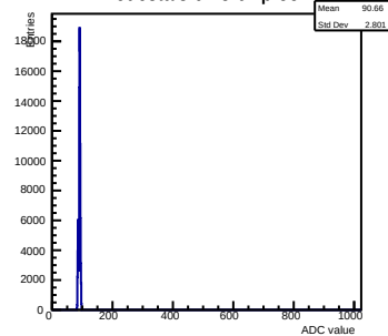
Pedestals ch 3 chip 55
