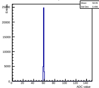
Pedestals ch 7 chip 6 nominal
