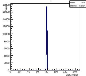
Pedestals ch 6 chip 6 nominal
