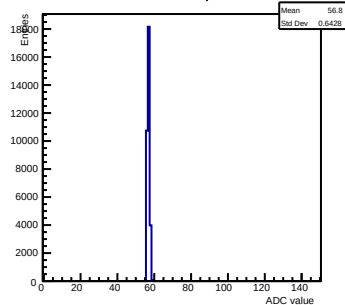
Pedestals ch 14 chip 6 nominal
