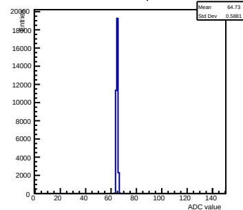
Pedestals ch 12 chip 6 nominal
