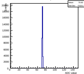
Pedestals ch 15 chip 6 nominal
