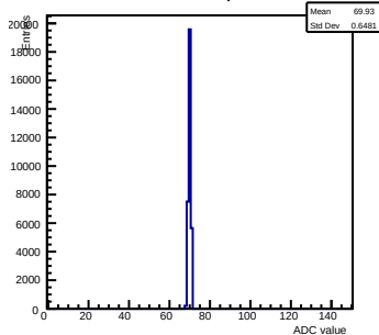
Pedestals ch 13 chip 6 nominal
