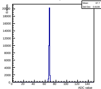
Pedestals ch 5 chip 6 nominal
