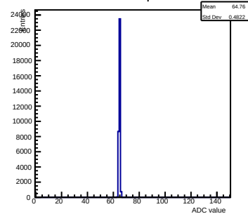
Pedestals ch 8 chip 6 nominal
