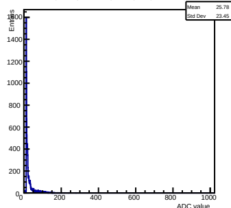
CI length 0sup ch 12 chip 6 shaper0-gain0-decay05
