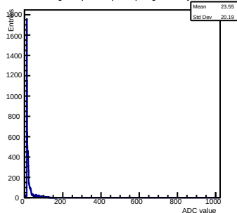
CI length 0sup ch 9 chip 6 shaper0-gain0-decay05
