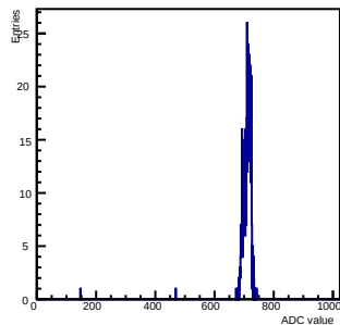
Max PH Oup ch 7 chip 63 zerosuppreamp0gain0shaper0decay05
