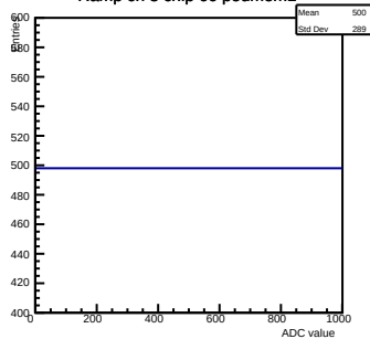
Ramp ch 8 chip 66 pedmem1
