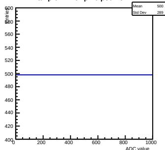
Ramp ch 12 chip 70 pedmem1
