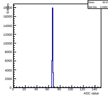
Pedestals ch 2 chip 9 nominal
