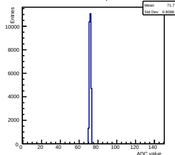
Pedestals ch 15 chip 9 nominal
