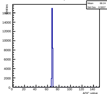
Pedestals ch 13 chip 9 nominal
