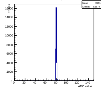
Pedestals ch 12 chip 9 nominal
