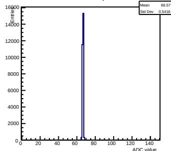
Pedestals ch 14 chip 9 nominal
