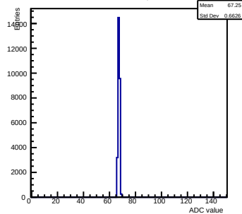
Pedestals ch 11 chip 9 nominal
