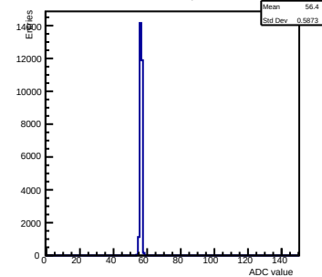
Pedestals ch 0 chip 9 nominal
