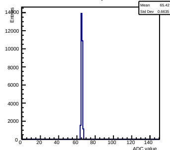
Pedestals ch 7 chip 9 nominal
