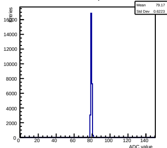
Pedestals ch 5 chip 9 nominal
