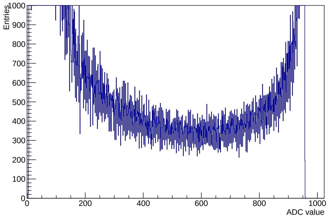
ADC samples for channel 6 clusters 61895 (used 61076)
