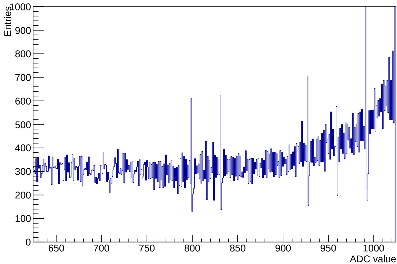
ADC samples for channel 3 clusters 218321 (used 61108)
