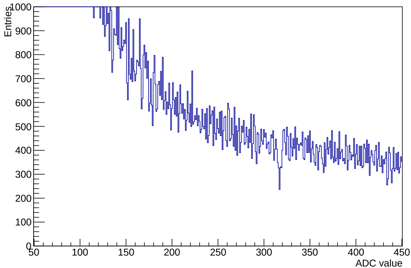
ADC samples for channel 1 clusters 61837 (used 61101)
