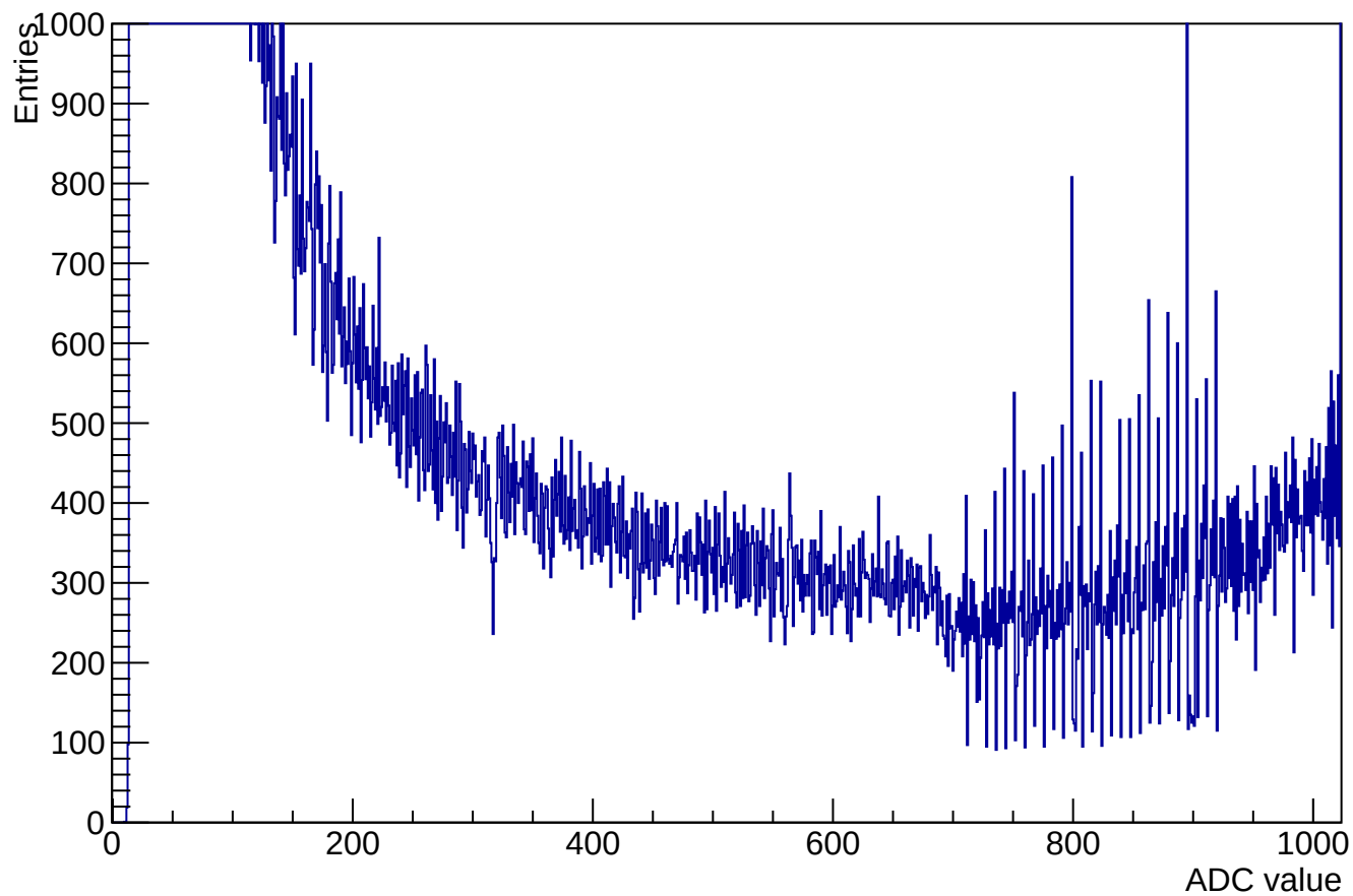
ADC samples for channel 1 clusters 61837 (used 61101)
