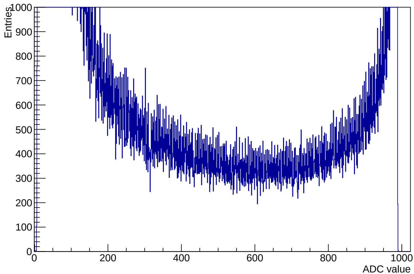
ADC samples for channel 13 clusters 62045 (used 61061)
