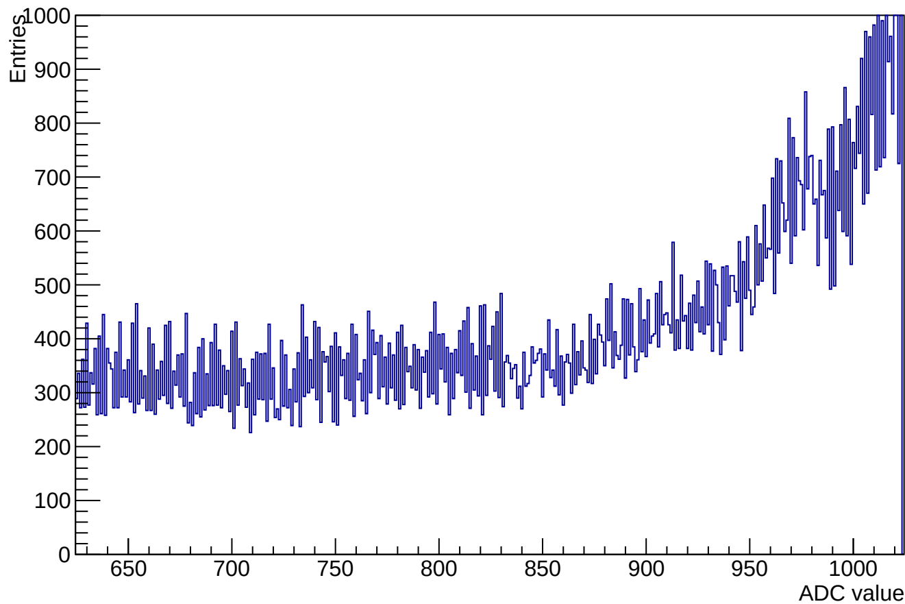
ADC samples for channel 14 clusters 456119 (used 60995)
