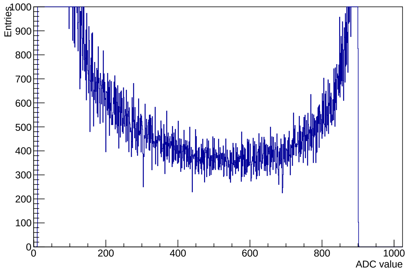
ADC samples for channel 9 clusters 61708 (used 61045)
