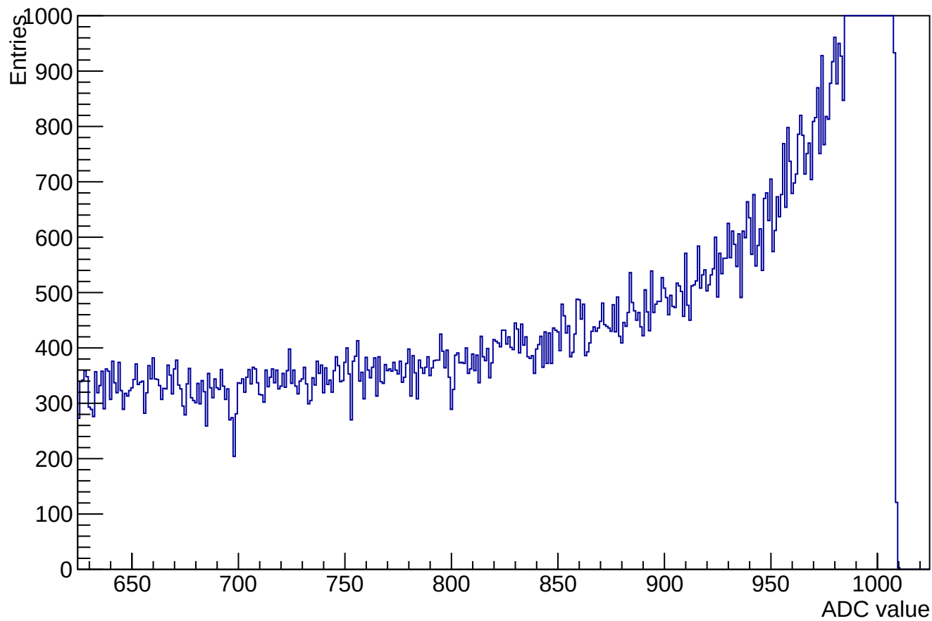
ADC samples for channel 4 clusters 434000 (used 61096)
