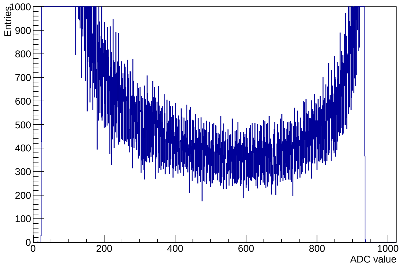
ADC samples for channel 8 clusters 144147 (used 61082)
