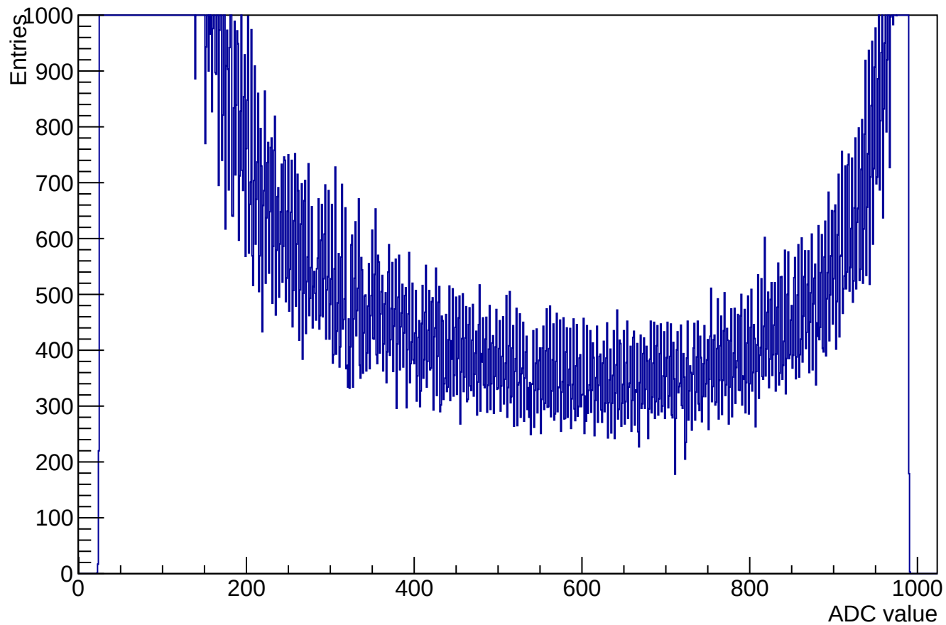
ADC samples for channel 12 clusters 174476 (used 61068)
