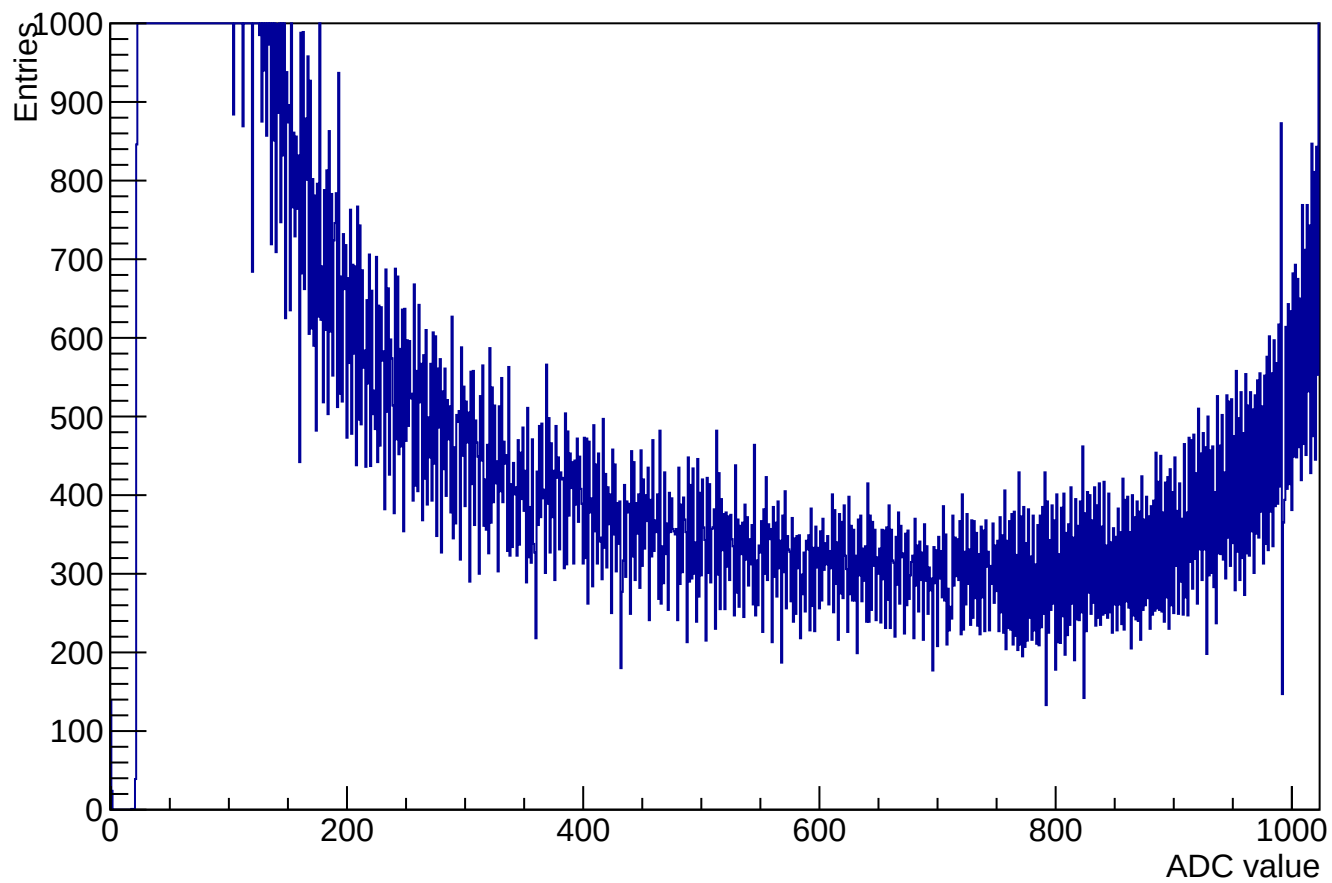
ADC samples for channel 15 clusters 61812 (used 60936)
