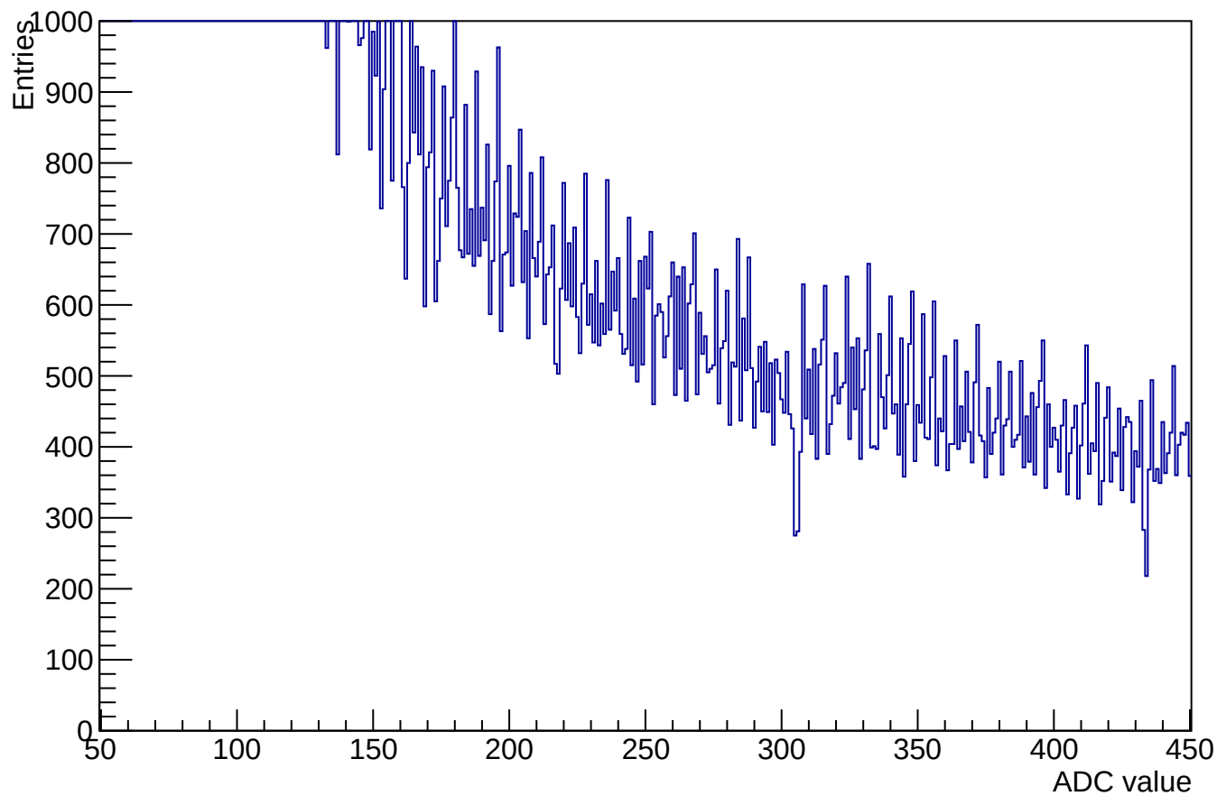
ADC samples for channel 7 clusters 62755 (used 61088)
