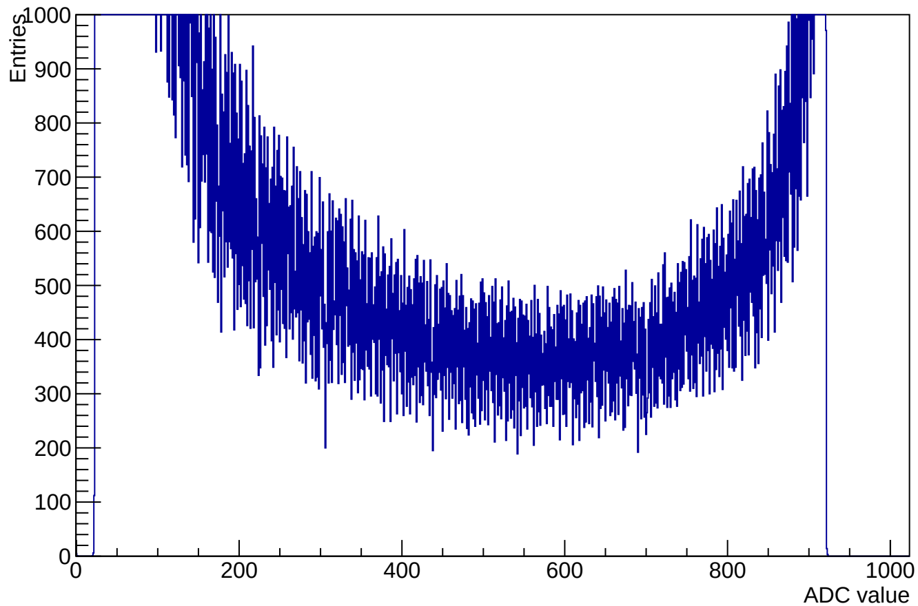
ADC samples for channel 11 clusters 62488 (used 61054)
