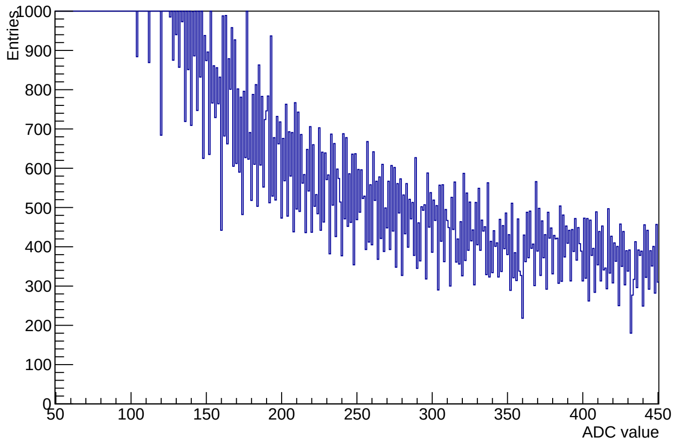
ADC samples for channel 15 clusters 61812 (used 60936)
