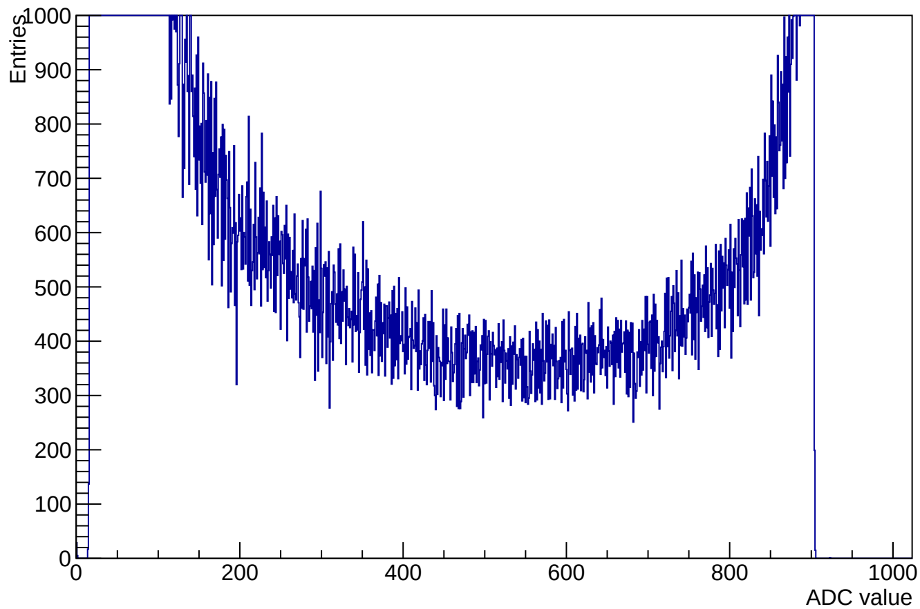
ADC samples for channel 10 clusters 61731 (used 61043)
