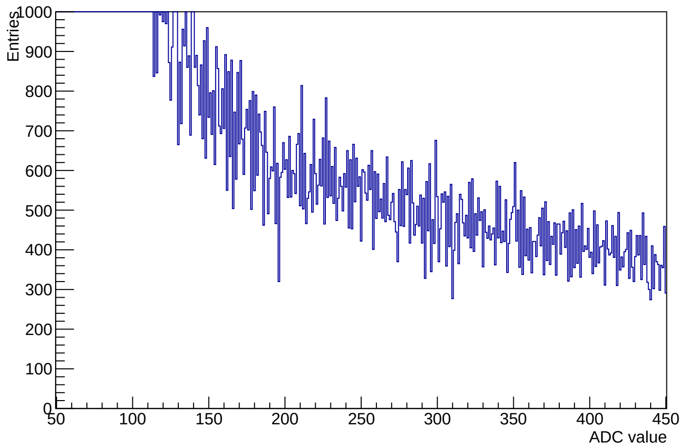
ADC samples for channel 10 clusters 61731 (used 61043)
