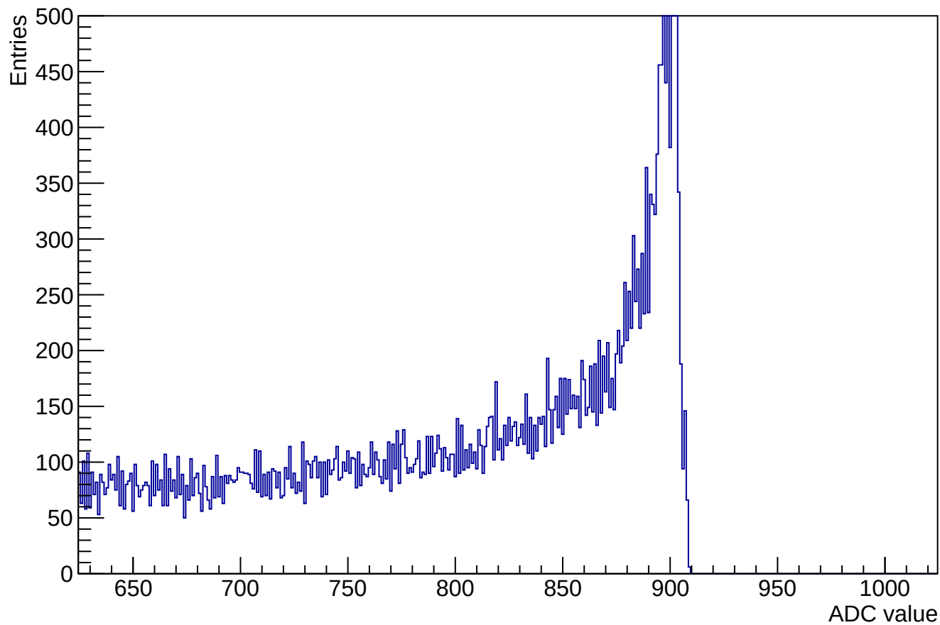
ADC samples for channel 10 events 56318 (used 0)
