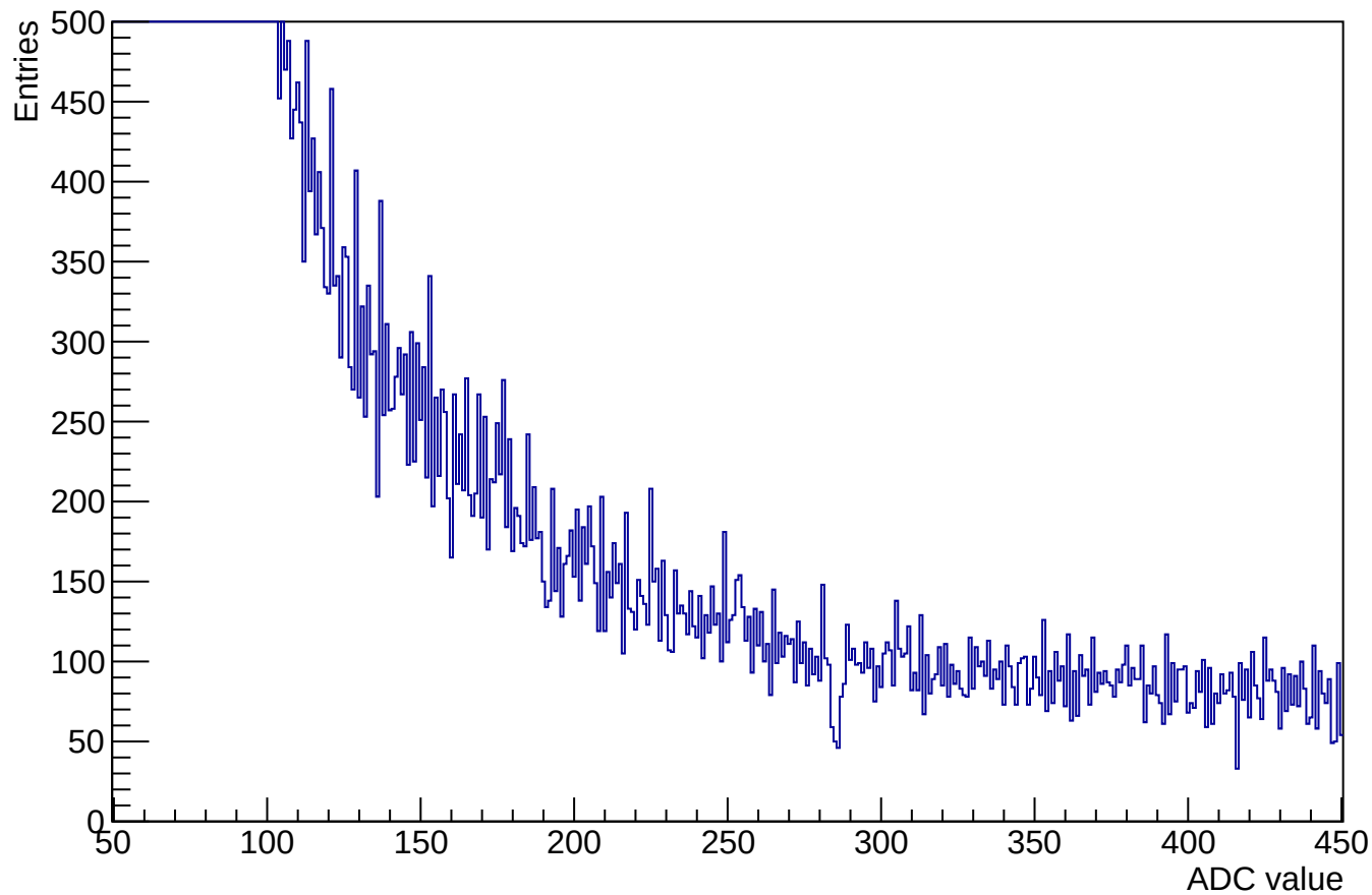
ADC samples for channel 0 events 56040 (used 0)
