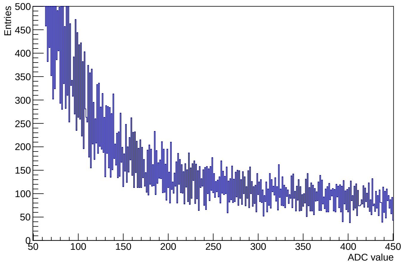
ADC samples for channel 11 events 56318 (used 0)
