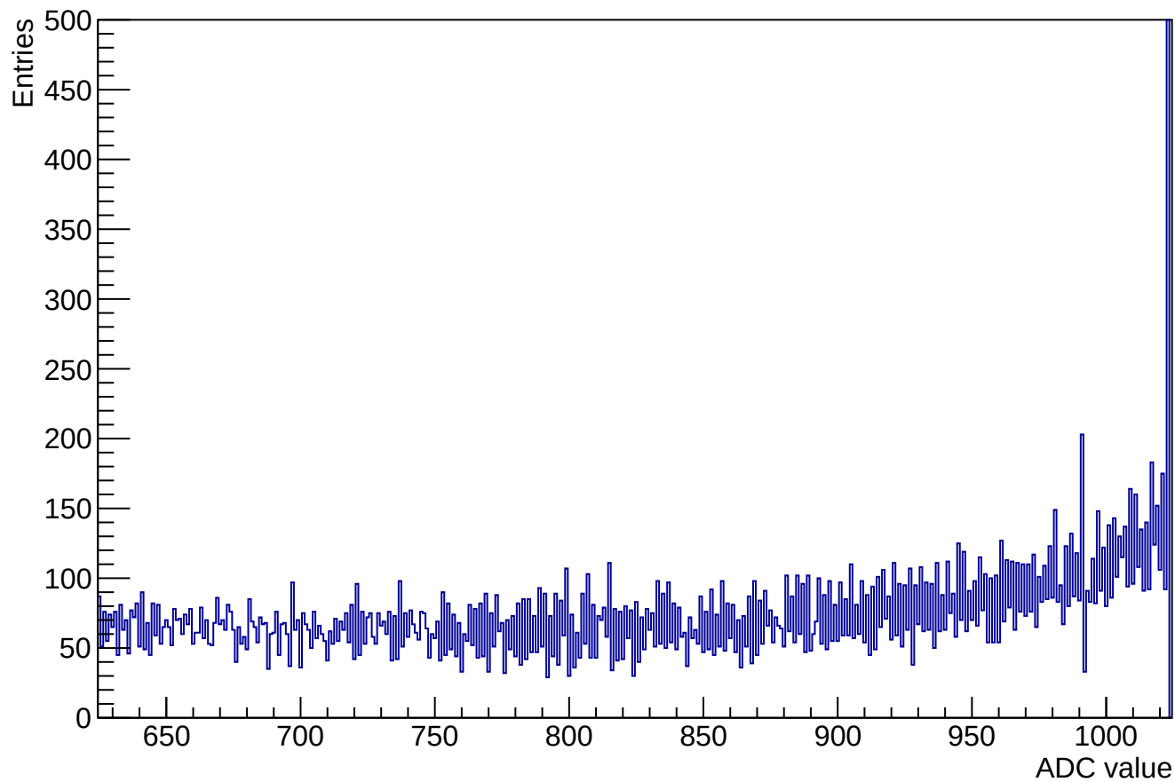
ADC samples for channel 15 events 56318 (used 0)
