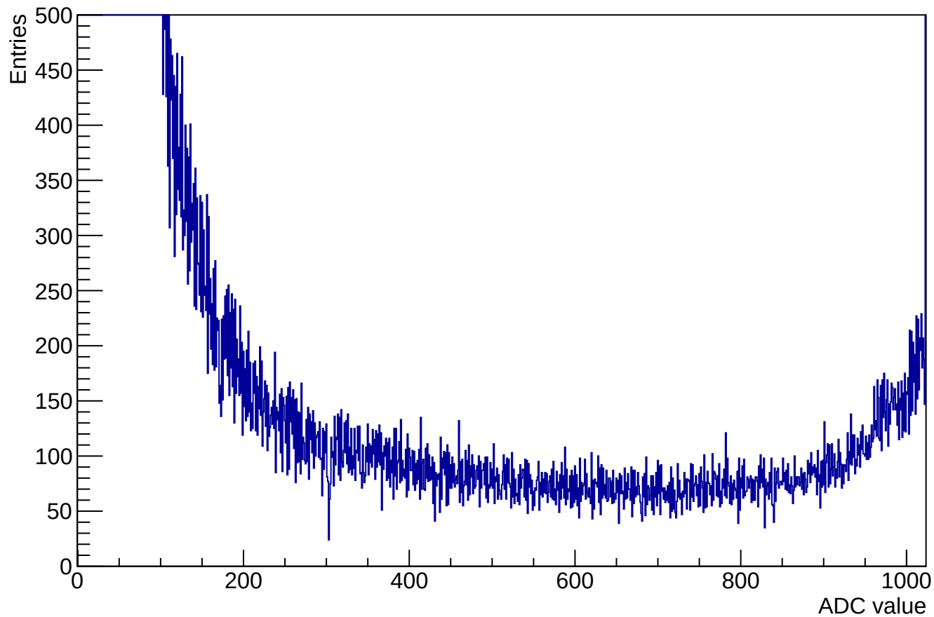
ADC samples for channel 14 events 56318 (used 0)
