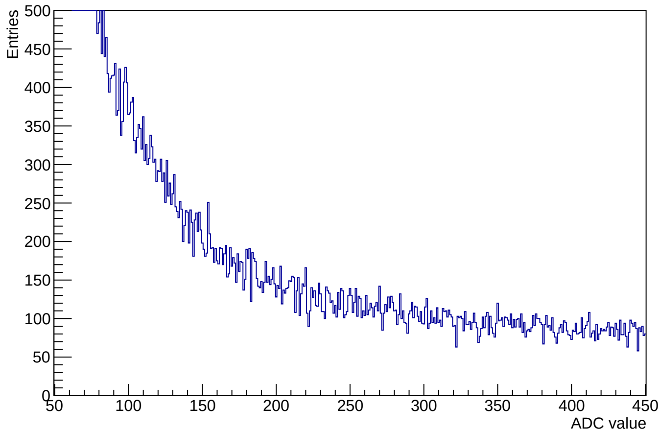
ADC samples for channel 4 events 56318 (used 0)
