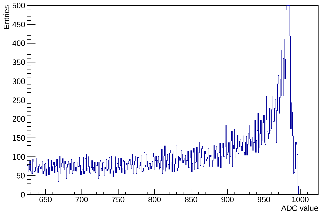
ADC samples for channel 12 events 56318 (used 0)
